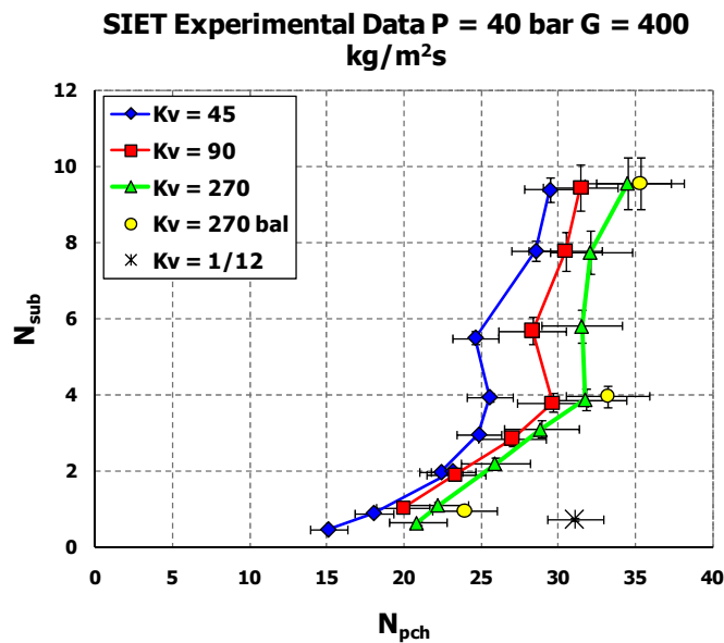
Figure 25 - Effect of inlet throttling on instability threshold at system pressure p = 40 bar and mass flux G = 400 \text{kg/m}^2\text{s} .
