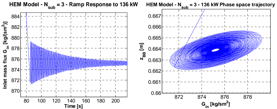
Figure 28 - Inlet mass flux oscillation curves and corresponding trajectories in the phase space for a stable state.
