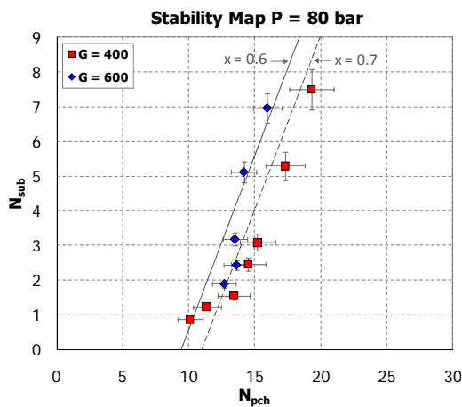
Figure 14 - Stability map obtained at system pressure p = 80 bar and different mass fluxes ( G = 600 kg/m 2 s, 400 kg/m 2 s).
