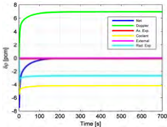
Figure 88. Reactivity contributors variation due to an enhancement by 5 K of core inlet temperature (MOX BoC).
