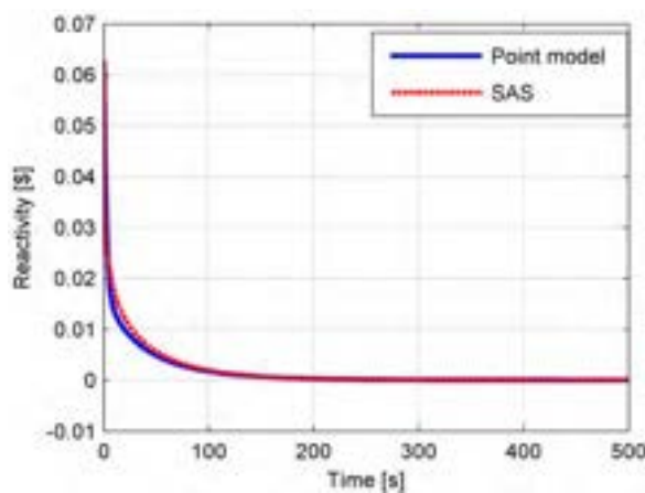
Figure 20. Reactivity function following a 20 pcm reactivity insertion for MOX BoC.
