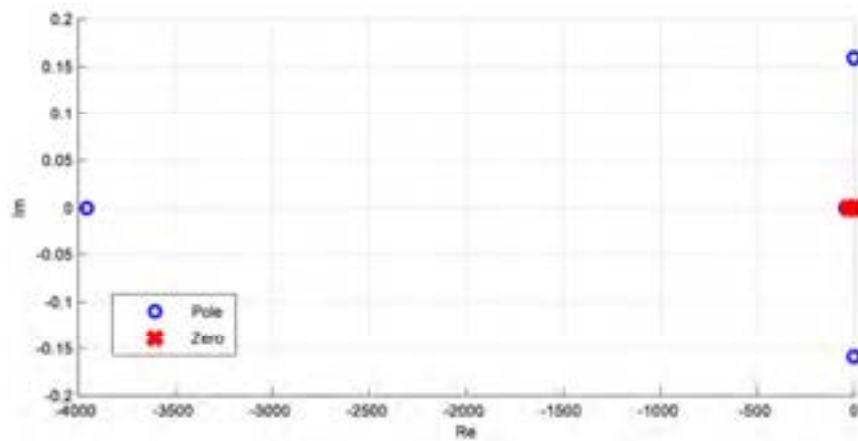
Figure 76. Pole-zero map of the TF between power (output) and coolant inlet temperature (input).
