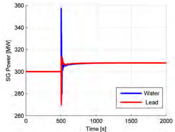
Figure 211. SG power variation following a 20 pcm reactivity insertion.
