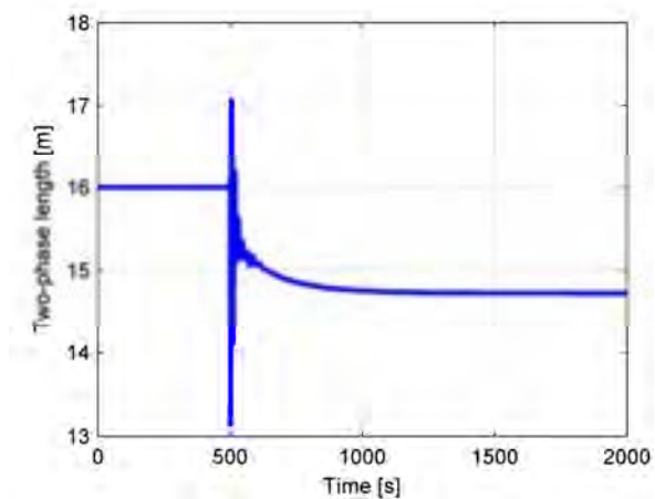
Figure 207. Two-phase length variation in the SG following a 20 pcm reactivity insertion.
