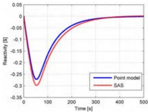
Figure 38. Reactivity function following a mass flow rate reduction for MET BoC.
