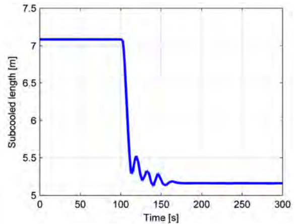
Figure 119. Sub-cooled length following an enhancement by 10 K of feedwater inlet temperature.
