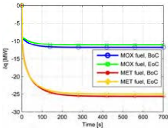
Figure 90. Core power variation due to an enhancement by 5 K of core inlet temperature.
