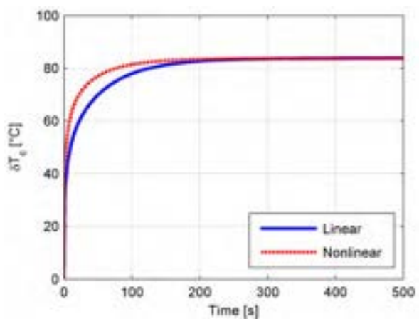
Figure 68. Cladding temperature variation following a 170 pcm reactivity insertion (met, EoC).
