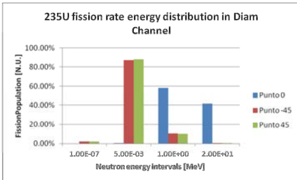
Figure 27 a) Comparison of mesh tally and detector tally responses for fission rate of ^{235}\text{U} along the axis of the diametrical channel b) Four energy bins representation of the fission rate spectrum in three selected point detectors along the diametrical channel.
