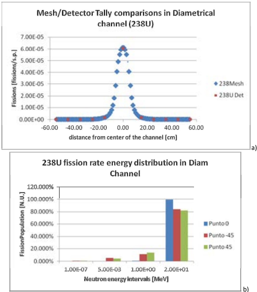
Figure 28 a) Comparison of mesh tally and detector tally responses for fission rate 238 U along the axis of the diametrical channel. b) Four energy bins representation of the fission rate spectrum in three selected point detectors along the diametrical channel.
