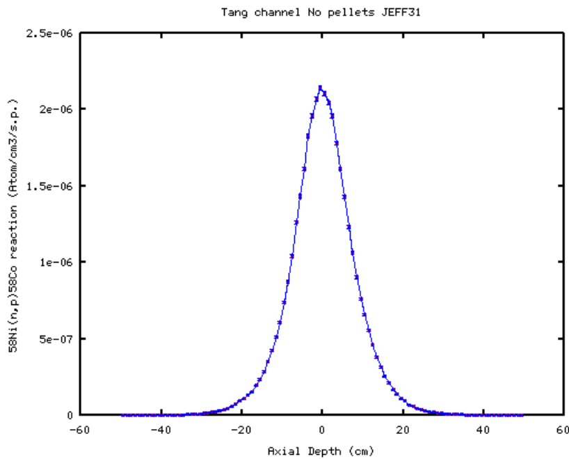
Figure 49 Monte Carlo estimates of ^{58}\text{Ni}(n,p)^{58}\text{Co} reaction rate on mesh tally in the tangential channel of TAPIRO (JEFF31 data set, no pellet, Mesh voxel 1 \times 1 \times 1 \text{ cm}^3 ).
