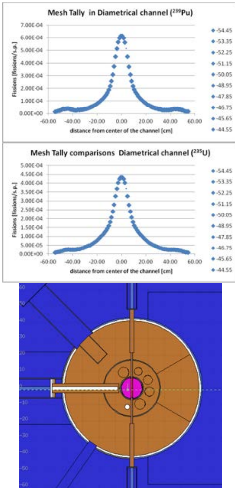
Figure 22 Fission rate on mesh tally for 239 Pu (a), 235 U (b) in the diametrical channel of TAPIRO (JEFF31 data set, no pellet, Mesh voxel 1x1x1 cm 3 ).
