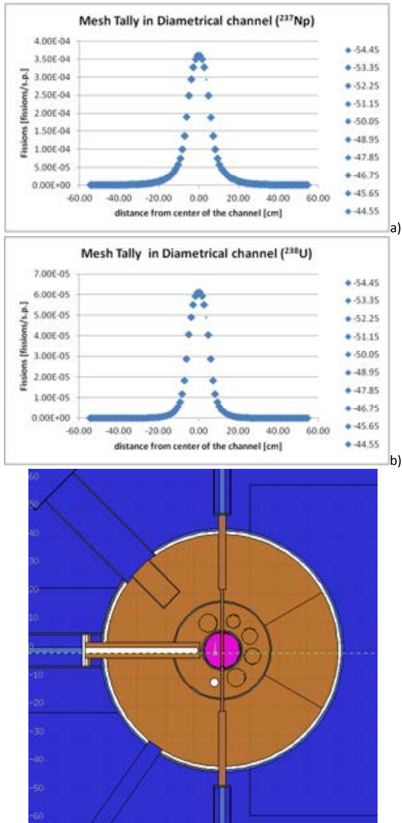
Figure 21: Fission rate on mesh tally for ^{237}\text{Np} (a), ^{238}\text{U} (b) in the diametrical channel of TAPIRO (JEFF31 data set, no pellet, Mesh voxel 1 \times 1 \times 1 \text{ cm}^3 ).
