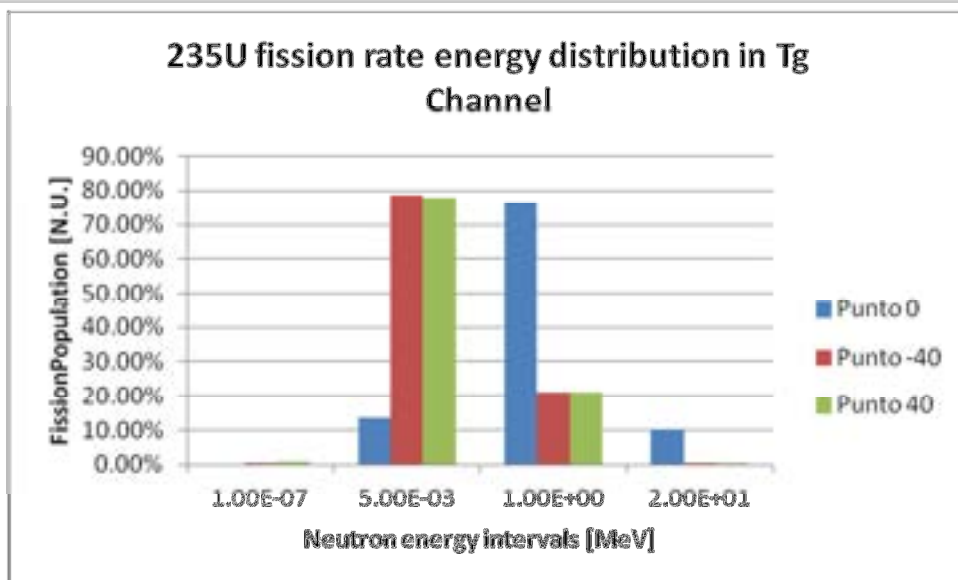
Figure 35 a) Comparison of mesh tally and detector tally responses for fission rate of ^{235}\text{U} along the axis of the Tangential channel. b) Four energy bins representation of the fission rate spectrum in three selected point detectors along the tangential channel.
