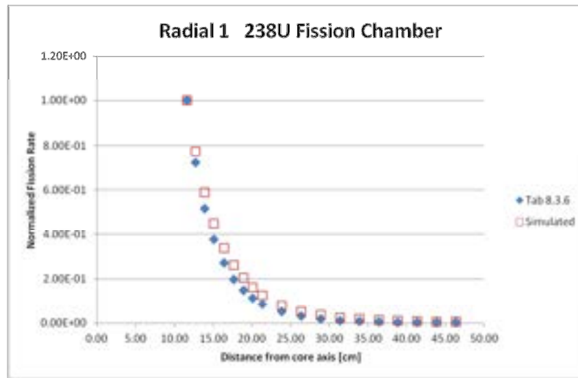
Figure 68 : Comparison of experimental vs. simulated responses 238 U fission chambers along Radial 1 channel.
