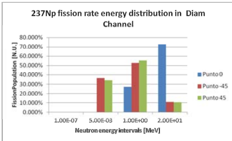
Figure 30 a) Comparison of mesh tally and detector tally responses for fission rate of 237 Np along the axis of the diametrical channel. b) Four energy bins representation of the fission rate spectrum in three selected point detectors along the diametrical channel.
