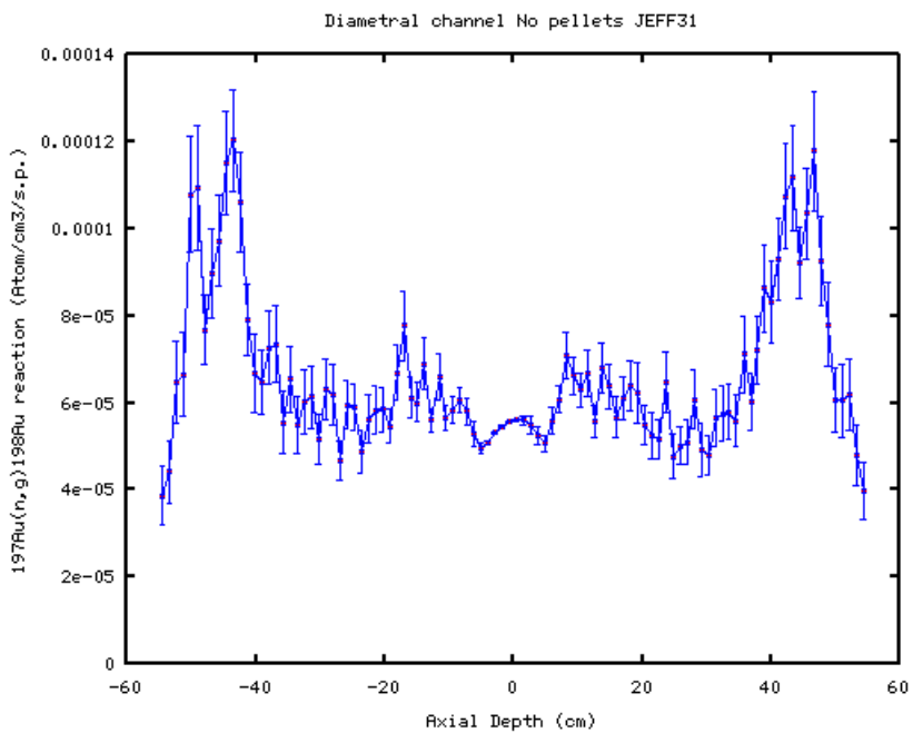
Figure 44 Monte Carlo estimates of ^{197}\text{Au}(n,\gamma)^{198}\text{Au} reaction rate on mesh tally for in the diametral channel of TAPIRO (JEFF31 data set, no pellet, Mesh voxel 1 \times 1 \times 1 \text{ cm}^3 ).
