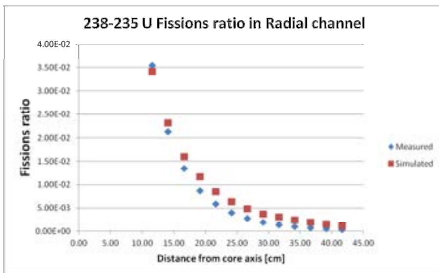
Figure 71 Comparison of the measured and estimated 238 U/ 235 U fissions ratio in the Radial channel 1.
