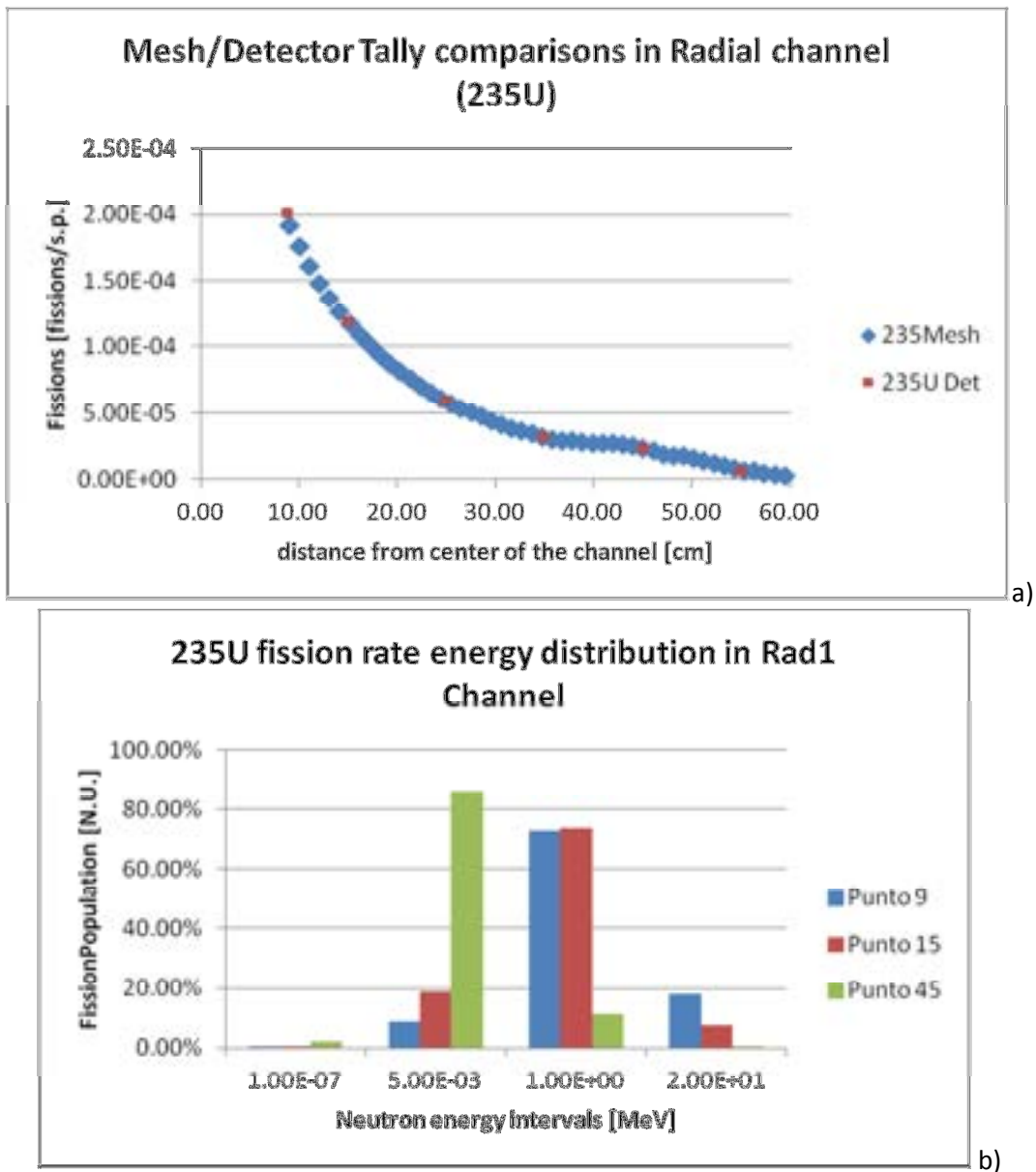
Figure 31 a) Comparison of mesh tally and detector tally responses for fission rate of 235 U along the axis of the Radial 1 channel. b) Four energy bins representation of the fission rate spectrum in three selected point detectors along the radial 1 channel.
