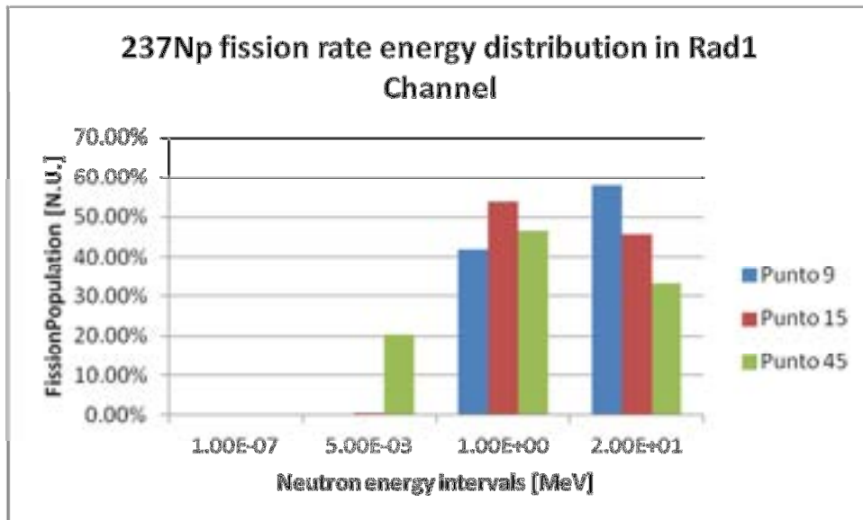
Figure 34 a) Comparison of mesh tally and detector tally responses for fission rate of ^{237}\text{Np} along the axis of the Radial 1 channel. b) Four energy bins representation of the fission rate spectrum in three selected point detectors along the radial 1 channel.
