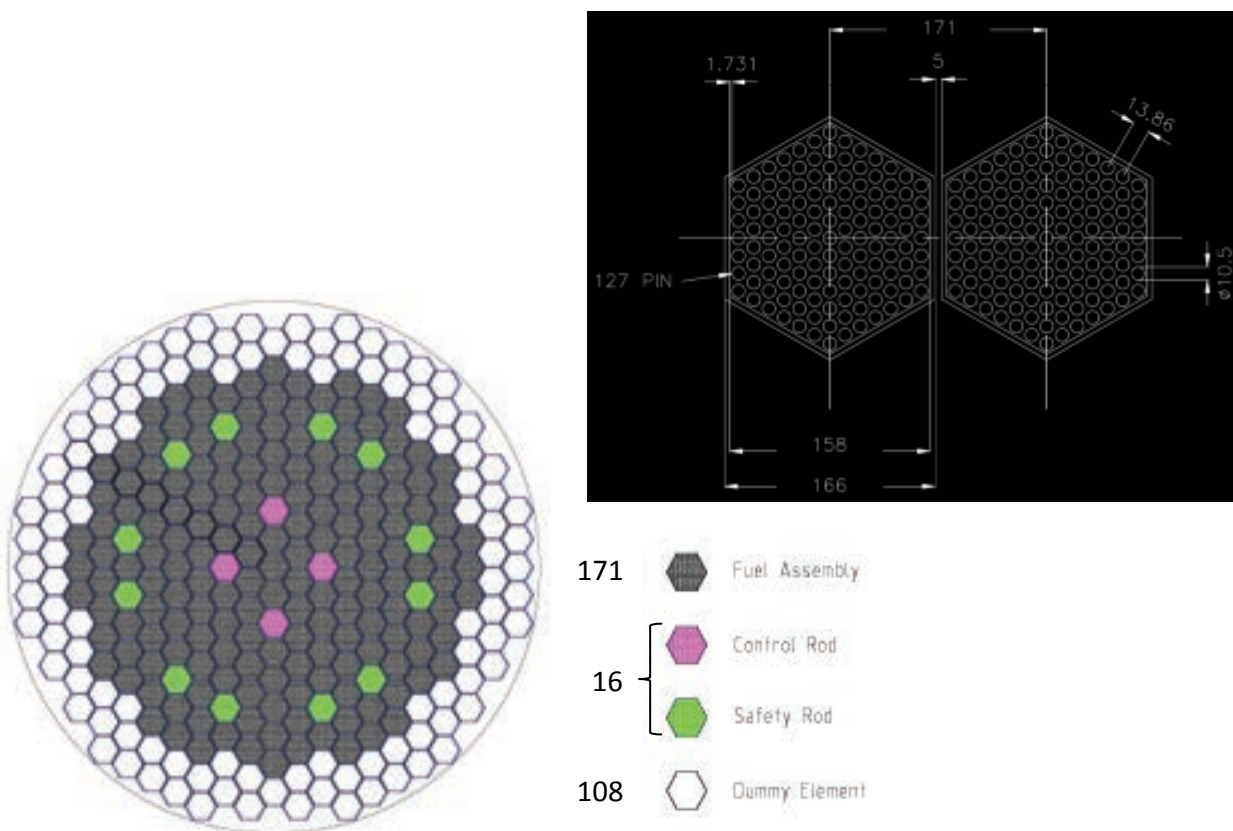
Fig. 1 – ALFRED Core
