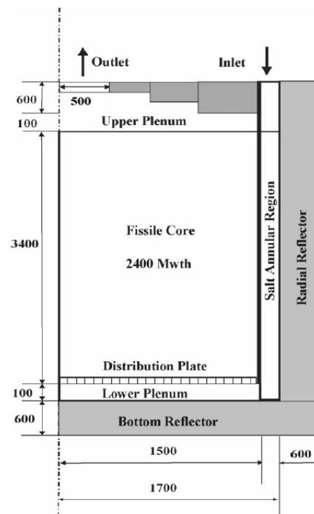
Figure 2.11: MOSART geometric model for SIMMER-III analysis.
