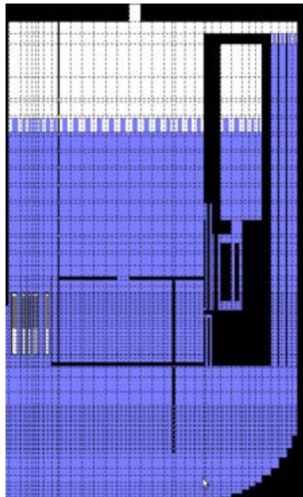
Figure 3.1: Overview of the MYRRHA FASTEF reactor and the SIMMER-III model.
