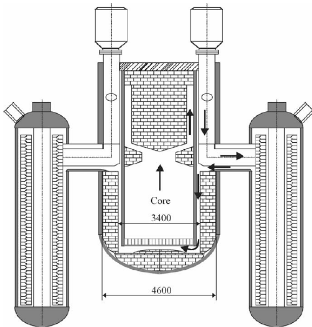
Figure 2.10: 2400 MW th MOSART preliminary design configuration.
