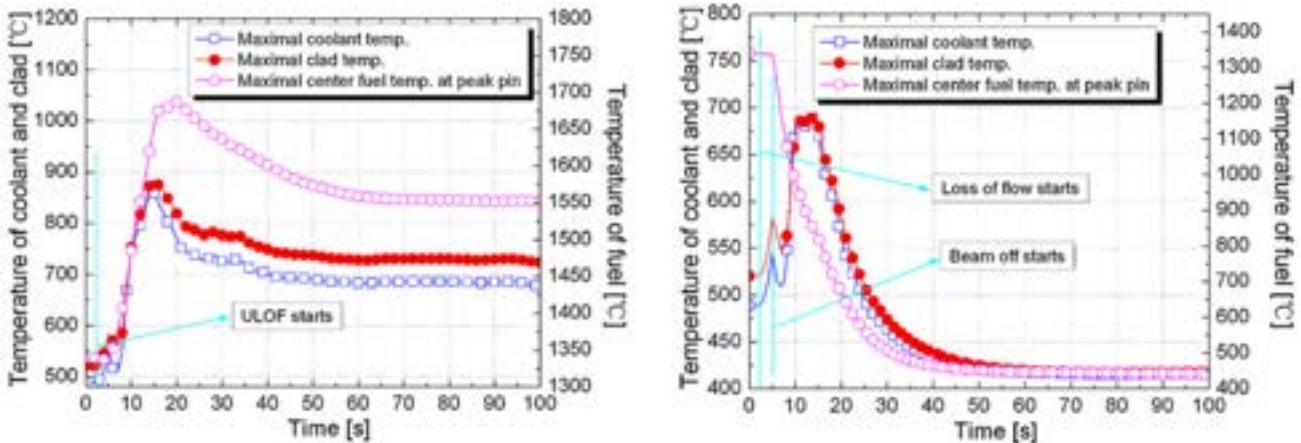
Figure 2.4: Temperature transients in ULOF and PLOF cases.
