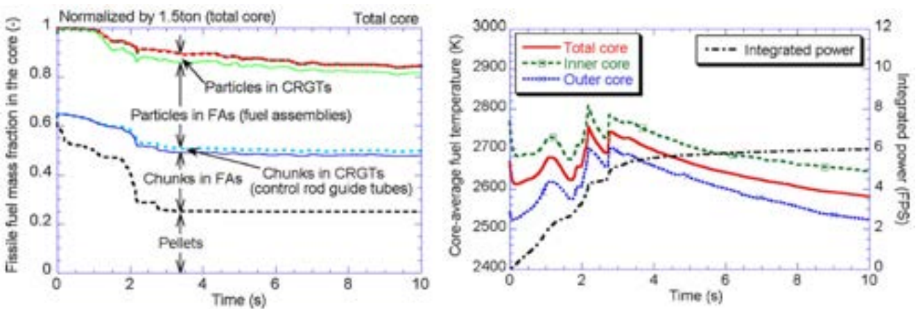
Figure 2.8: Fuel components and average fuel temperature in the core.
