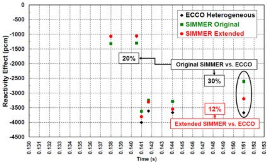
Figure 2.16: Reactivity effect in degraded models (comparison with SIMMER-III and ECCO).
