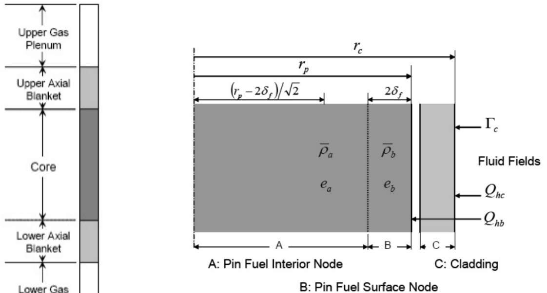
Figure 1.4: Radial fuel pin cross section in SIMMER-III.
