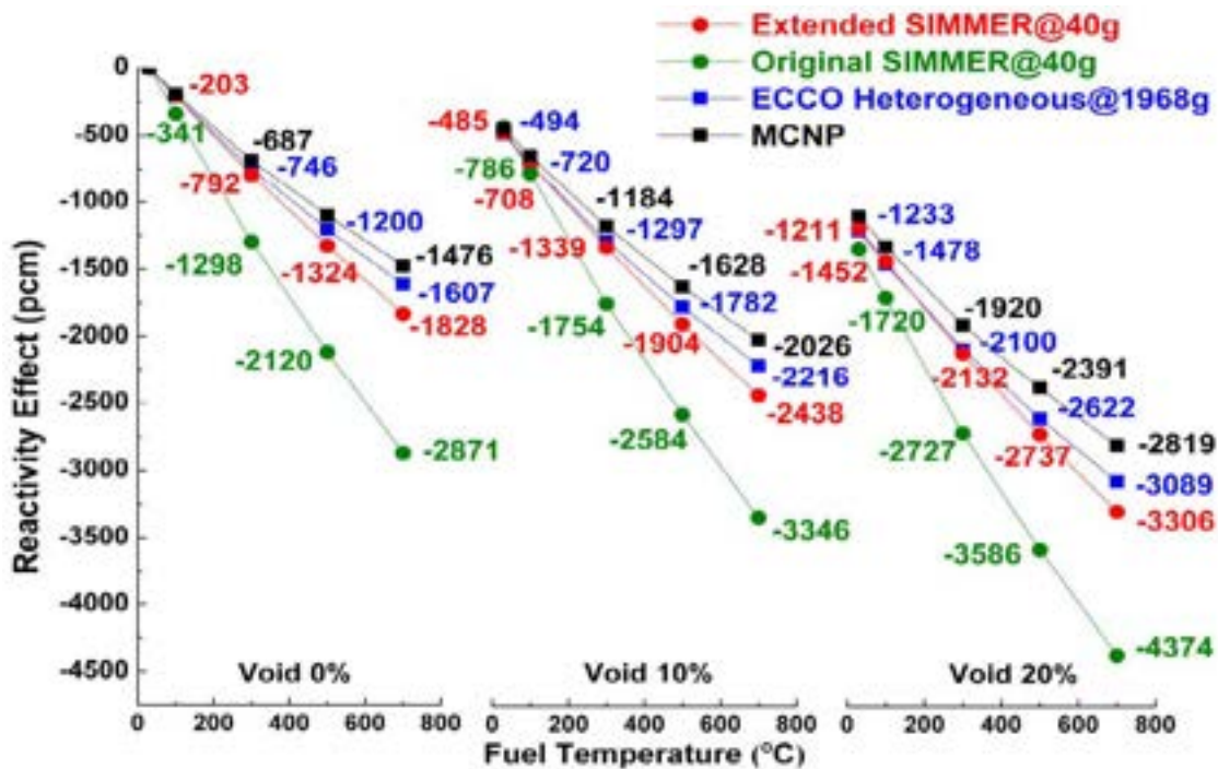
Figure 2.14: PWR fuel subassembly results with different codes.
