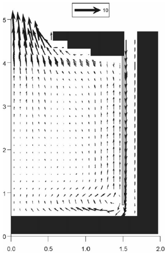
Figure 2.12: Velocity vector distribution.
