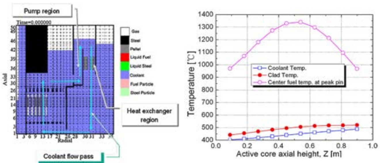
Figure 2.1: SIMMER-III model of EFIT and axial temperature profile in the first fuel ring.
