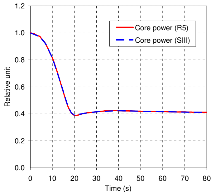
Figure 5.1: Core nuclear power evolution in the ULOF transient,
