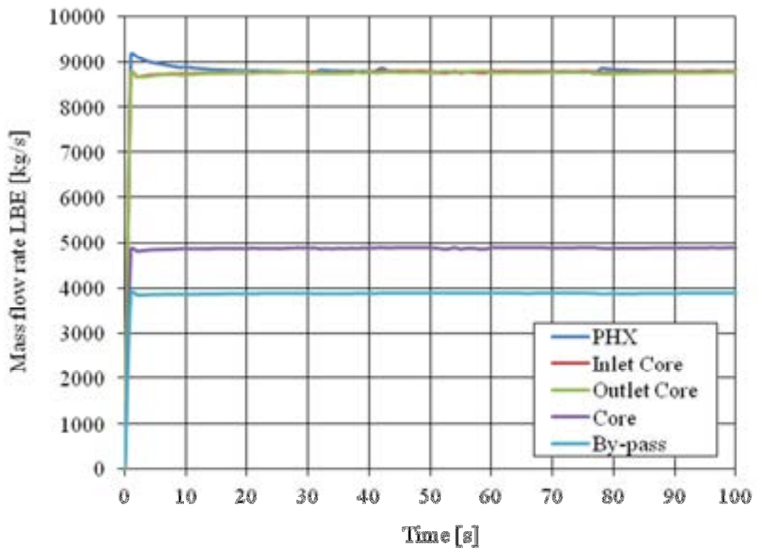
Figure 4.7: Trends mass flow rate in PHX and in the core
