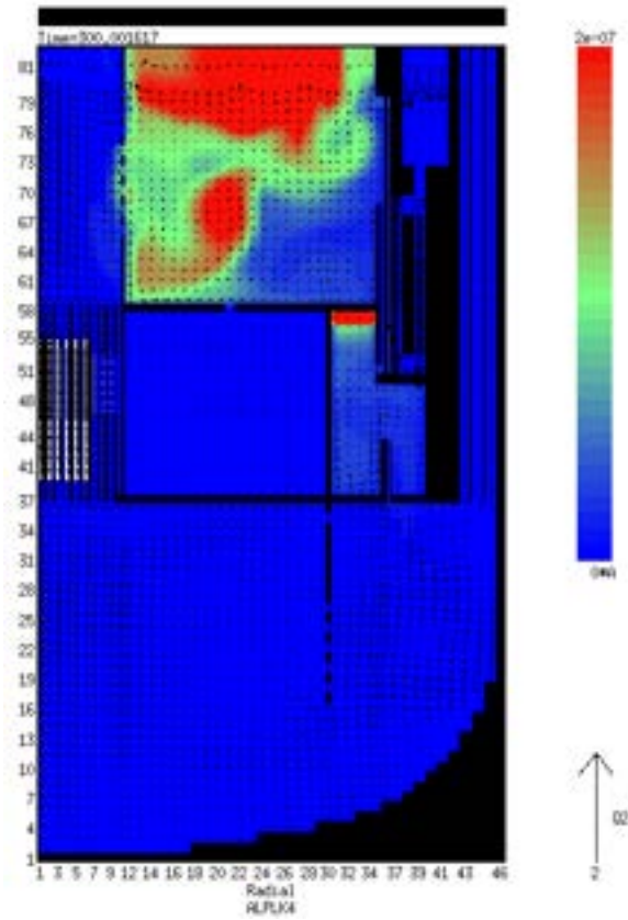
Figure 5.10: Fuel particle concentration in the primary circuit at t = 300 s (fuel porosity = 10%).
