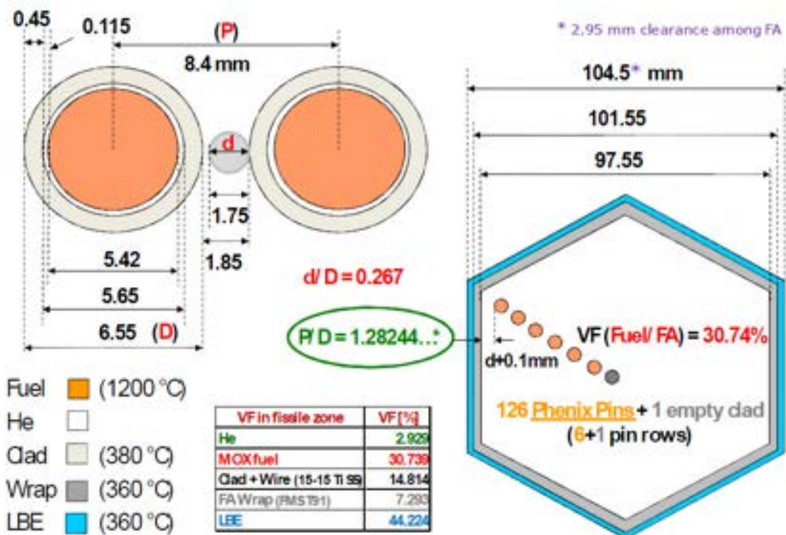
Figure 3.3: The reference FASTEF FA design.
