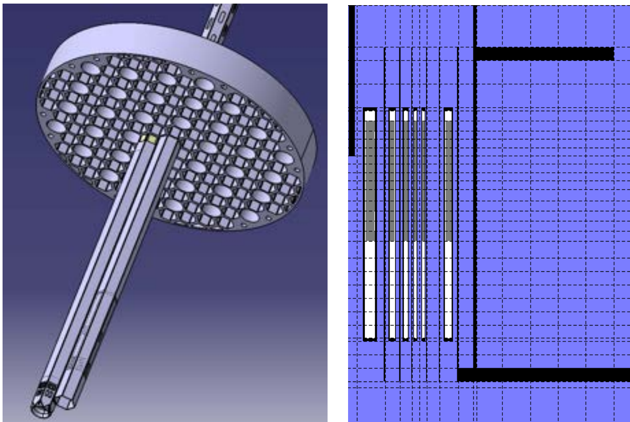
Figure 3.5: CAD and SIMMER-III model of the core.
