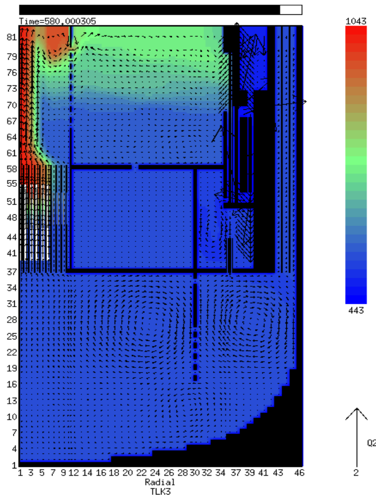
Figure 5.2: LBE temperature and velocity field at t = 80 s in the ULOF transient.
