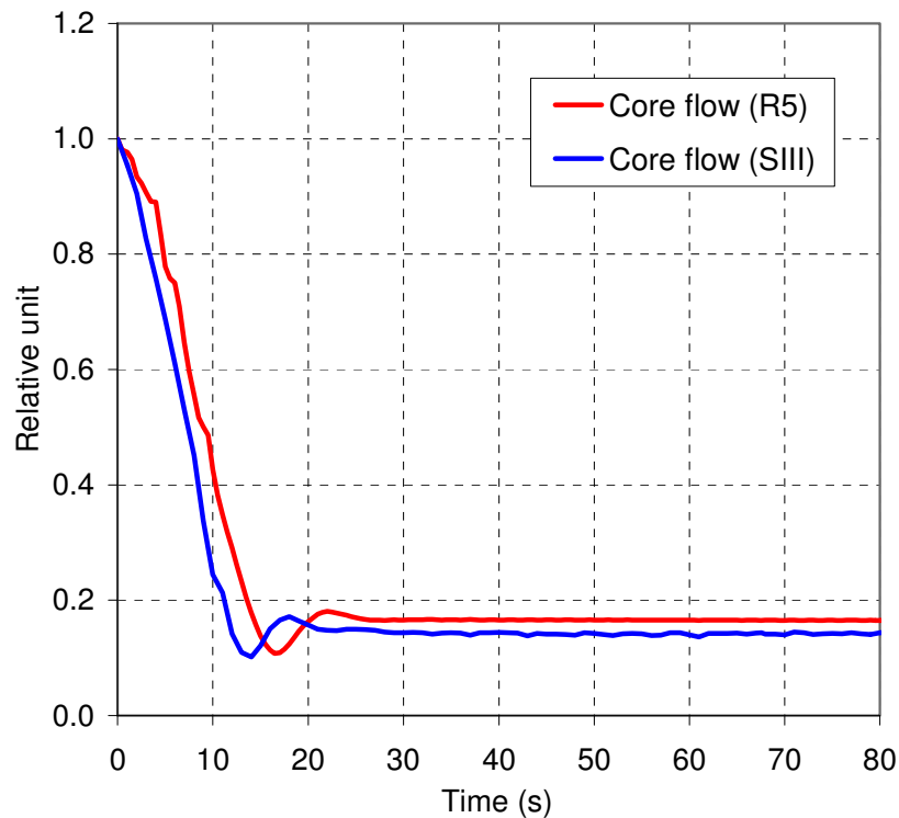
Figure 5.3: Core mass flow rate evolution in the ULOF transient.
