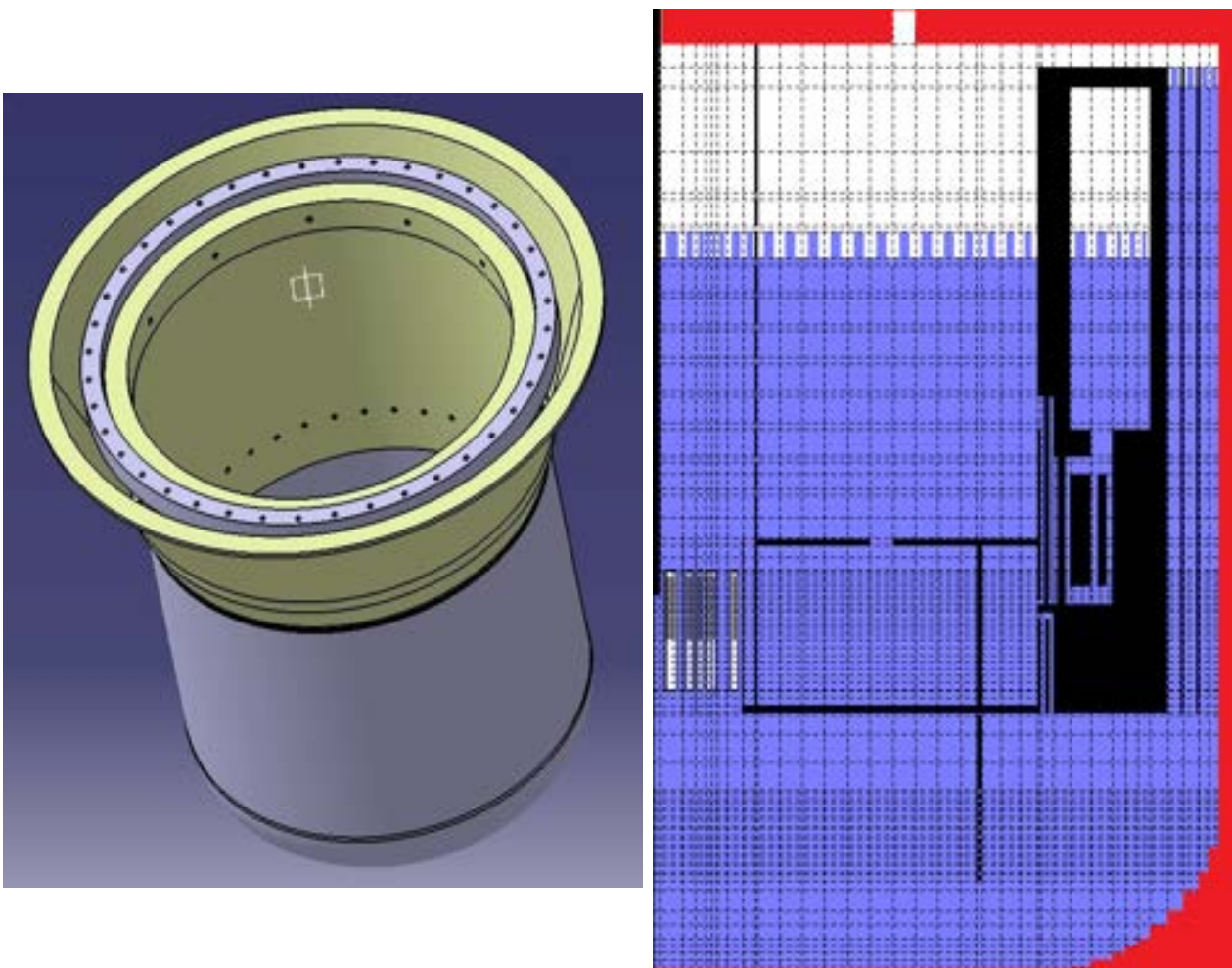
Figure 3.6: Reactor vessel model in CAD and in SIMMER-III.
