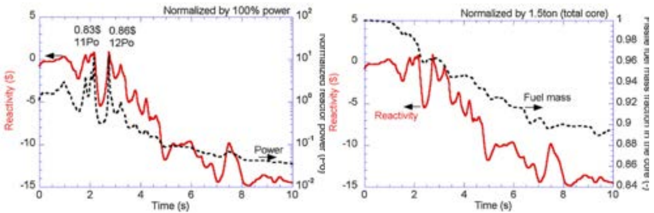
Figure 2.7: Reactivity, power and fuel mass fraction in the core.
