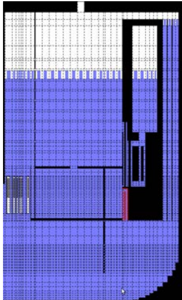
Figure 3.10: Pump model in CAD and in SIMMER-III.
