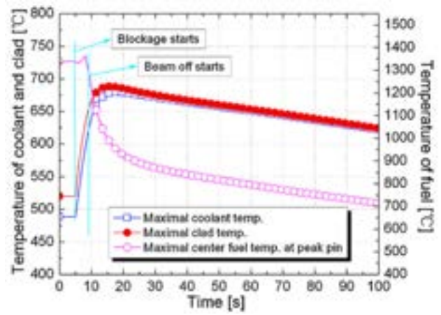
Figure 2.5: Highest clad temperature in UBA and temperature transient in PBA.
