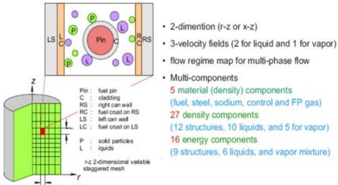
Figure 1.2: Multi-phase, multi-component fluid-dynamics model in SIMMER-III.
