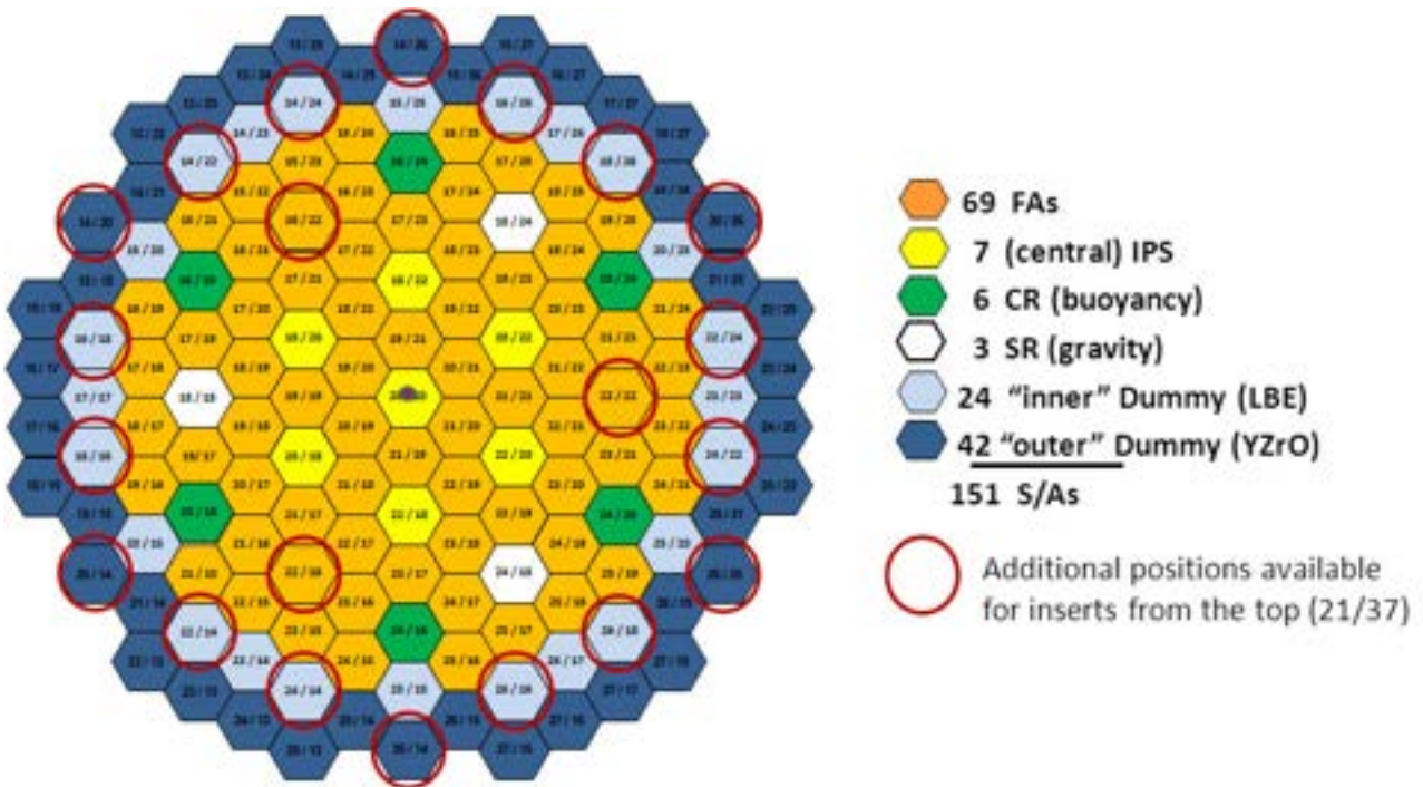
Figure 3.2: 100 MW - 69 FA critical core layout.
