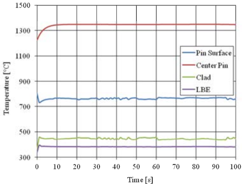
Figure 4.2: Temperature trends in cell [2,52] (middle of core).
