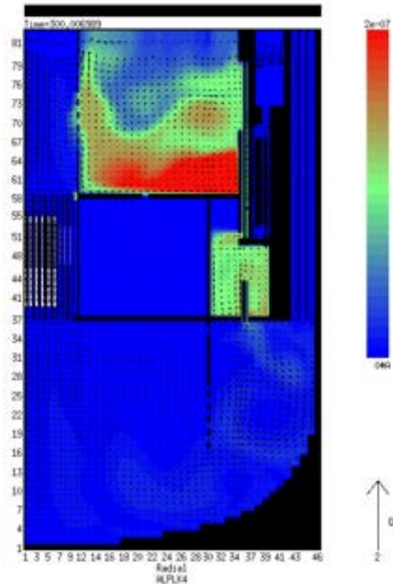
Figure 5.9: Fuel particle concentration in the primary circuit at t = 300 s (fuel porosity = 5%).
