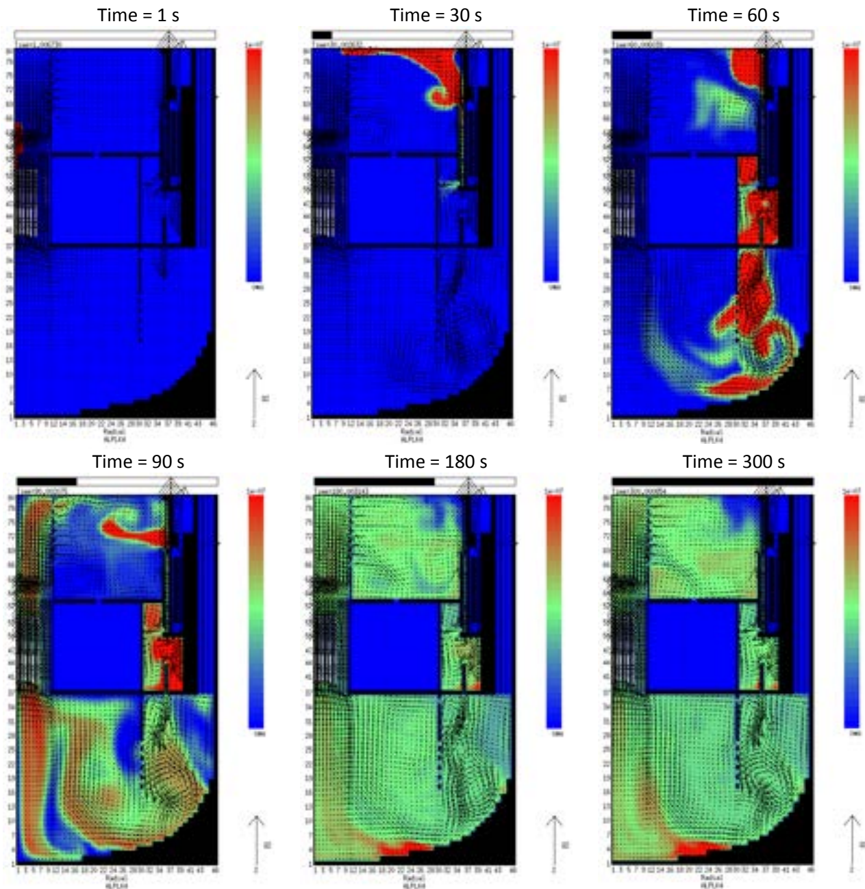
Figure 5.6: Evolution of fuel particle concentration in the primary circuit (fuel porosity = 5%).
