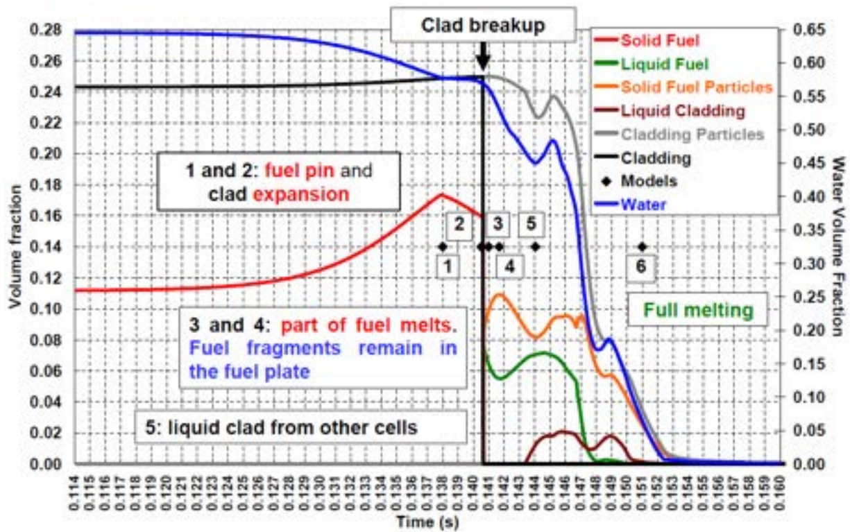
Figure 2.15: Assessment of degraded fuel SA models.
