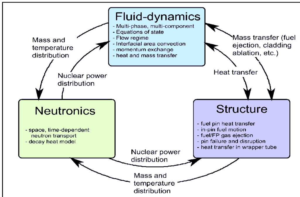
Figure 1.1: Overall framework of SIMMER-III code.
