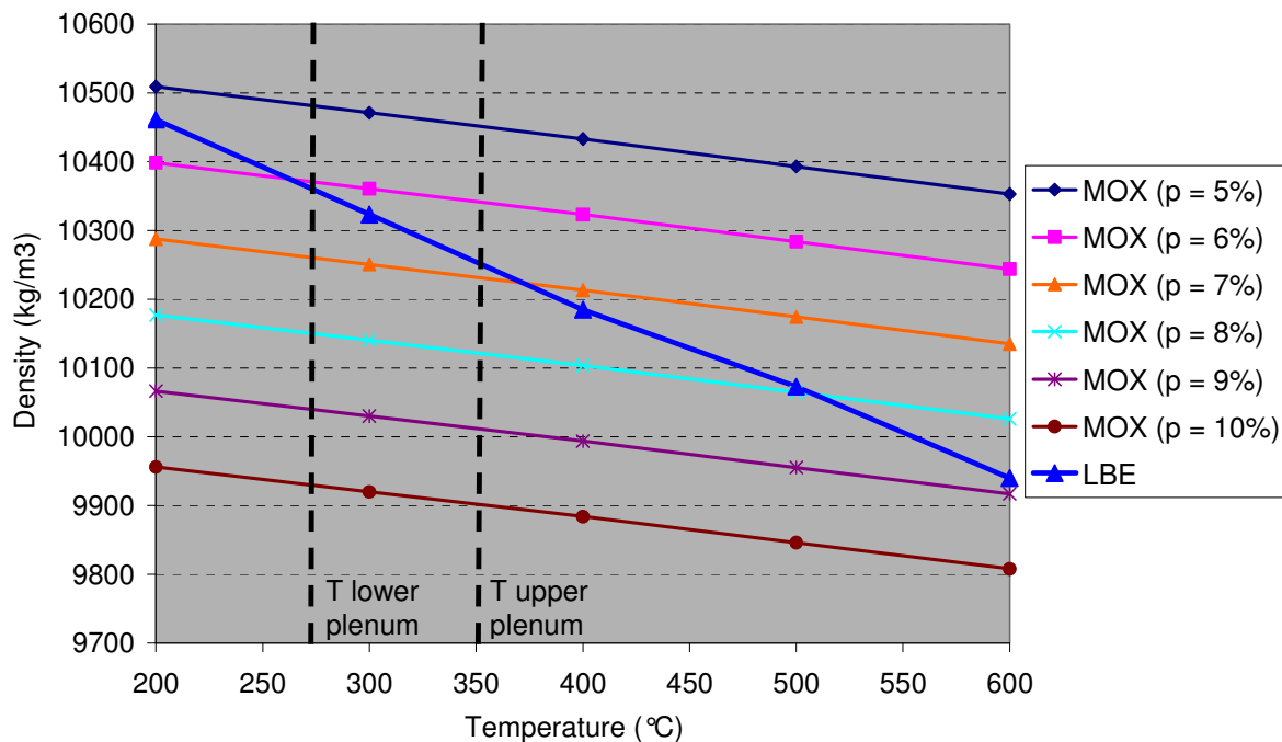
Figure 5.5: Density versus temperature for LBE and MOX with different porosity.
