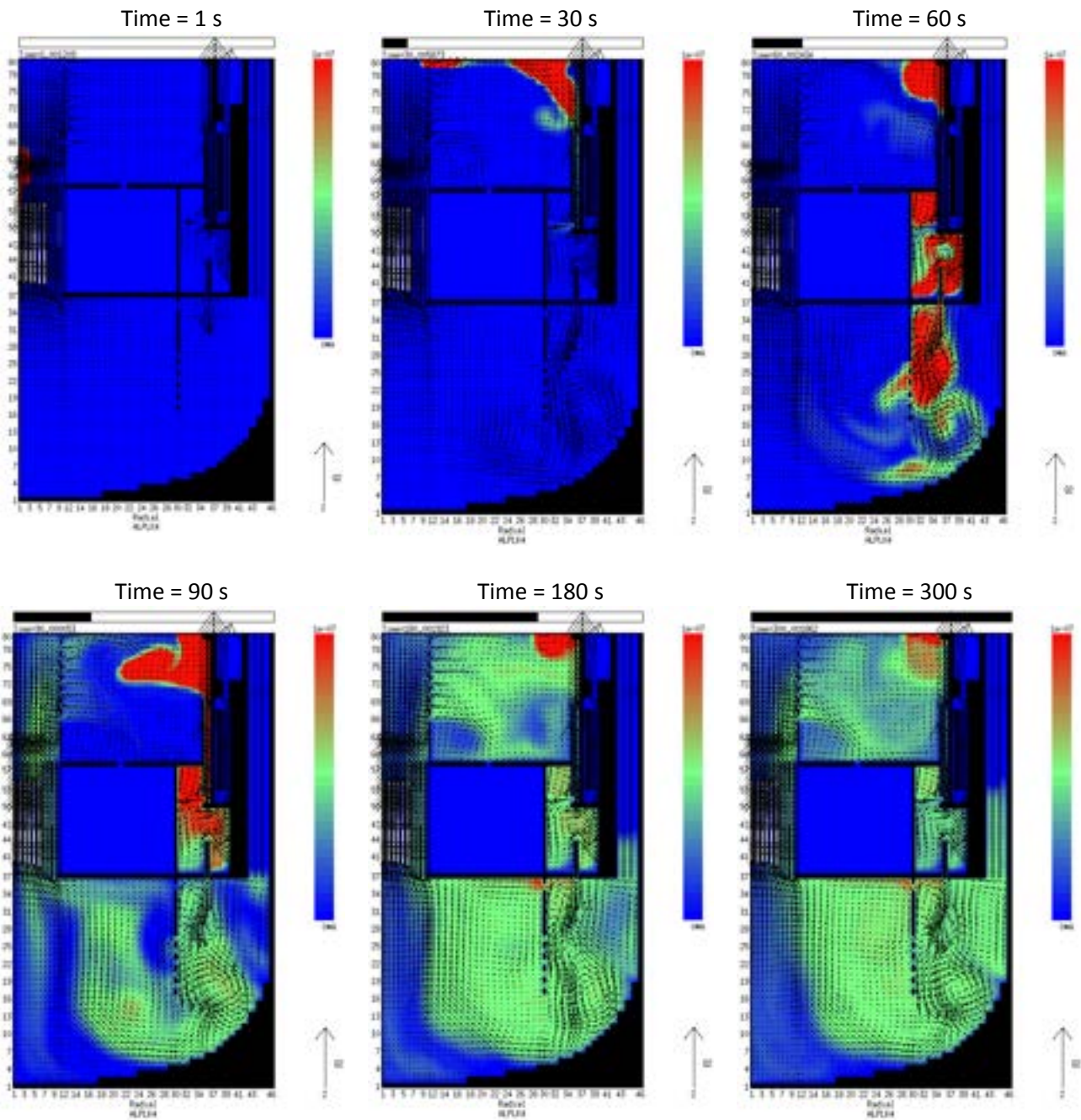
Figure 5.7: Evolution of fuel particle concentration in the primary circuit (fuel porosity = 10%).
