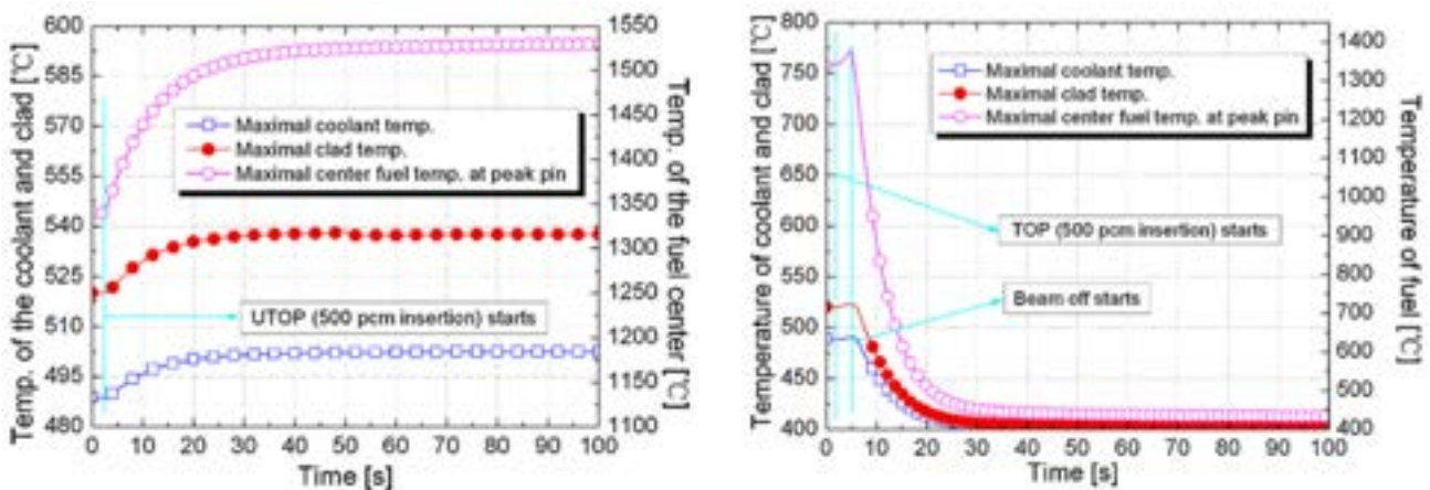
Figure 2.3: Temperature transients in the UTOP and PTOP cases.
