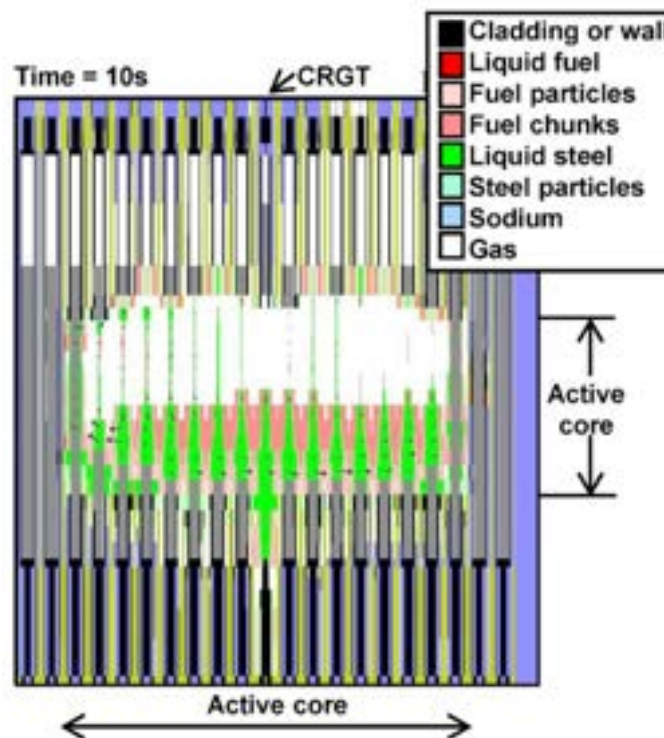
Figure 2.9: Disruptive core relocation.
