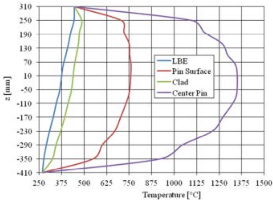
Figure 4.3: Axially temperature profile in the active fuel zone in second ring.
