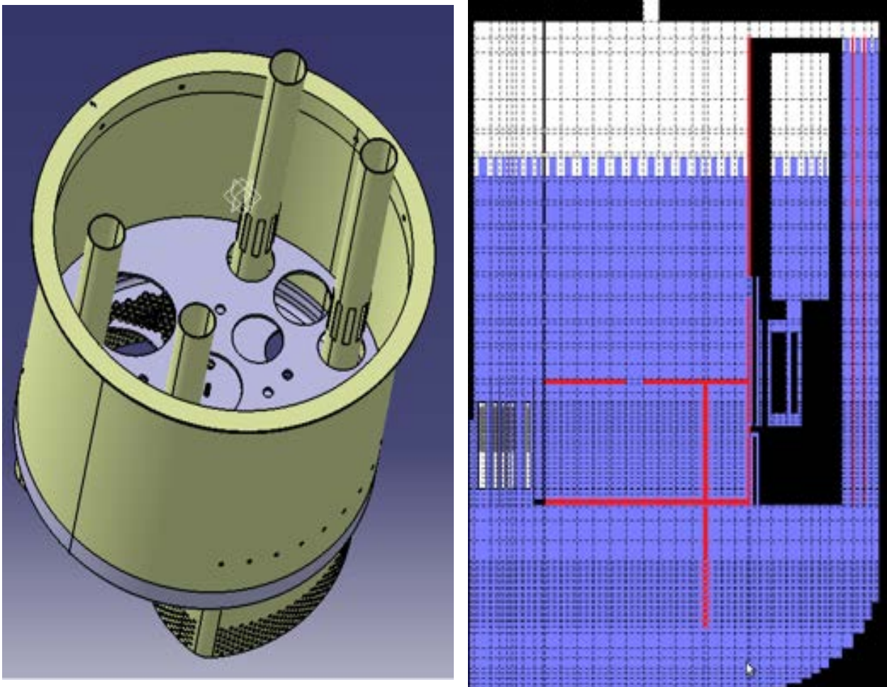
Figure 3.7: Diaphragm model in CAD and in SIMMER-III.
