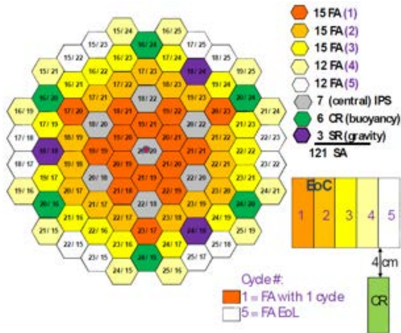
Figure 3.4: 100 MW - 69 FA EoC core layout (CR completely withdrawn).
