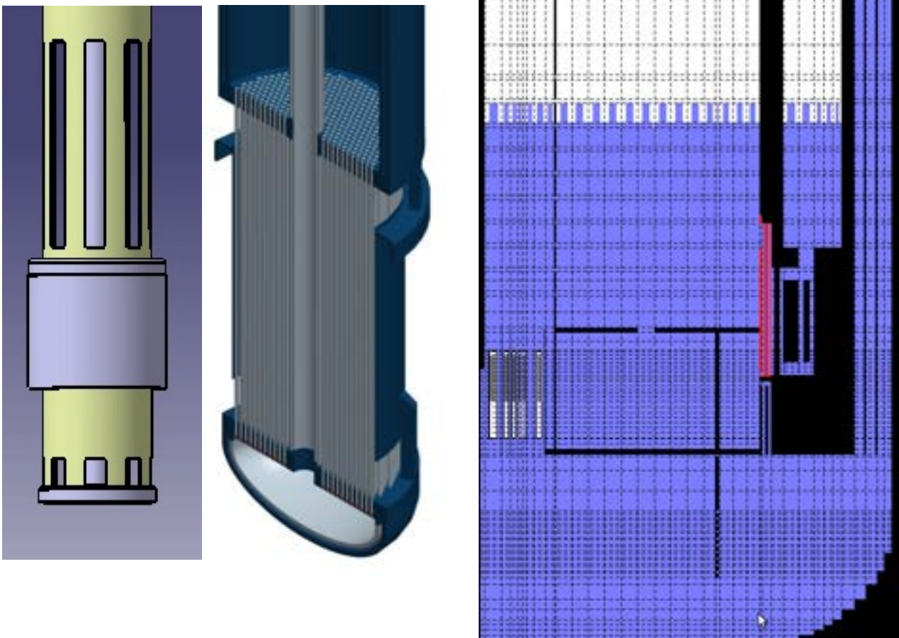
Figure 3.9: PHX model in CAD and in SIMMER-III.
