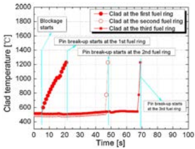
Figure 2.5: Highest clad temperature in UBA and temperature transient in PBA.
