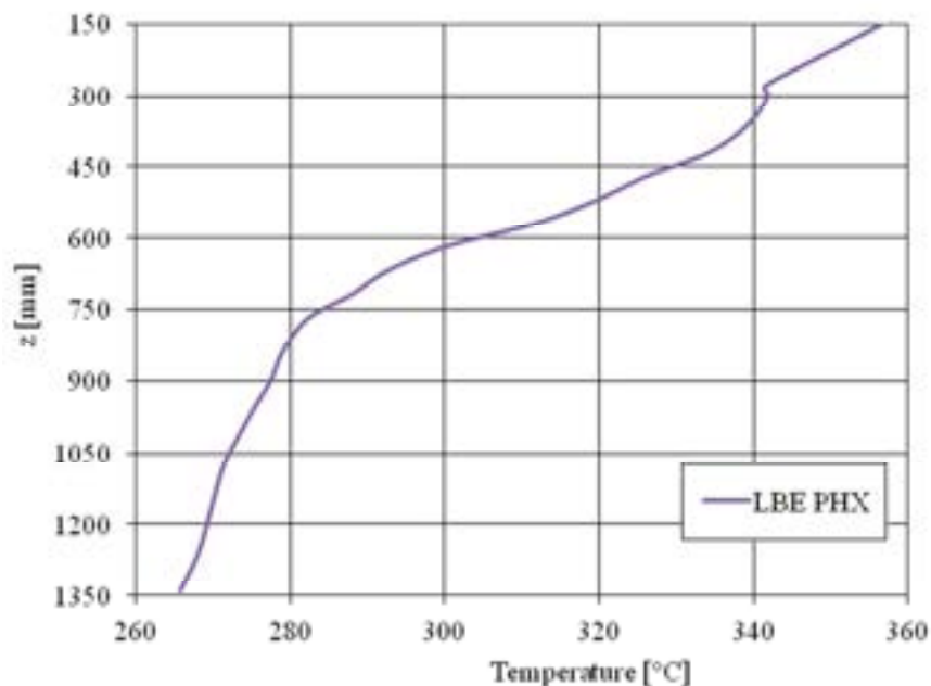
Figure 4.4: LBE temperature profile in PHX.
