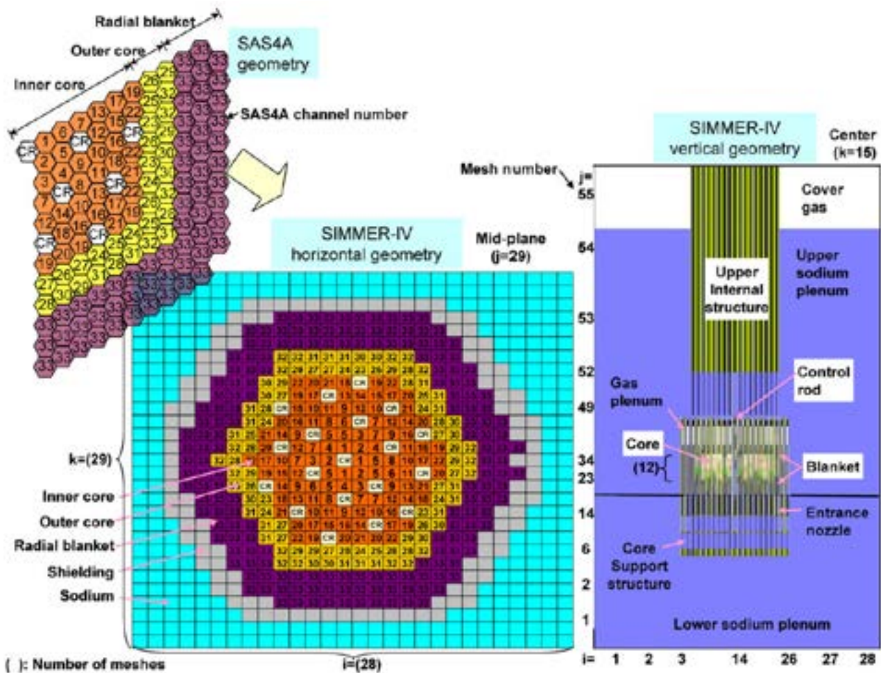
Figure 2.6: SFR Geometry in SIMMER-IV simulation.
