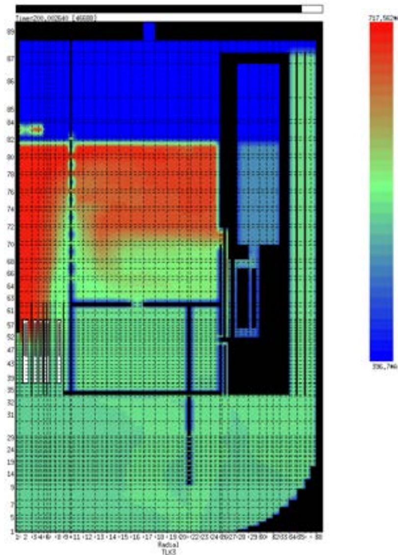
Figure 4.1: LBE temperature at steady-state conditions.
