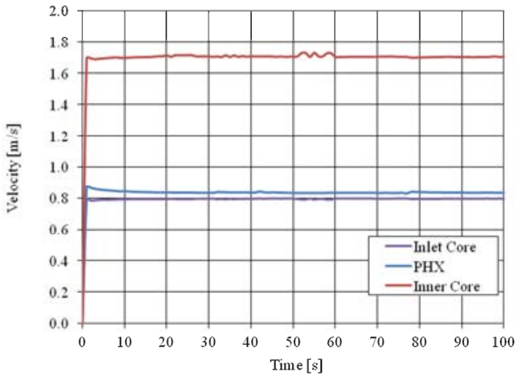
Figure 4.6: Velocity in the second ring at the inlet and inner of core and in the PHX.
