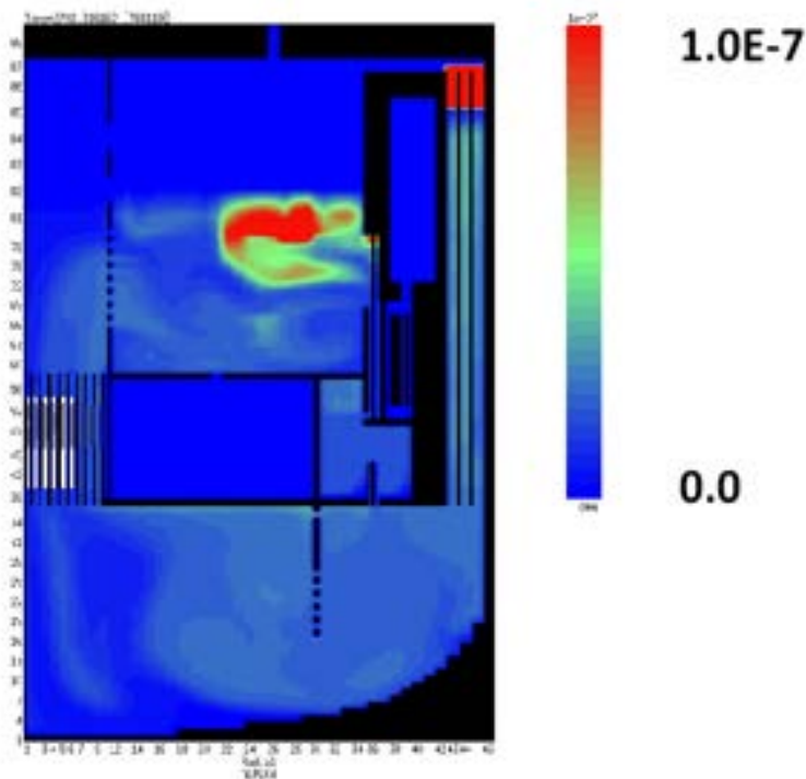
Figure 5.8: Fuel particle concentration in the primary circuit at t = 2700 s (fuel porosity = 10%).
