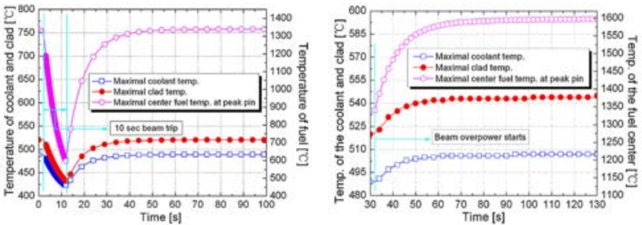
Figure 2.2: Temperature transients in the BT case and in the beam overpower.
