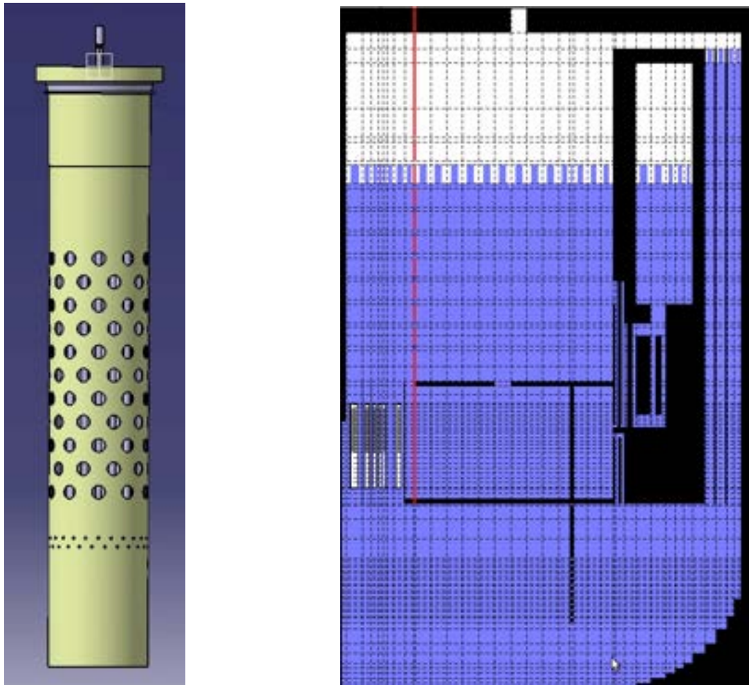
Figure 3.8: Barrel model in CAD and in SIMMER-III.
