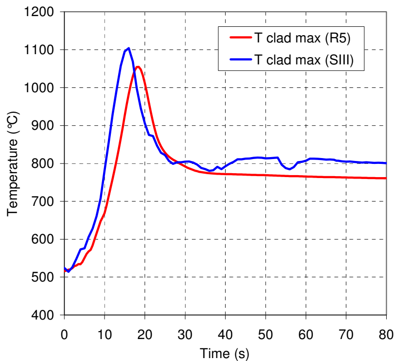
Figure 5.4: Maximum clad temperature evolution in the ULOF transient.
