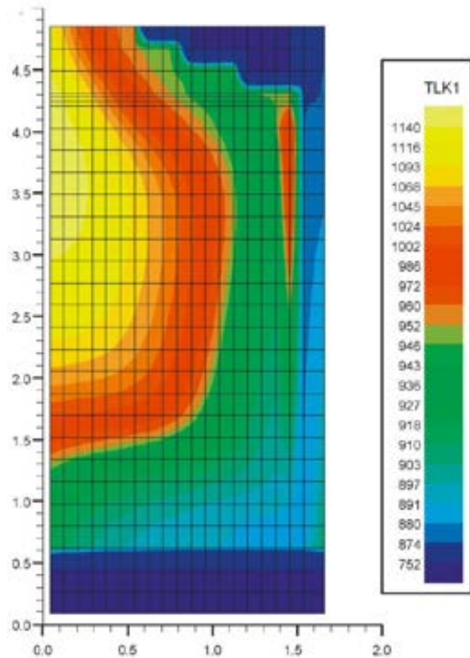
Figure 2.13: 2D Temperature distribution.
