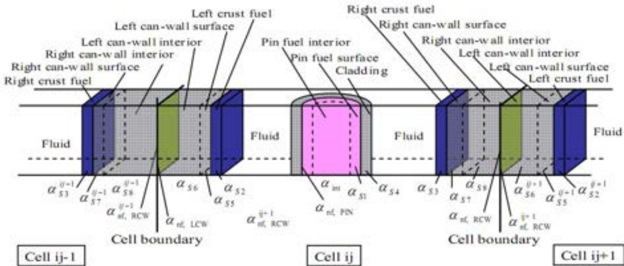
Figure 1.5: Fuel pin and can wall configuration in a mesh cell.
