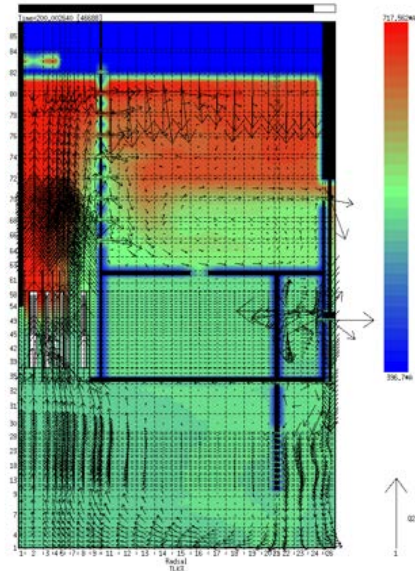
Figure 4.5: LBE velocity fields in steady-state conditions.
