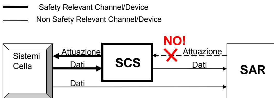
Fig. 7: Connessione SCS – SAR
