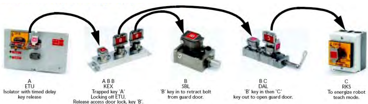
Fig. A.1: Trapped Key Interlocking
