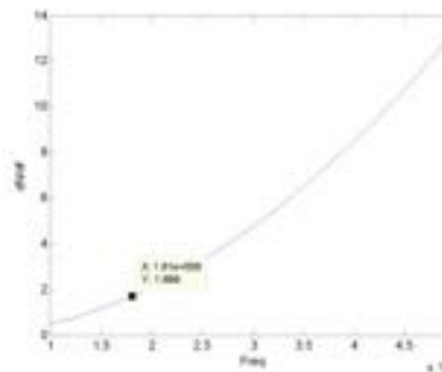
Fig 4: Theoretical mode density for the ENEA shielded room.
