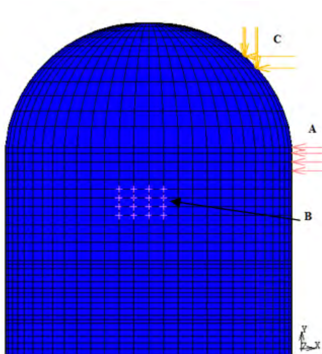
Figure 14 - Entry directions in the aircraft impact analyses
