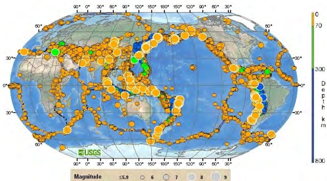
Figure 3 – Seismicity map
