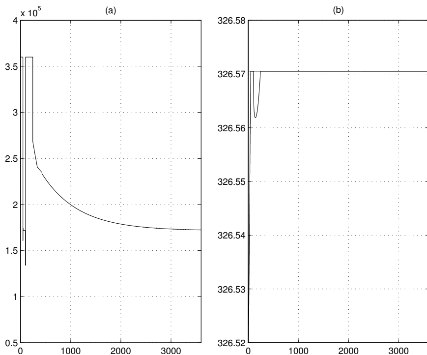
Figure 21: Controllers (18), (37). (a) Pressurizer heating power W_{heat,pr} [kW]; (b) Pressurizer temperature T_{pr} (solid) and estimate \hat{T}_{pr} (dashed) [ ^{\circ}\text{C} ]
