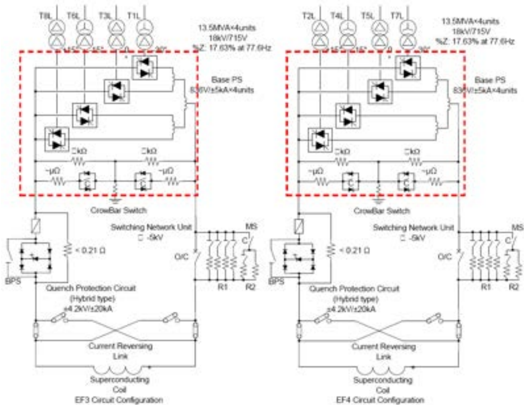
Figure 4.4.1-1 JT-60SA PFC reference schemes
