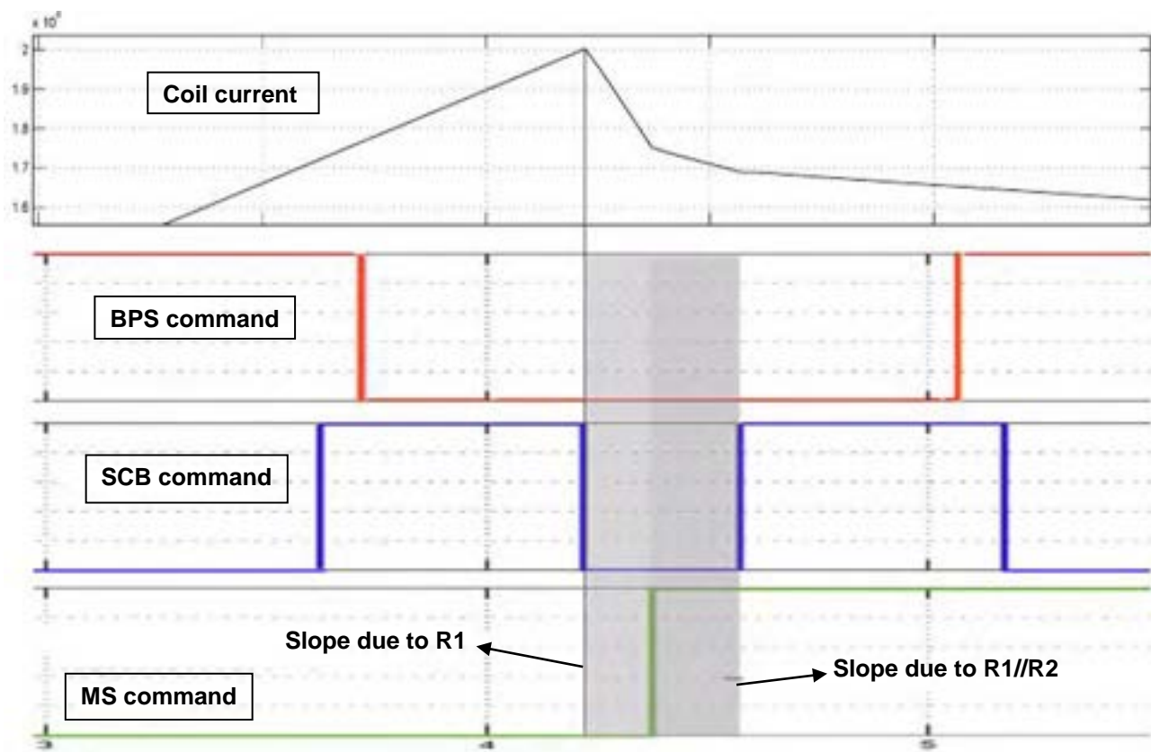
Fig. 11: Example of switching operations in the hybrid scheme. At the breakdown, the current abruptly decreases with two different slopes due to the SNU resistors R1 and R2.
