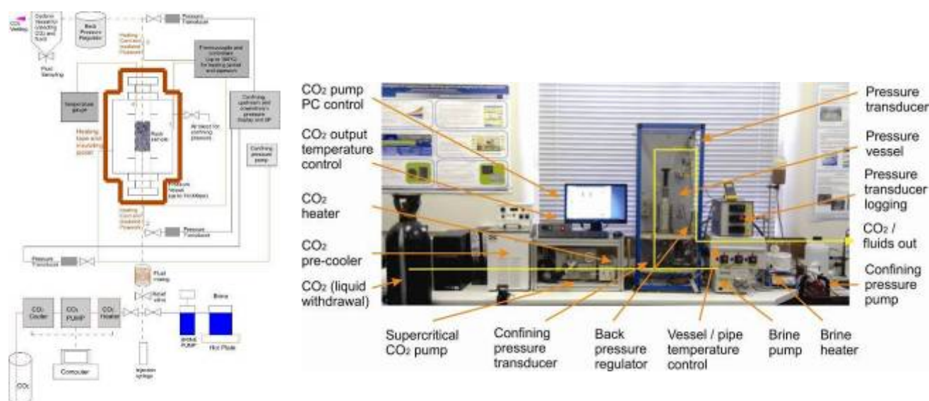
Fig 1 .COFR: CO2 Flow rig Transport and Storage, Laboratory
