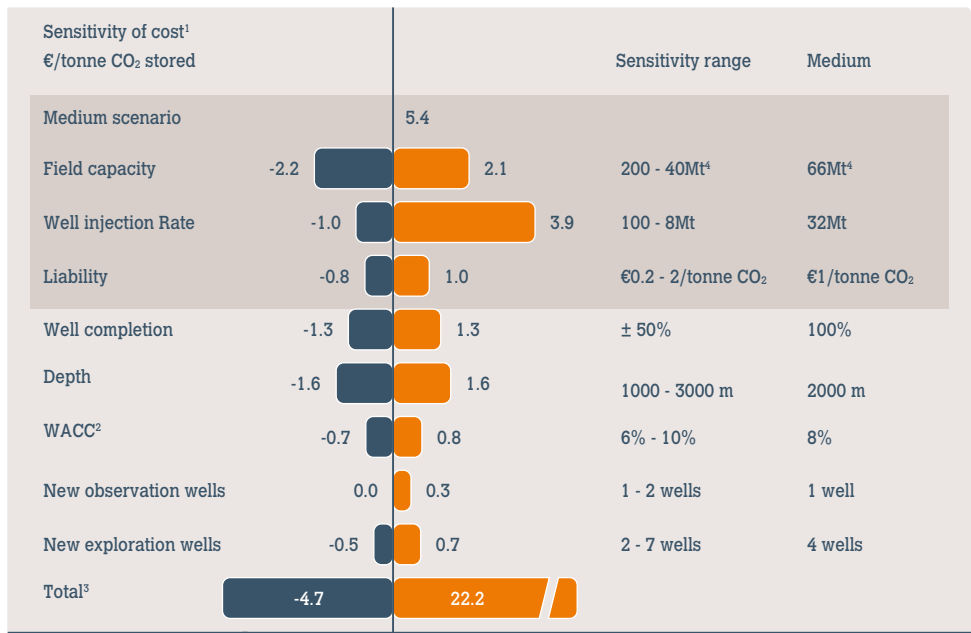
Figure 20: Illustration of sensitivities in the storage cost calculations for one storage case
