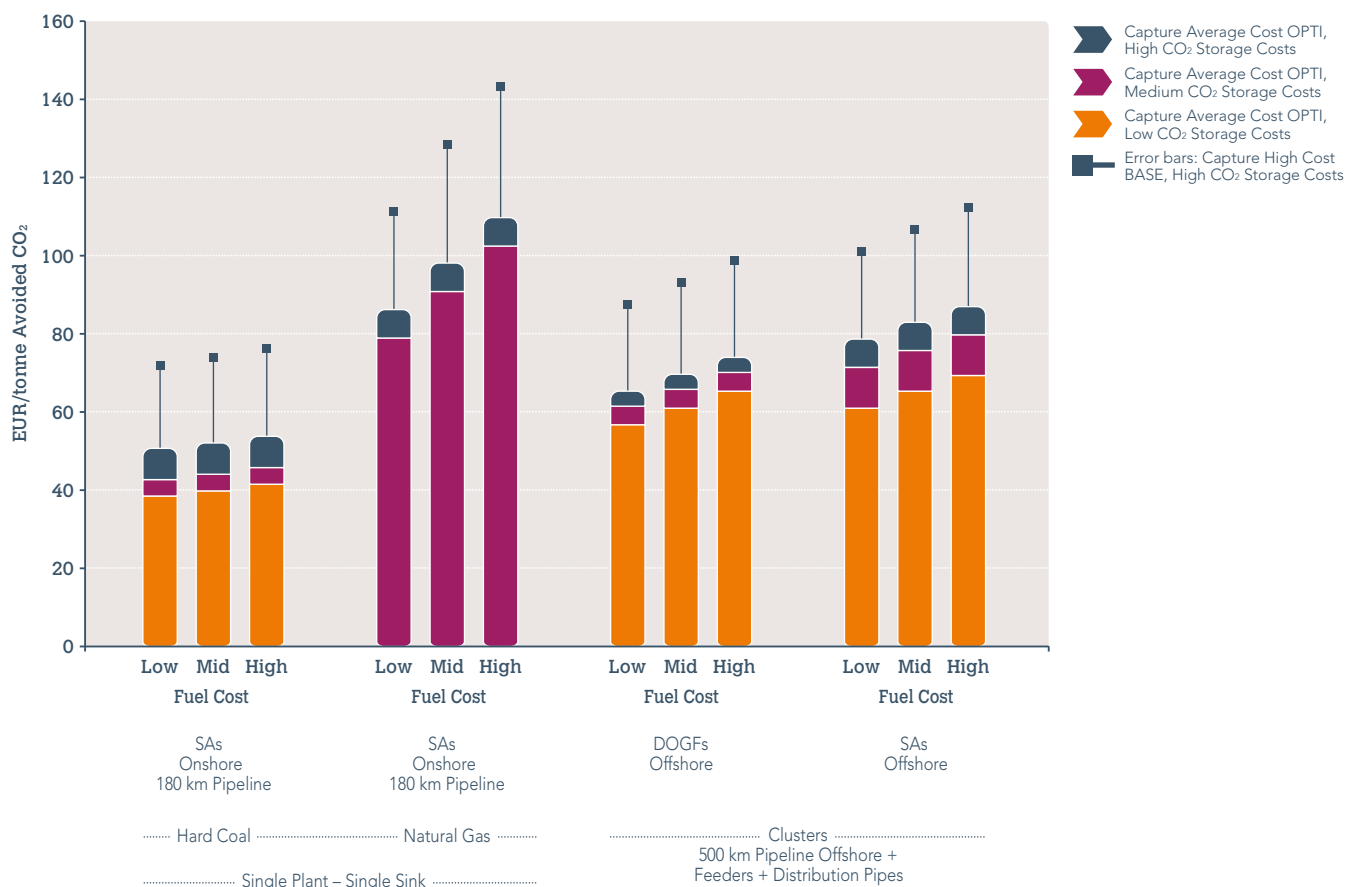
Figure 10: Total CO 2 avoidance costs for integrated CCS projects – the price of EUAs required to justify building CCS projects vs. a plant without CCS from a purely economic point of view.
