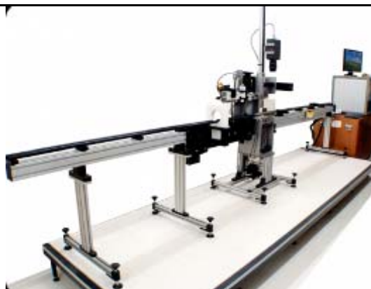
View of the two equipments within the CCSLAB: The MSCL-S system for laboratory core logging & Benchtop liquid permeability system to be upgraded for CO 2 (sc) studies
