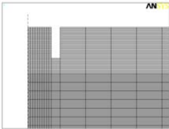
Fig. 3.3 detail of the axisymmetric FEM model of the ring drilling procedure: step 20 of 30.
