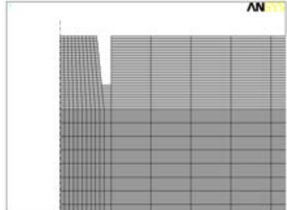
Fig. 3.4 detail of the axisymmetric FEM model with slope: step 20 of 30.
