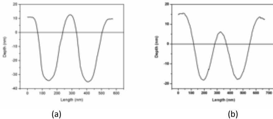
Figure 12. Two boxes milled by fixed dose of 9 \times 10^{16} ions/cm 2 with a magnification of (a) 19716x (D= 34nm, W=168nm) and (b) 8308x (D=18nm, W=178nm)
