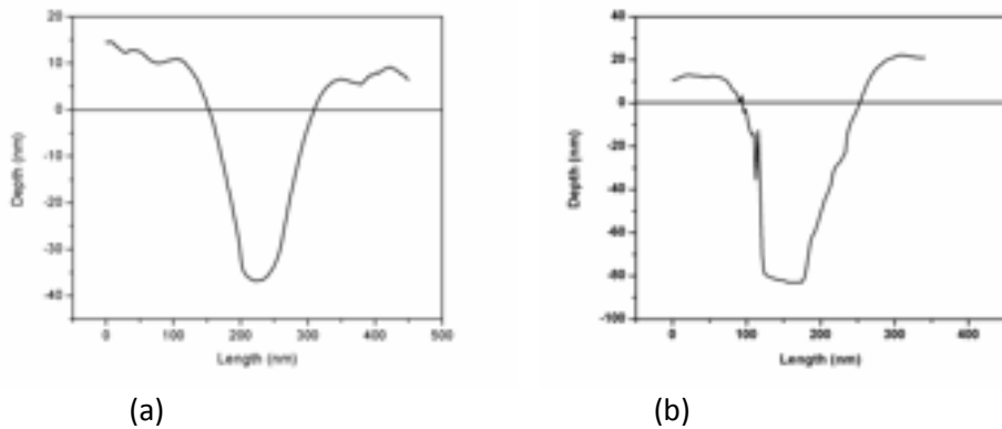
Figure 14. AFM profile of the milled trenches at (a) Ion current is 50pA, dose is 9 \times 10^{16} ions/cm 2 , dwell time is 1 \mu s and passes are 271 (D= 36nm, W=158nm), (b) Ion current is 1pA, dose is 3 \times 10^{17} ions/cm 2 , dwell time is 1 \mu s and passes are 6125 (D=83nm, W=158nm)
