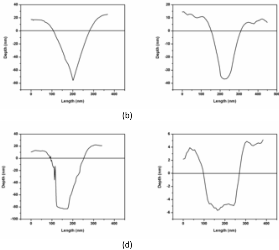
Figure 15. AFM profiles of the milled trenches at 50pA with doses a) 5 \times 10^{17} ions/cm 2 ( D=75\text{nm} , W=174\text{nm} ) and b) 9 \times 10^{16} ions/cm 2 ( D=37\text{nm} , W=156\text{nm} ); and at 1pA with doses (c) 3 \times 10^{17} ions/cm 2 ( D=83\text{nm} , W=158\text{nm} ) and (d) 5 \times 10^{16} ions/cm 2 ( D=5\text{nm} , W=172\text{nm} )
