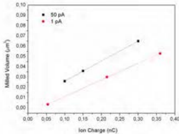
Figure 17. Milled volume dependence from the ion charge for different currents (1pA and 50pA). Straight lines represent the best fit
