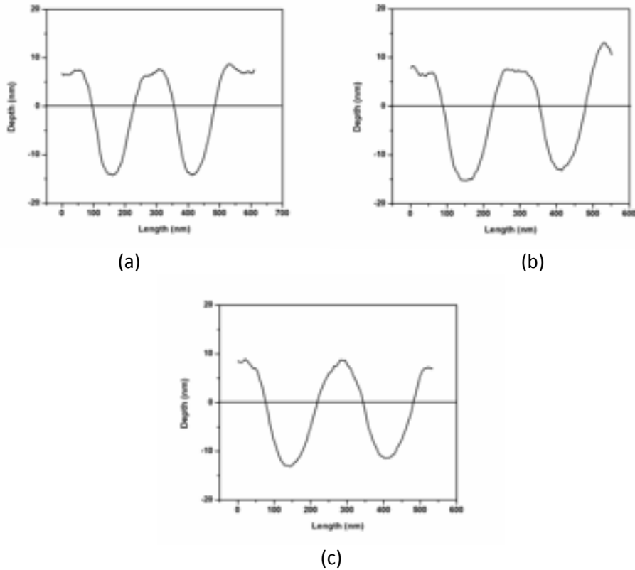
Figure 13. AFM profiles of the milled trenches at fixed current, 1pA, and different dwell times (a) 1 \mu s (D=14nm, W=133nm) (b) 500ns (D=13-15nm, W=138nm) and (c) 100 ns (D=11-13nm, W=142nm)
