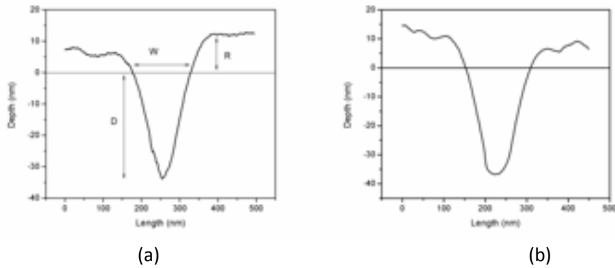
Figure 11. AFM images of the milled trenches with different milling direction. In (a), depth, D, width, W, and surface redeposition, R, (typically around 10nm) are drawn starting from the original surface at 0 value. (a) Milling direction “right to left” (D=33nm, W=152nm) and (b) “bottom to top” (D=37nm, W=156nm)
