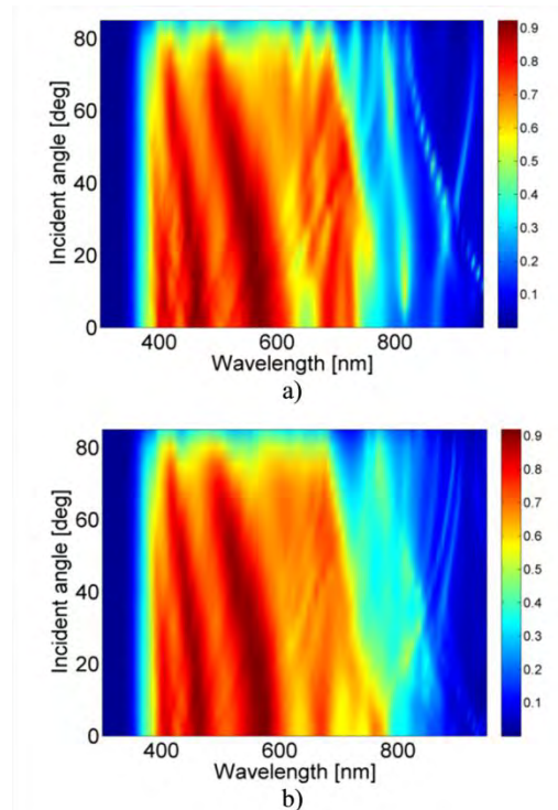
Figure 8. Pseudo color plot of the absorption of periodic (a) and Fibonacci (b) configuration of Fig. 1d as function of the incident angle \theta evaluated in range [0-85]^\circ .
