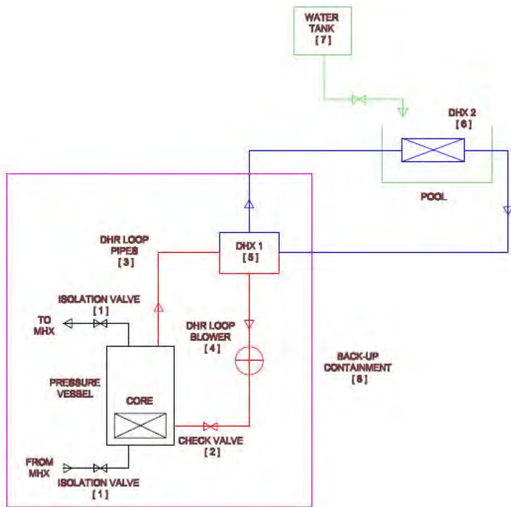
Figure 8. Scheme of a Demonstrator DHR loop
