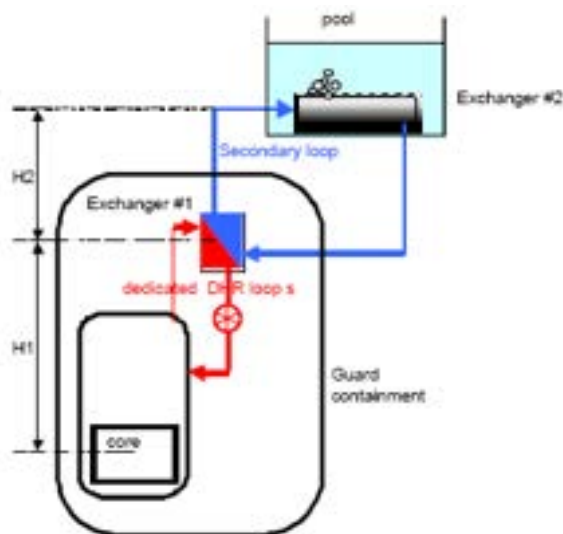
Figure 1. Schematic of the DHR system
