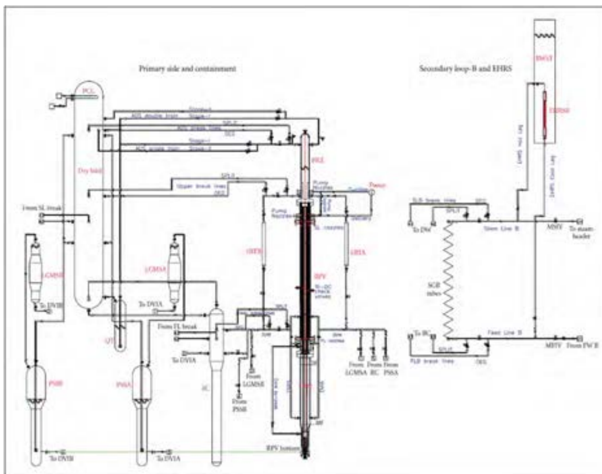
Fig.1 – SPES-3 Layout
