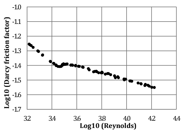
Figure 1.28 Experimental friction factor profile for Coil
