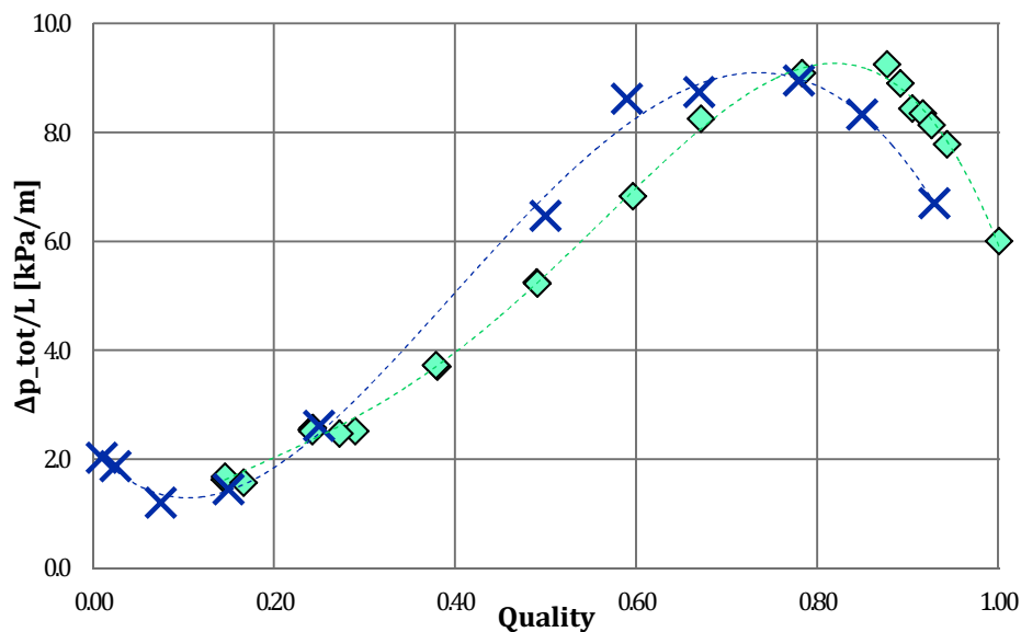
Figure 3.12 Pressure drop results of CFD study with two-phase model and Fine Mesh (Simulation 06 excluded)
