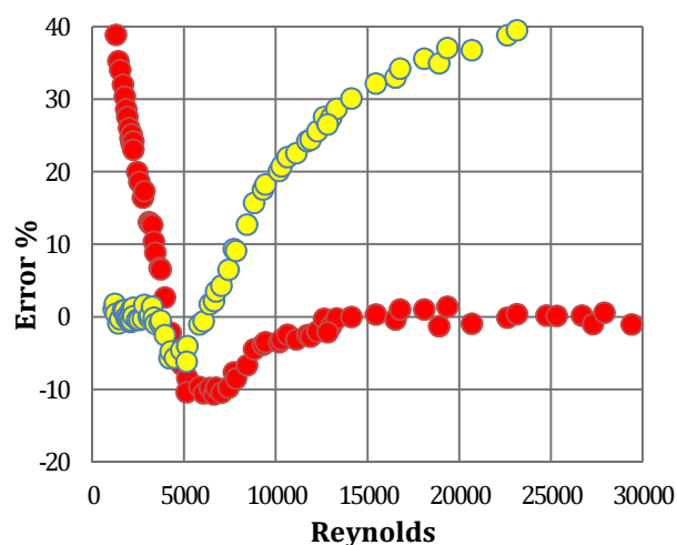
Figure 1.39 Relative error between Ito's formulas and experimental data of Coil 06
