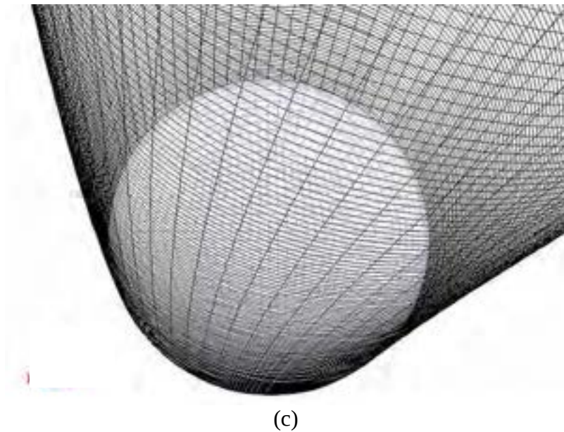
Figure 3.2 Global view (a), section view (b) and wall view (c) of the fine mesh
