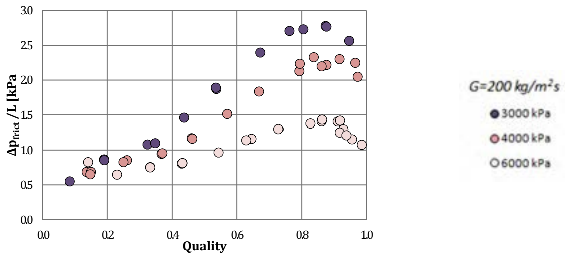
Figure 2.6 Experimental data of \Delta p_{\text{frict}} per unit of length vs. quality in SIET Facility helically coiled pipe (no power input) at three different pressure levels for a given mass flux value
