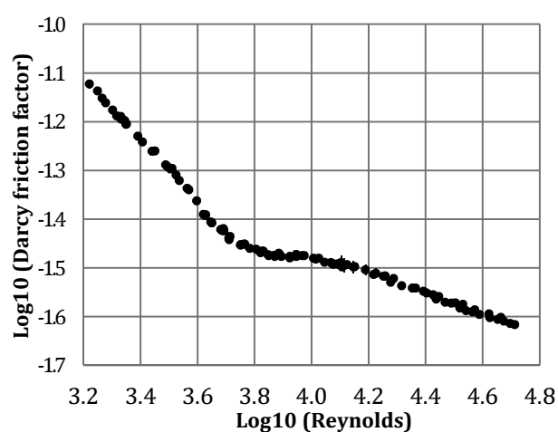
Figure 1.22 Experimental friction factor profile for Coil 06
