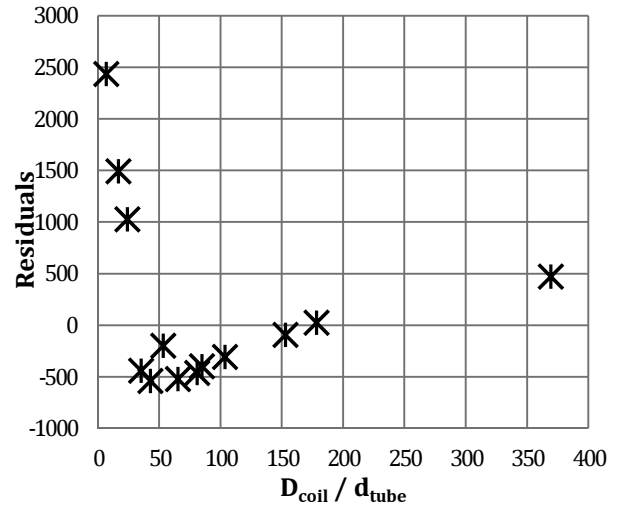
Figure 1.51 Residual plot of model in eq. (1.43)
