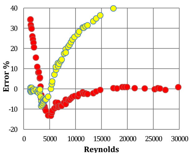
Figure 1.41 Relative error between Ito's formulas and experimental data of Coil 08
