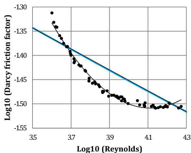
Figure 1.53 Re_{crit\_2} determination for Coil 04
