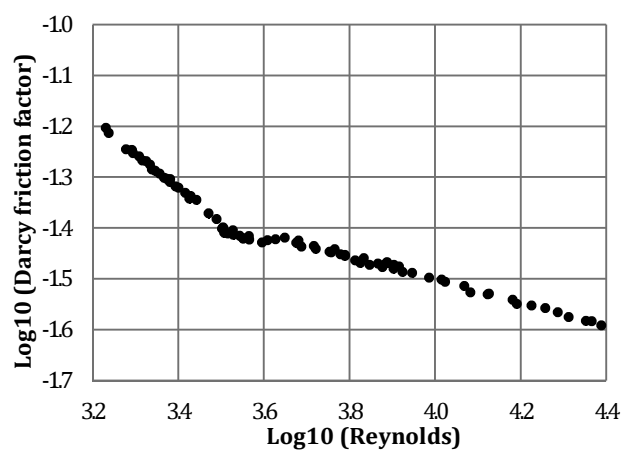
Figure 1.26 Experimental friction factor profile for Coil
