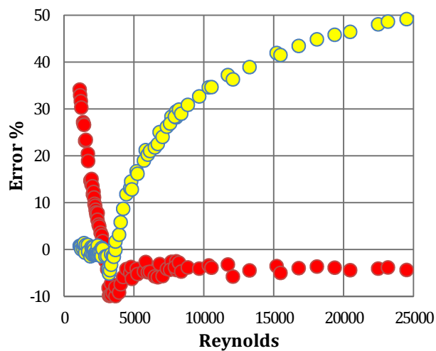
Figure 1.43 Relative error between Ito's formulas and experimental data of Coil 10
