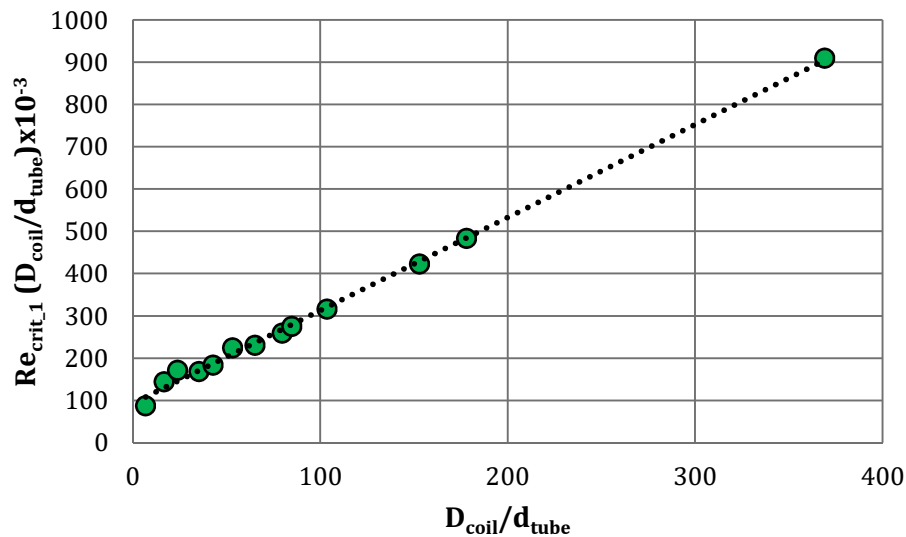
Figure 1.47 Plot of the product Re_{crit\_1} \cdot \left(\frac{D_{coil}}{d_{tube}}\right) vs. curvature ratio and linear fitting
