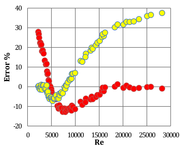
Figure 1.37 Relative error between Ito's formulas and experimental data of Coil 04
