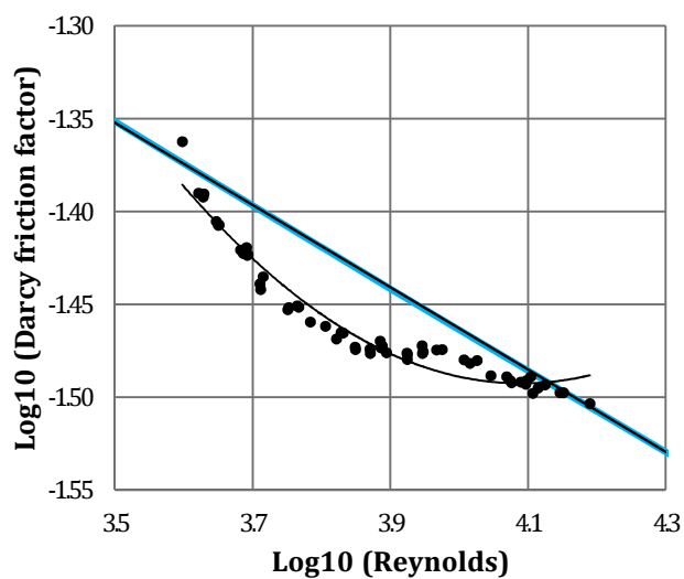
Figure 1.55 Re_{crit\_2} determination for Coil 06
