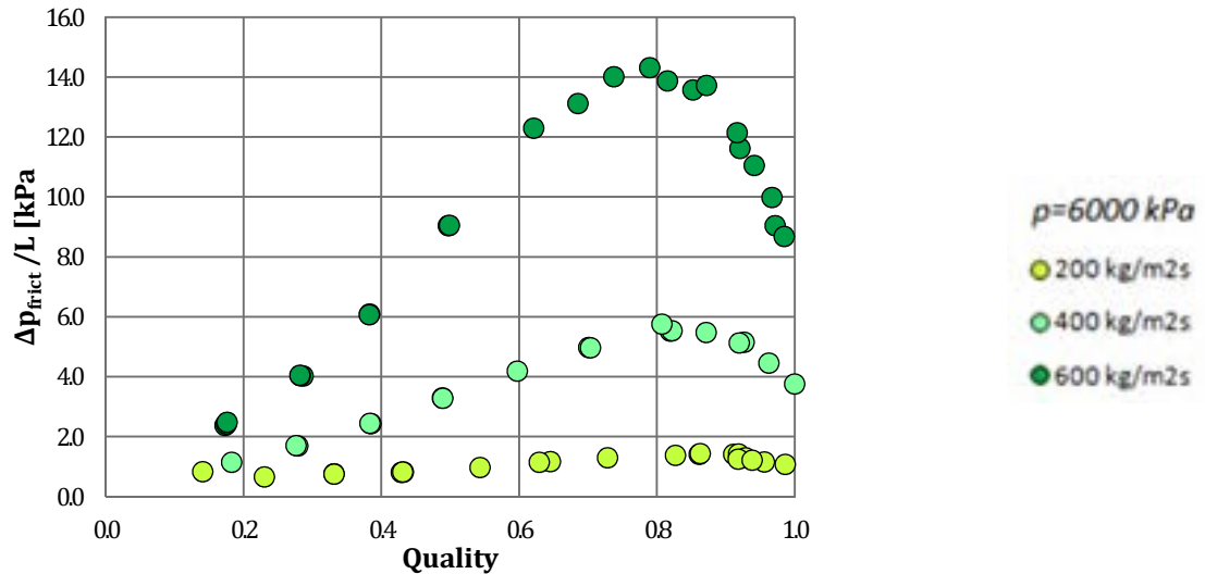
Figure 2.5 Experimental data of \Delta p_{\text{frict}} per unit of length vs. quality in SIET Facility helically coiled pipe (no power input) at three different mass flux levels for a given pressure value
