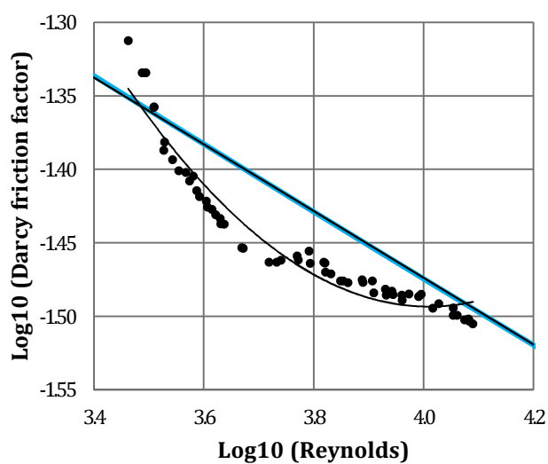
Figure 1.57 Re_{crit,2} determination for Coil 08
