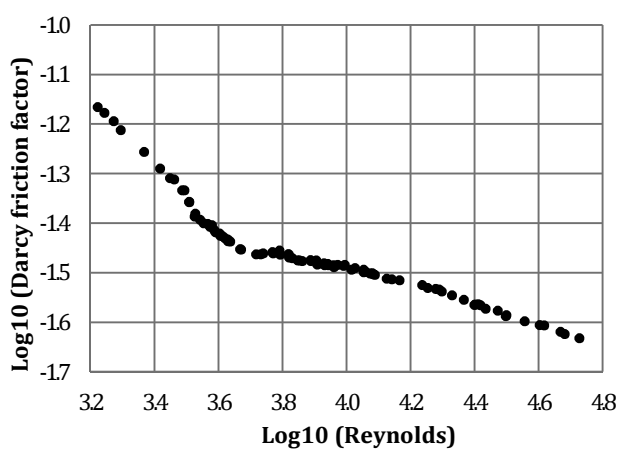
Figure 1.24 Experimental friction factor profile for Coil 08
