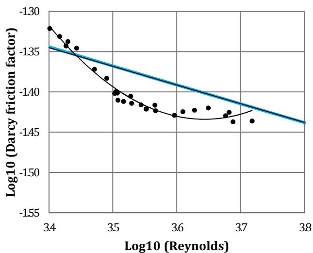
Figure 1.59 Re_{crit,2} determination for Coil 10
