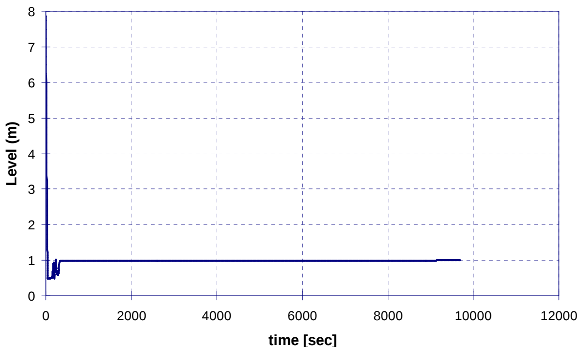
Figure 3.3: Steam generator A level
