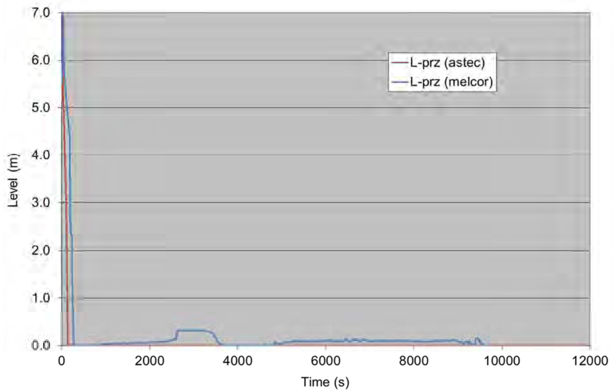
Figure 5.6: Pressurizer level
