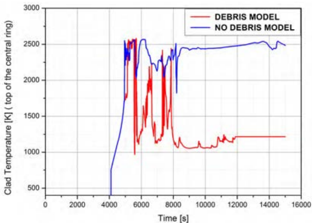
Figure 4.11: Cladding temperature (central ring)
