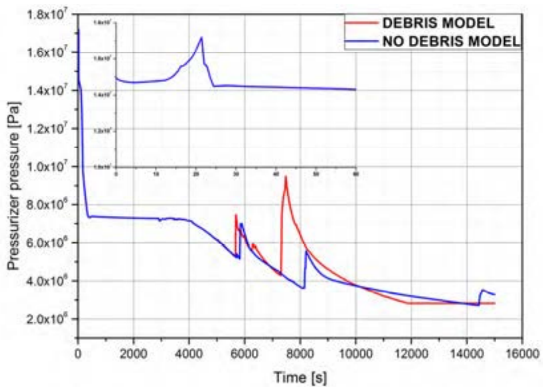
Figure 4.5: Pressurizer pressure
