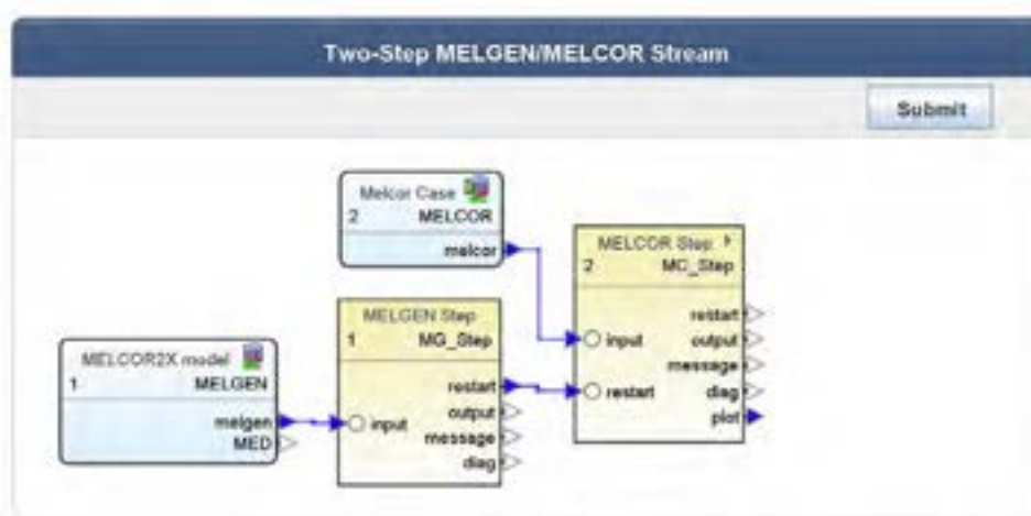
Figure 12: SNAP two-step MELGEN MELCOR stream.
