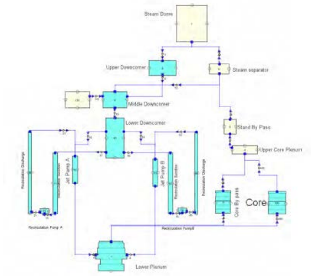
Figure 7: RPV MELCOR nodalization.
