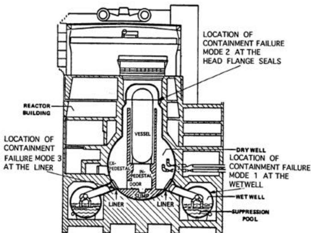
Figure 5: Peach Bottom Mark 1 containment and failure mode [12].
