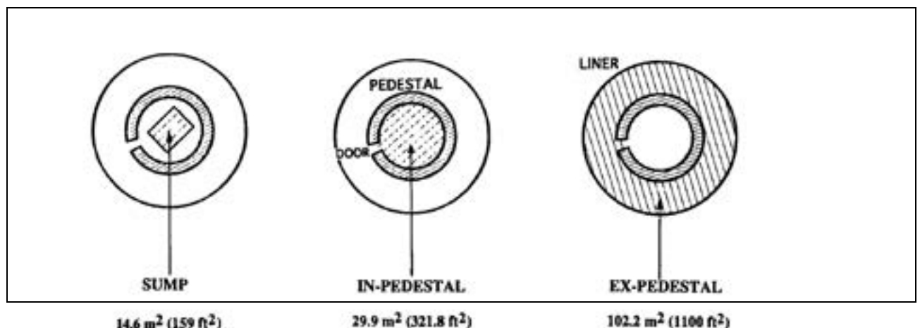
Figure 6: Horizontal view of the in-pedestal, ex-pedestal and sump cavity region [12]
