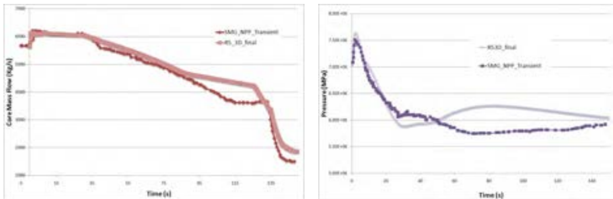
Figure 25 : On-transient qualification: Core Mass flow (kg/s, left), Steam Dome pressure (MPa, right)
