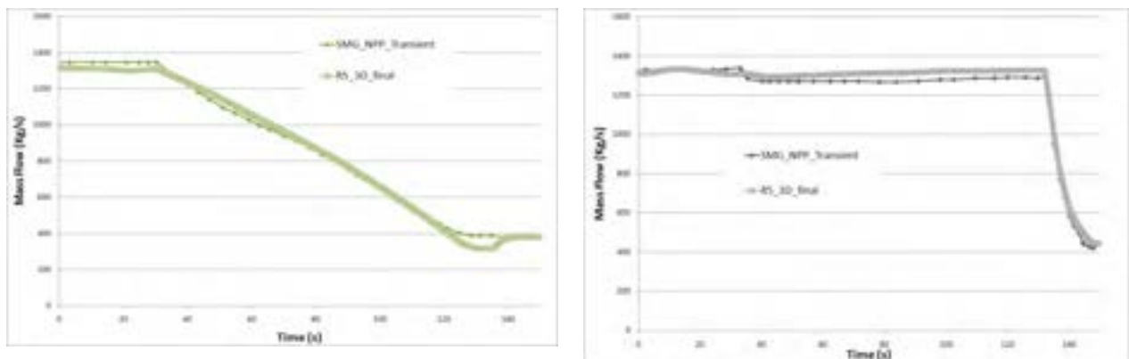
Figure 26: On-transient qualification: Recirculation line mass flows (kg/s), line A (left), line B (right)
