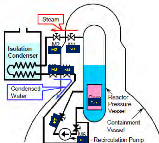
Figure 1 Piping of Isolation Condenser
