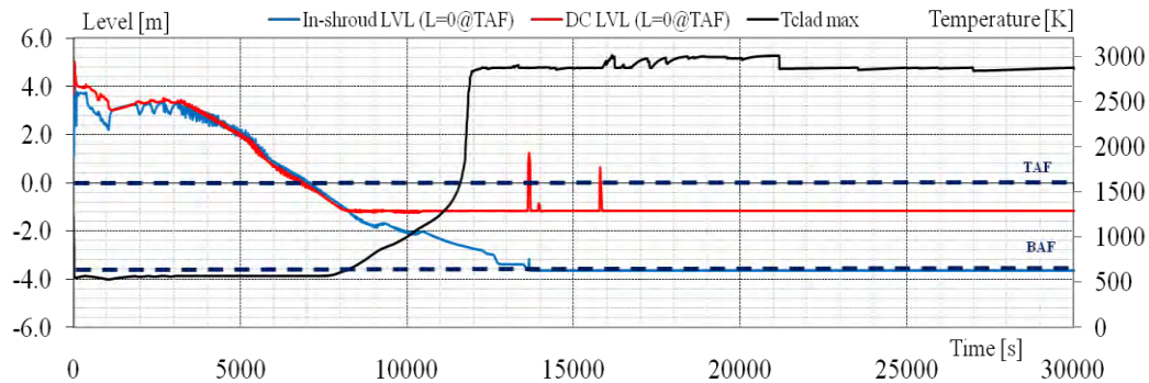
Figure 28: RPV DC and in-shroud level (m), Hot spot clad temperature ( ^{\circ}\text{C} )
