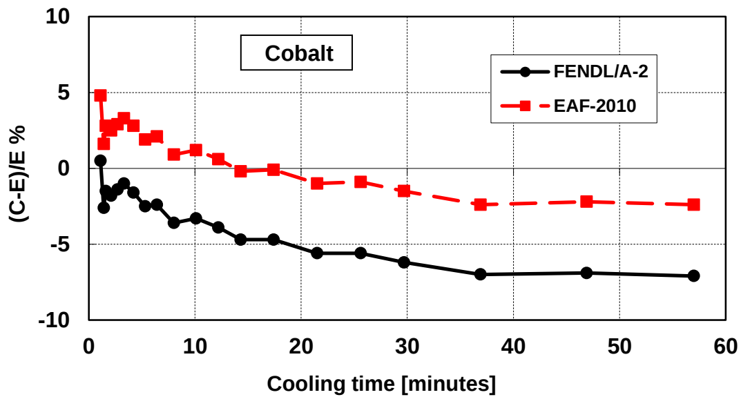
Figure 12 – Decay heat vs. cooling time of Cobalt sample irradiated for 5 min. Comparison of calculation with experiment (C-E)/E %.
