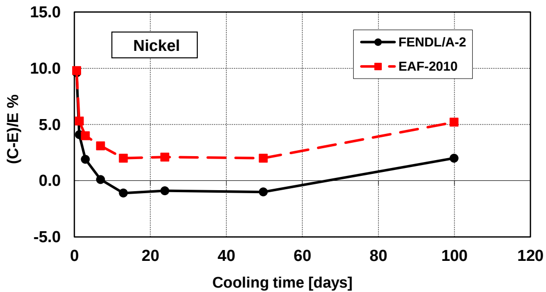
Figure 33 – Decay heat vs. cooling time of Nickel sample irradiated for 7 hours. Comparison of calculation with experiment (C-E)/E %.
