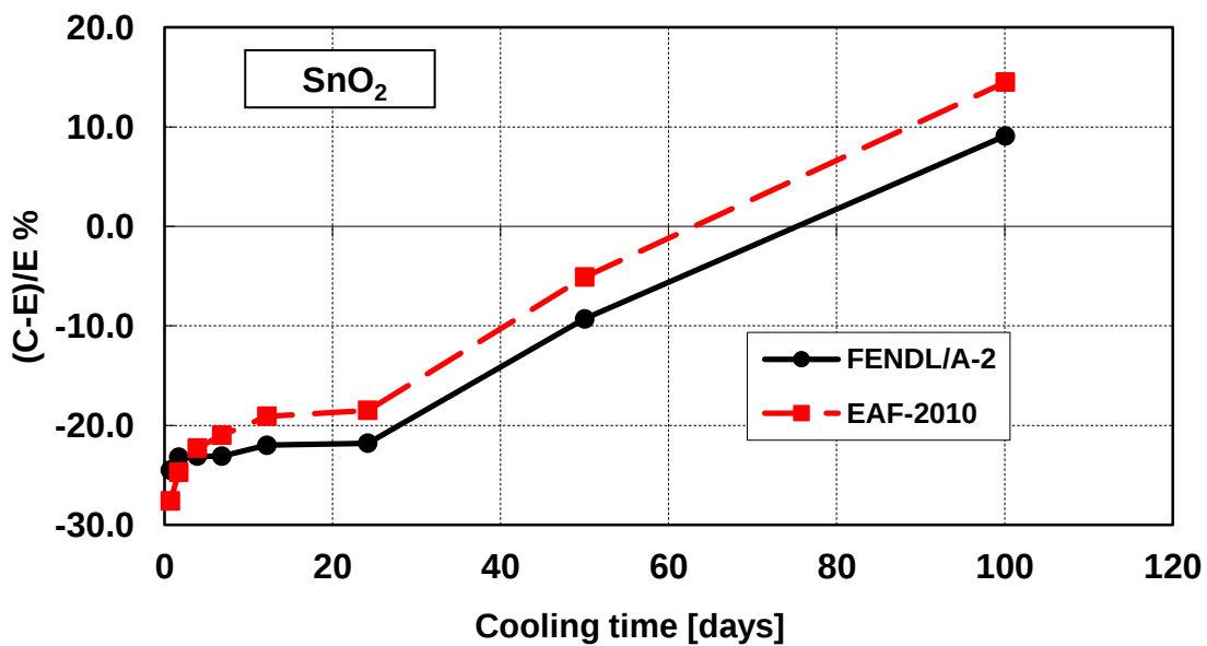
Figure 44 – Decay heat vs. cooling time of Tin Dioxide sample irradiated for 7 hours. Comparison of calculation with experiment (C-E)/E %.
