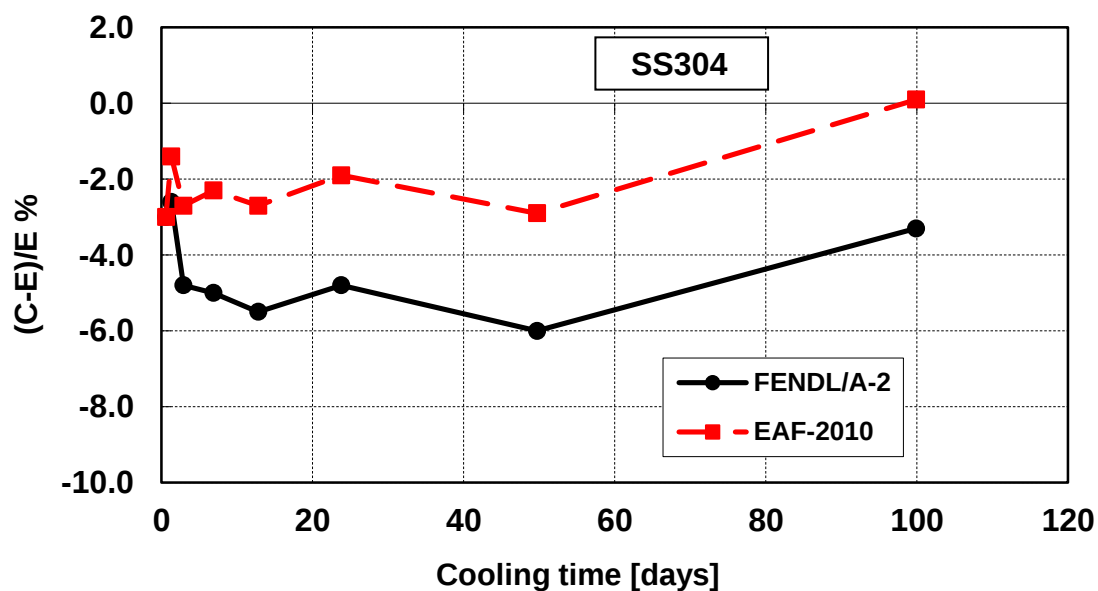
Figure 48 – Decay heat vs. cooling time of Stainless Steel SS304 sample irradiated for 7 hours. Comparison of calculation with experiment (C-E)/E %.
