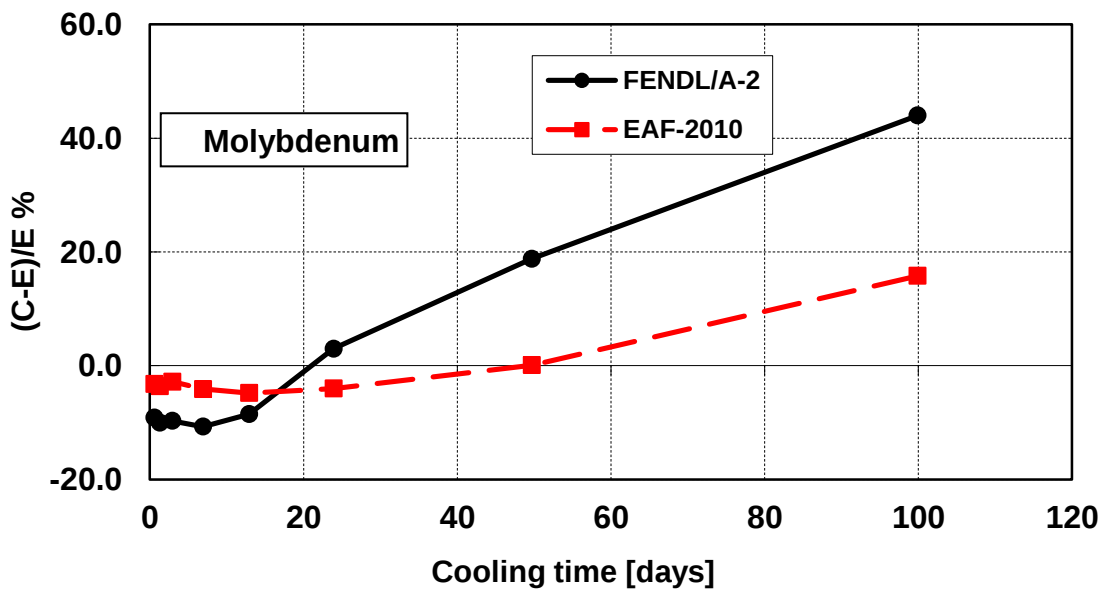
Figure 27 – Decay heat vs. cooling time of Molybdenum sample irradiated for 7 hours. Comparison of calculation with experiment (C-E)/E %.
