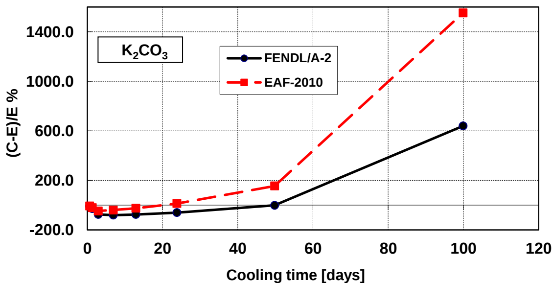
Figure 23 – Decay heat vs. cooling time of Potassium Carbonate sample irradiated for 7 hours. Comparison of calculation with experiment (C-E)/E %.
