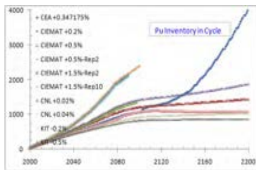
Fig. 2.2 Pu-Inventory. Exponential energy demand scenarios.
