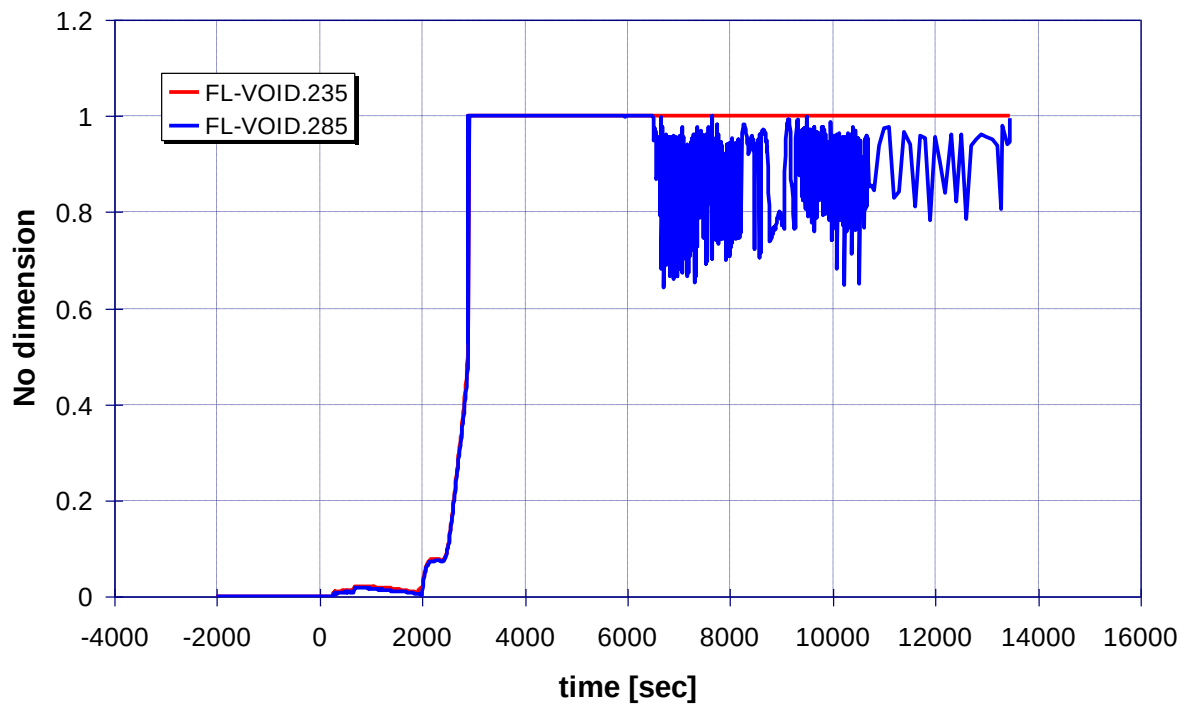
Figure 3.24: Sensitivity case A - Main pumps void fraction
