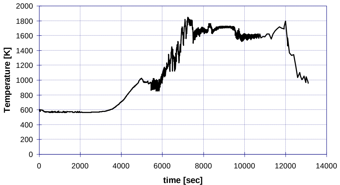
Figure 3.13: Reference case - Hot leg A temperature
