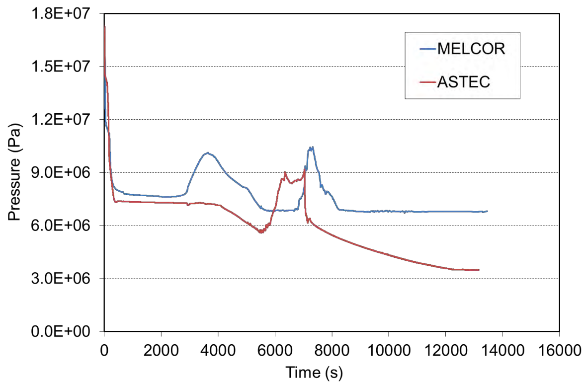
Figure 5.13: Pressurizer pressure
