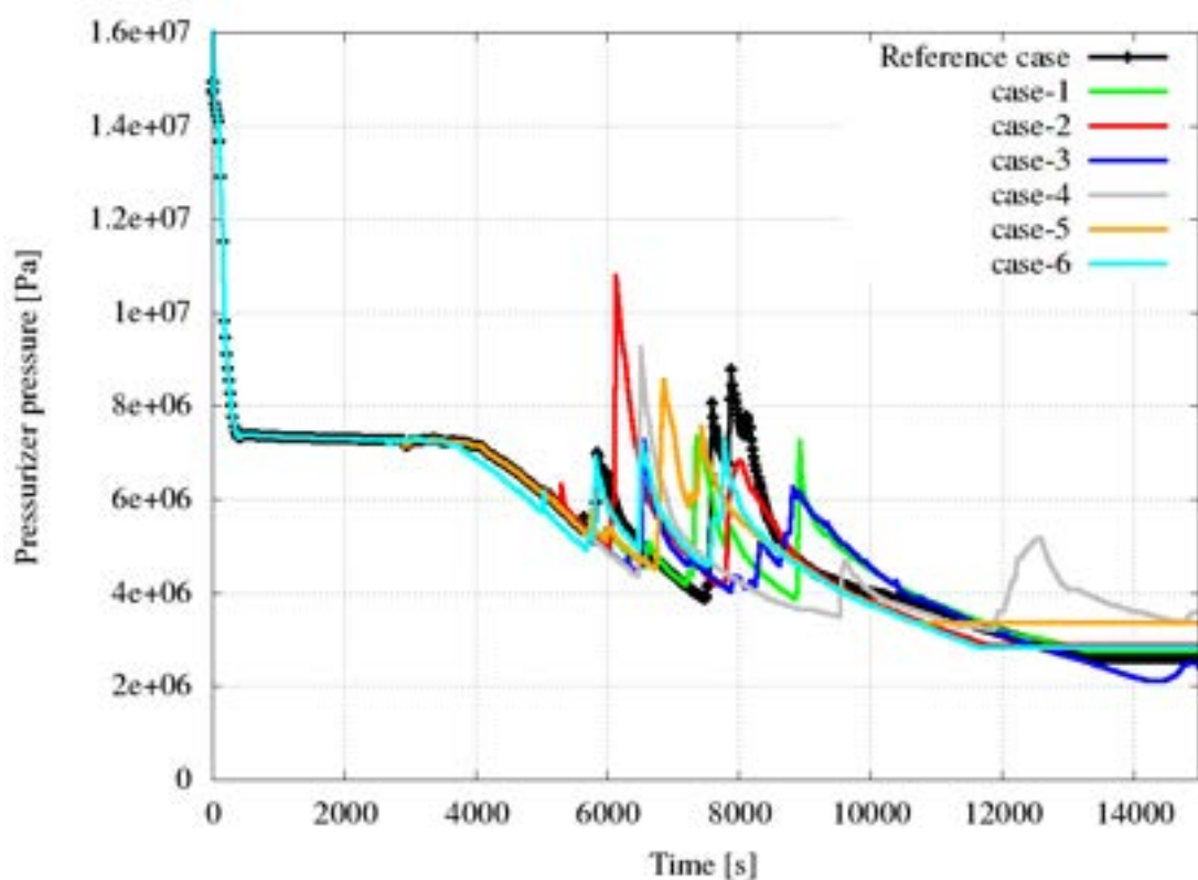
Figure 4.6: Pressurizer pressure
