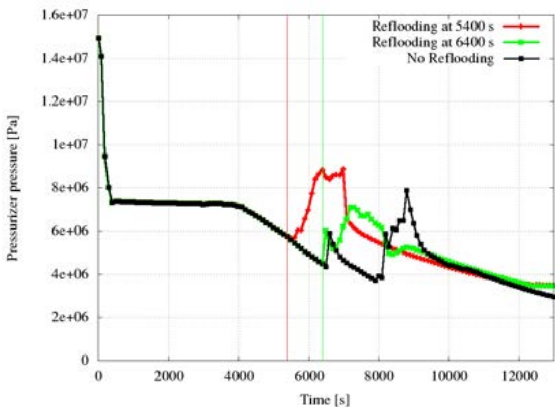
Figure 4.14: Pressurizer pressure
