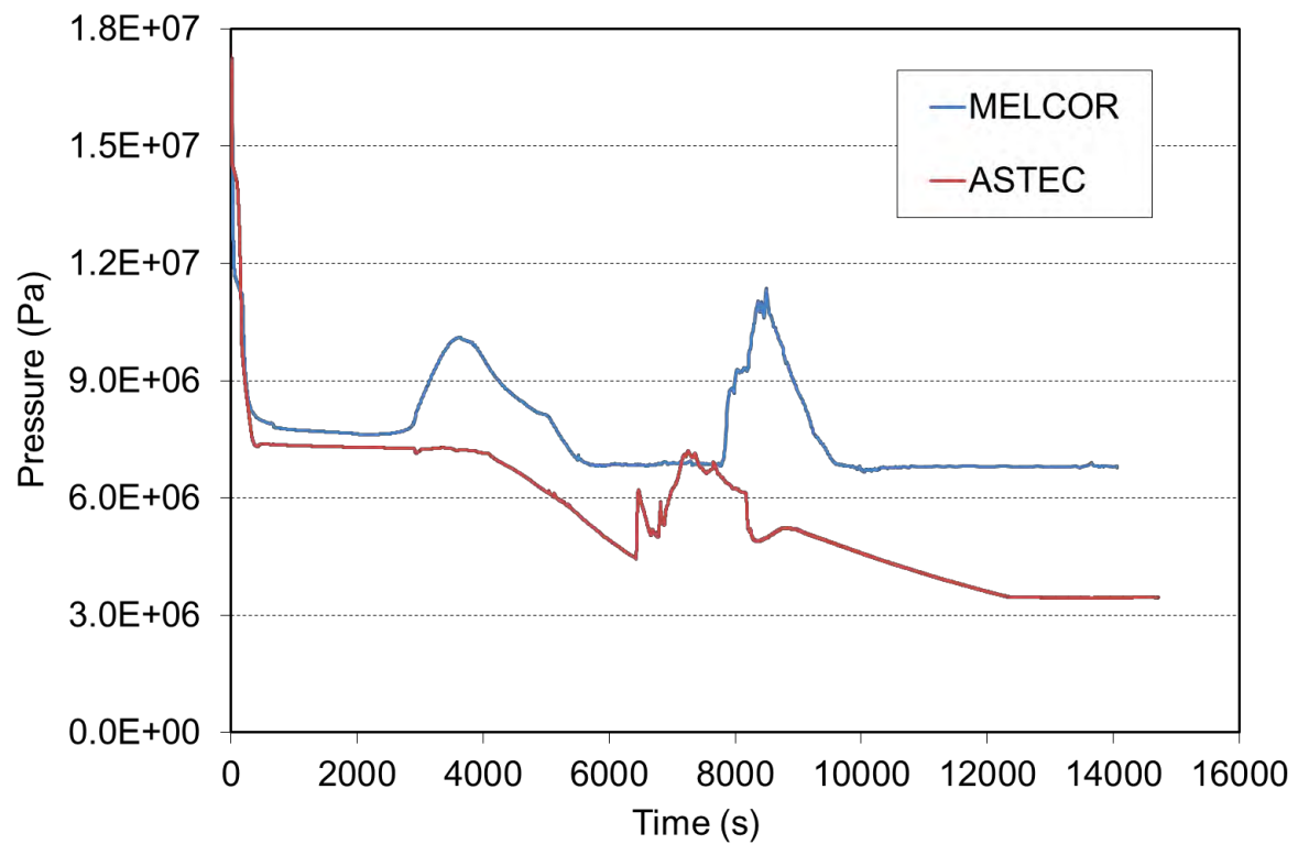
Figure 5.21: Pressurizer pressure
