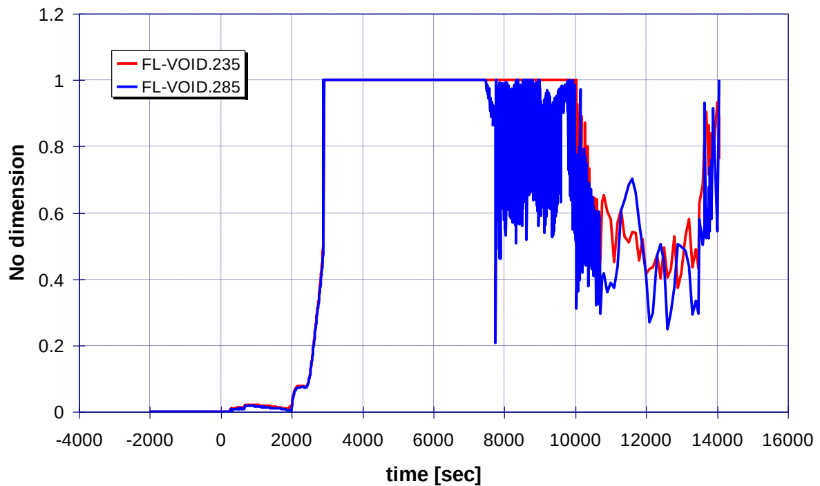
Figure 3.41: Sensitivity case B - Main pumps void fraction
