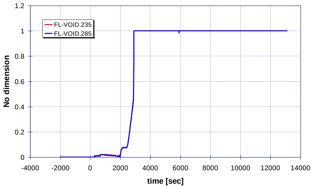
Figure 3.6: Reference case - Main pumps void fraction
