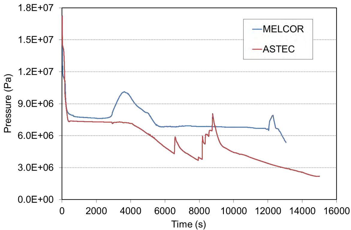
Figure 5.3: Pressurizer pressure
