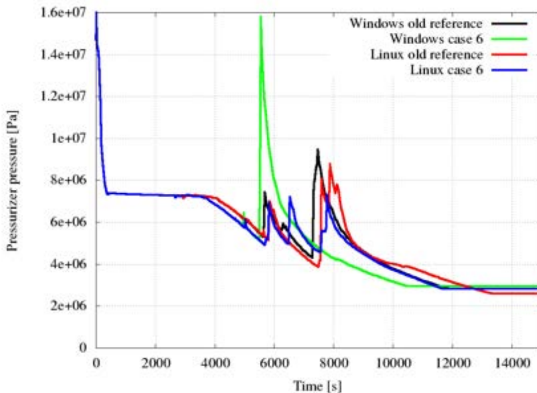
Figure 4.24: Pressurizer pressure
