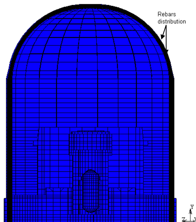
Figure 7. Containment model
