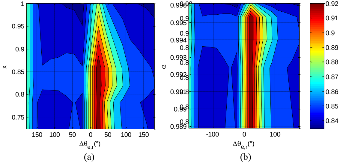
Fig. 24: S_{e,r} = f(\Delta\theta_{e,r}, x) e S_{e,r} = f(\Delta\theta_{e,r}, \alpha) per prove dinamiche
