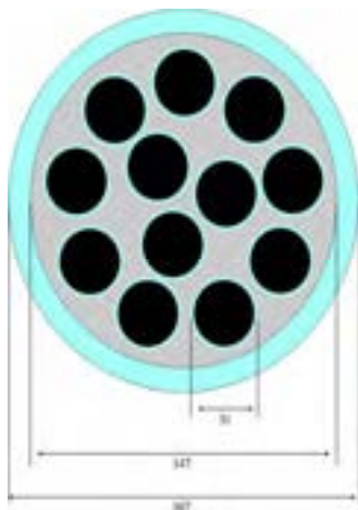
Figure 3 Safety rods scheme. To notice the 12 absorbing pins.
