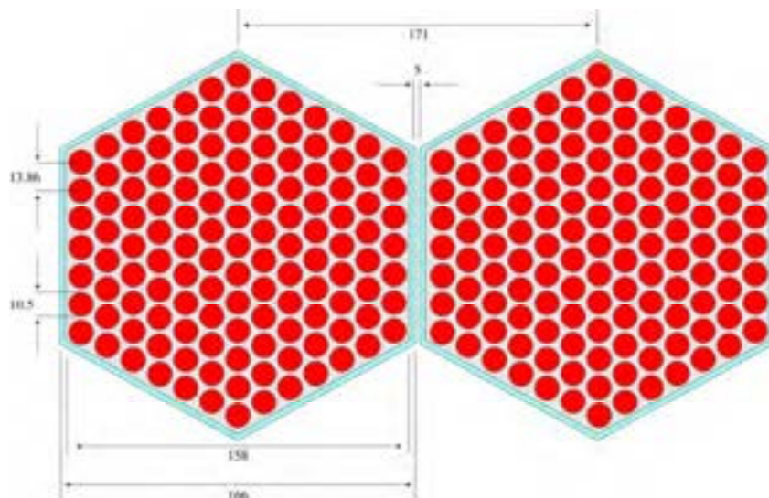
Figure 2 Fuel Assembly Scheme.
