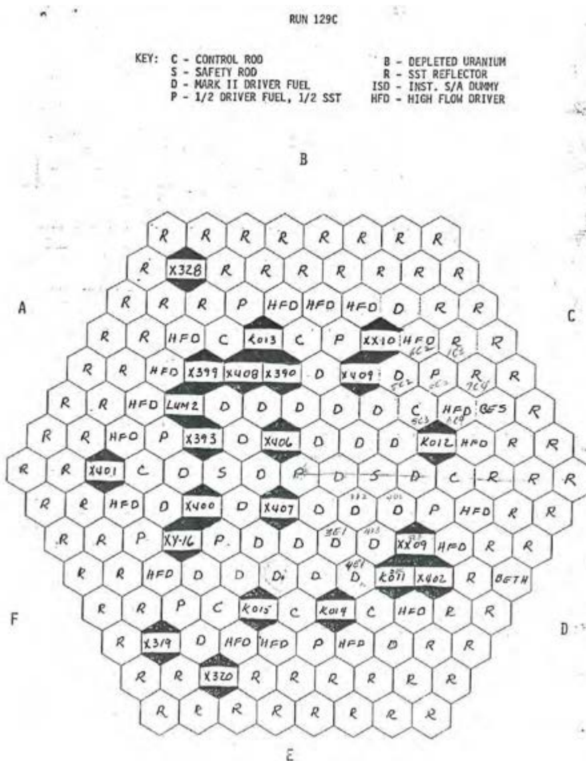
Fig. 4. SHRT-17 Core Loading Pattern (First 8 rings).
