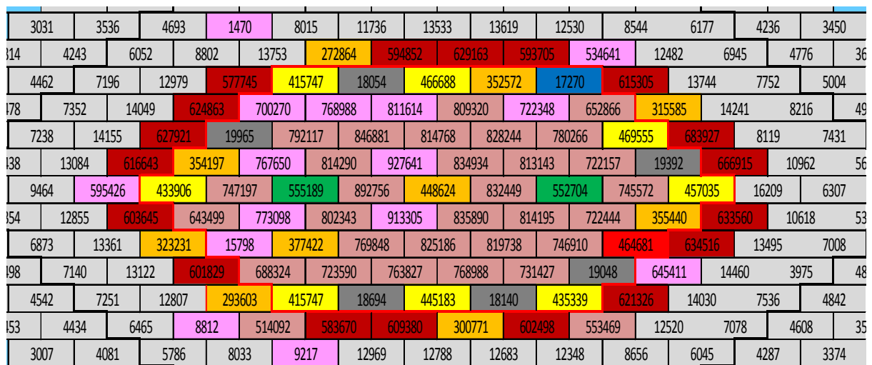
Fig. 6. Zoom of power distribution in the EBR-II assemblies on the zone of interest (first seven rings).
