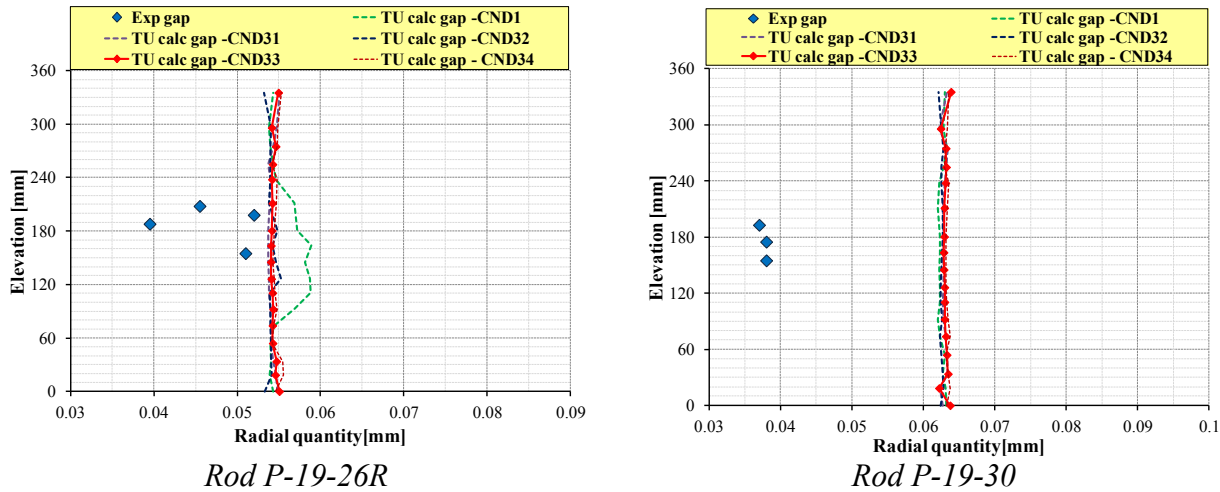
Fig. B. 16 – HEDL P-19, influence of fuel conductivity on gap size, rods #11, 14.
