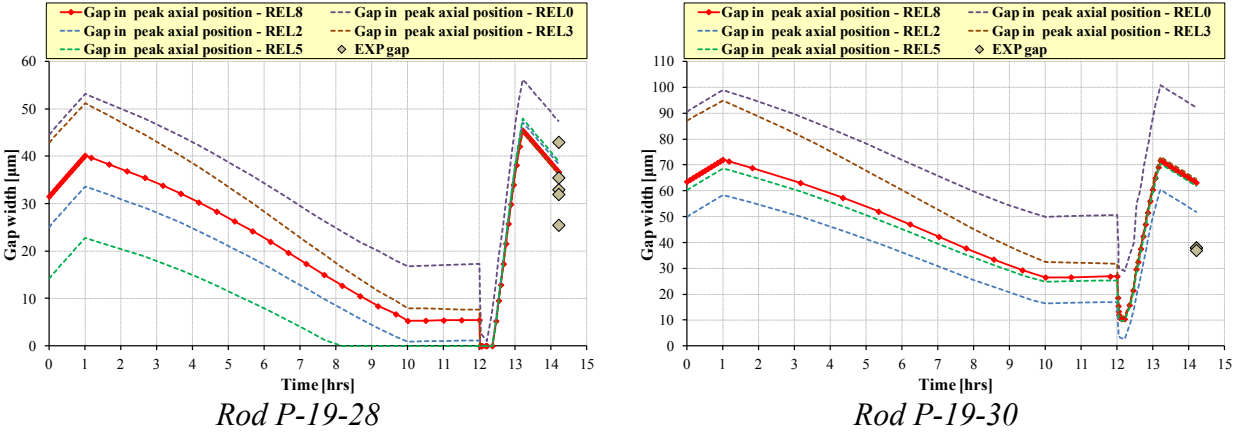
Fig. A. 7 – HEDL P-19, influence of relocation on gap trend, rods #13, 14.
