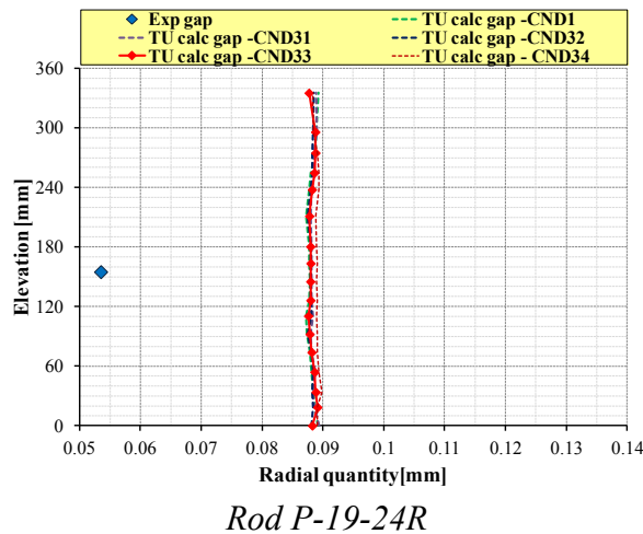
Fig. B. 15 – HEDL P-19, influence of fuel conductivity on gap size, rods #9, 10.
