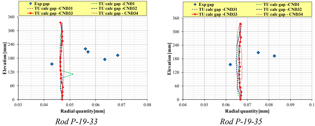
Fig. B. 17 – HEDL P-19, influence of fuel conductivity on gap size, rods #15, 16.
