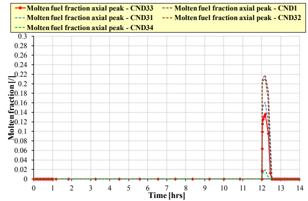
Fig. B. 2 – HEDL P-19, influence of fuel conductivity on the fuel melting fraction in peak axial section, rod P-19-2.
