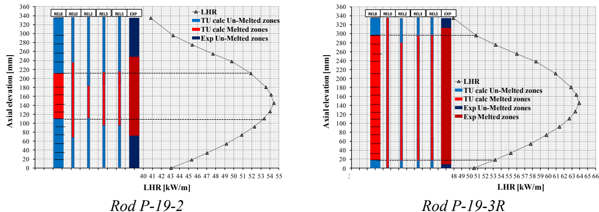
Fig. A. 9 – HEDL P-19, influence of the relocation model on fuel melting, rods #1, 2.
