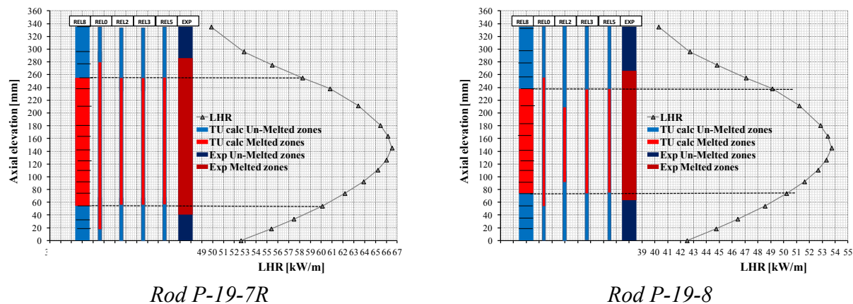
Fig. A. 11 – HEDL P-19, influence of the relocation model on fuel melting, rods #5, 6.
