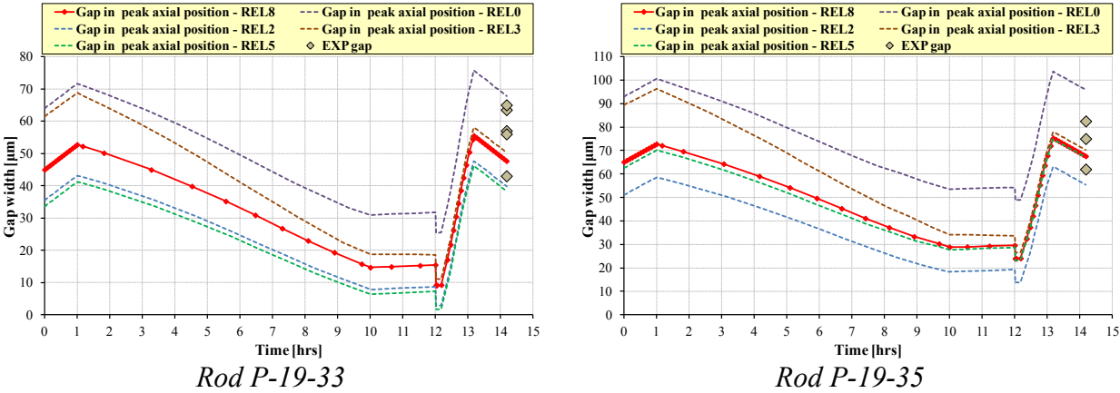
Fig. A. 8 – HEDL P-19, influence of relocation on gap trend, rods #15, 16.
