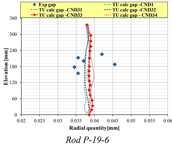
Fig. B. 14 – HEDL P-19, influence of fuel conductivity on gap size, rods #4, 6.
