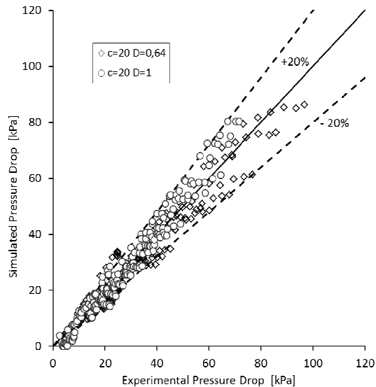
Fig. 13 – Experimental versus simulated two-phase pressure drops by RELAP5 code modified with C = 20
