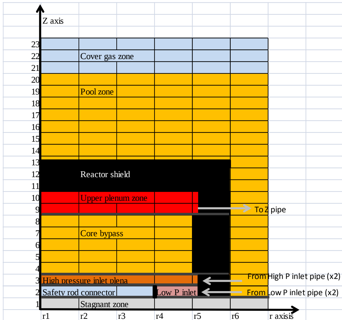
Fig. 25 - EBR-II nodalization: schematizzation of 3D component in the plane R, Z.
