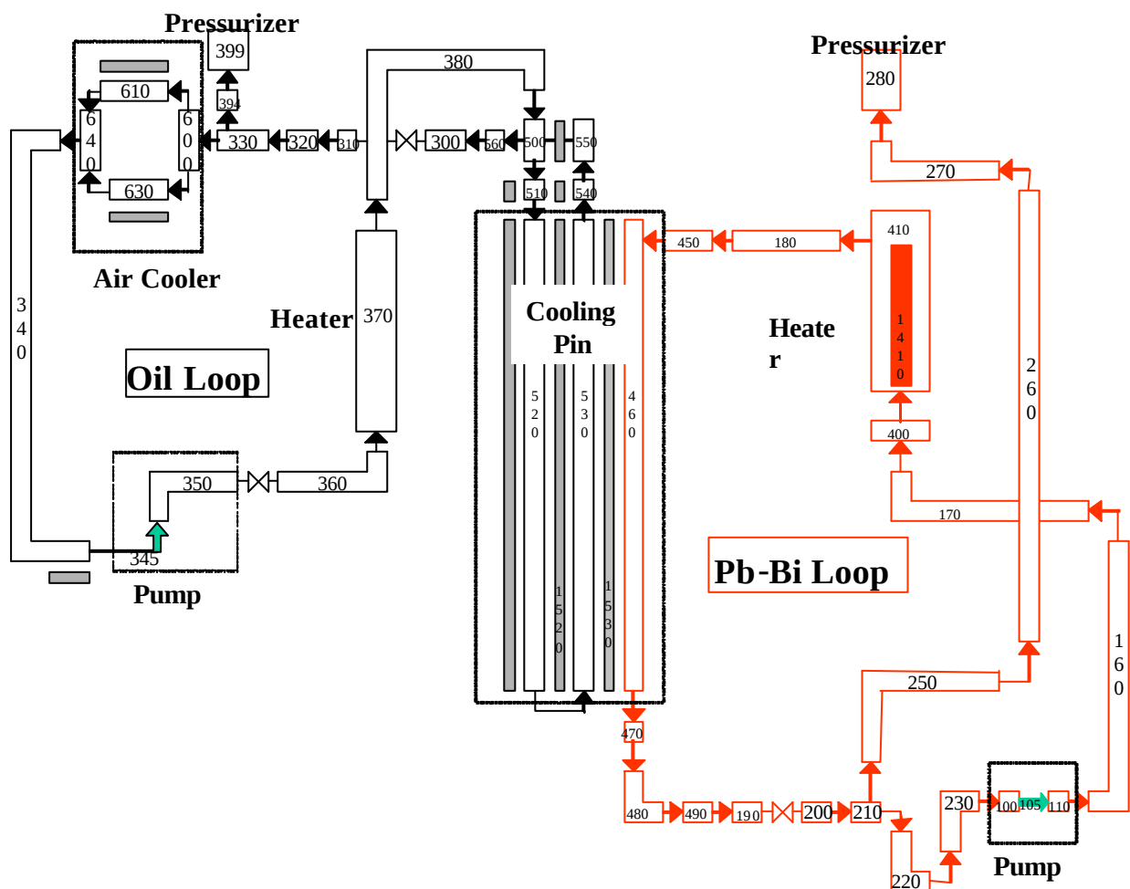
Fig. 3: RELAP nodalization
