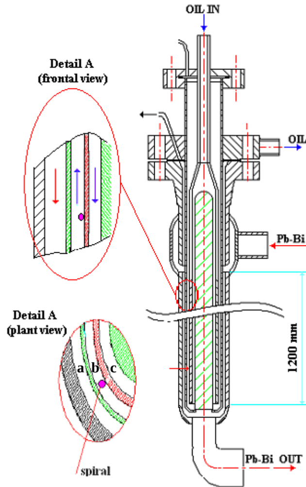
Fig. 1: Cooling pin
