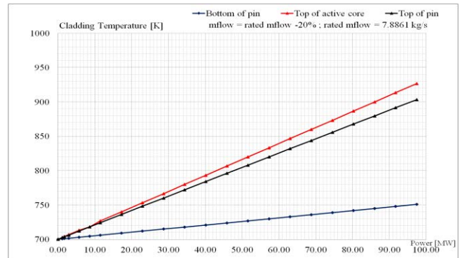
(b) Cladding temperature at different elevations vs power at nominal mass flow rate minus 20%
