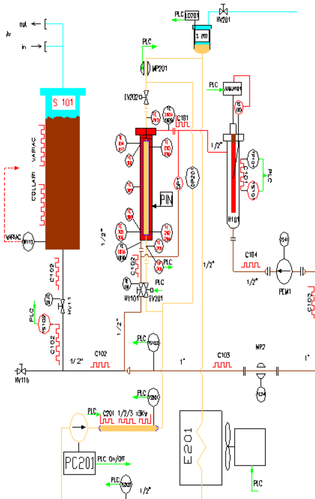
Fig. 1: CHEOPE facility flow plan
