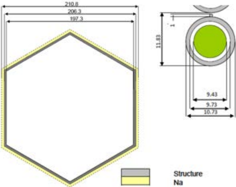
Fig. 4 – CP-ESFR: hexagonal wrapper tube and fuel pin
