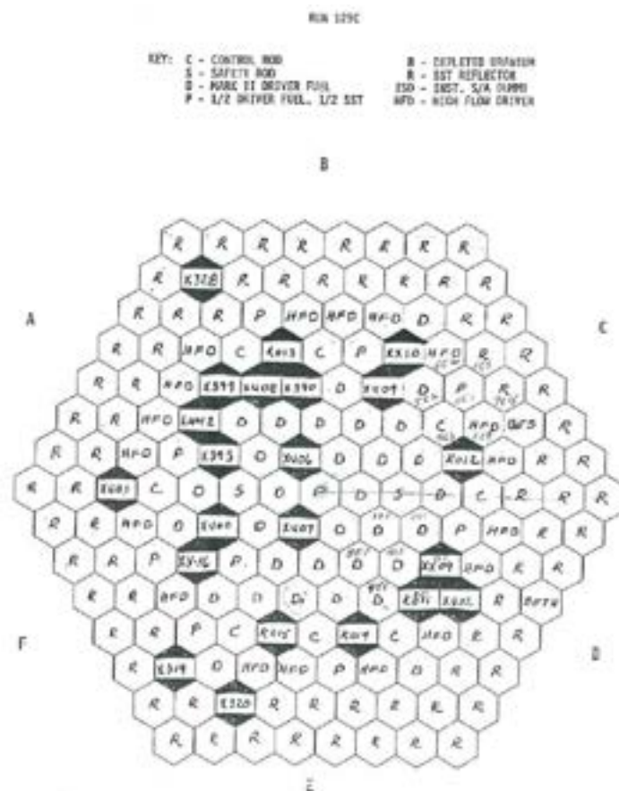
Fig. 17 - EBR-II SHRT-17 Core Loading Pattern (First 8 Rows)
