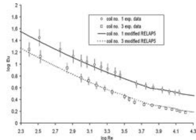
Fig. 1. Ali's (2001) experiments relevant to log Euler numbers for coil no. 1 and coil no. 3: effect of modified RELAP5 smoothing procedure. The bars represent \pm 10\% errors.
