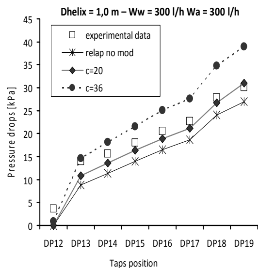
Fig. 8 - Pressure drops along the pipe D = 1.0 m for water mass flow rate of 300 l/h and air mass flow rate of 300 l/h
