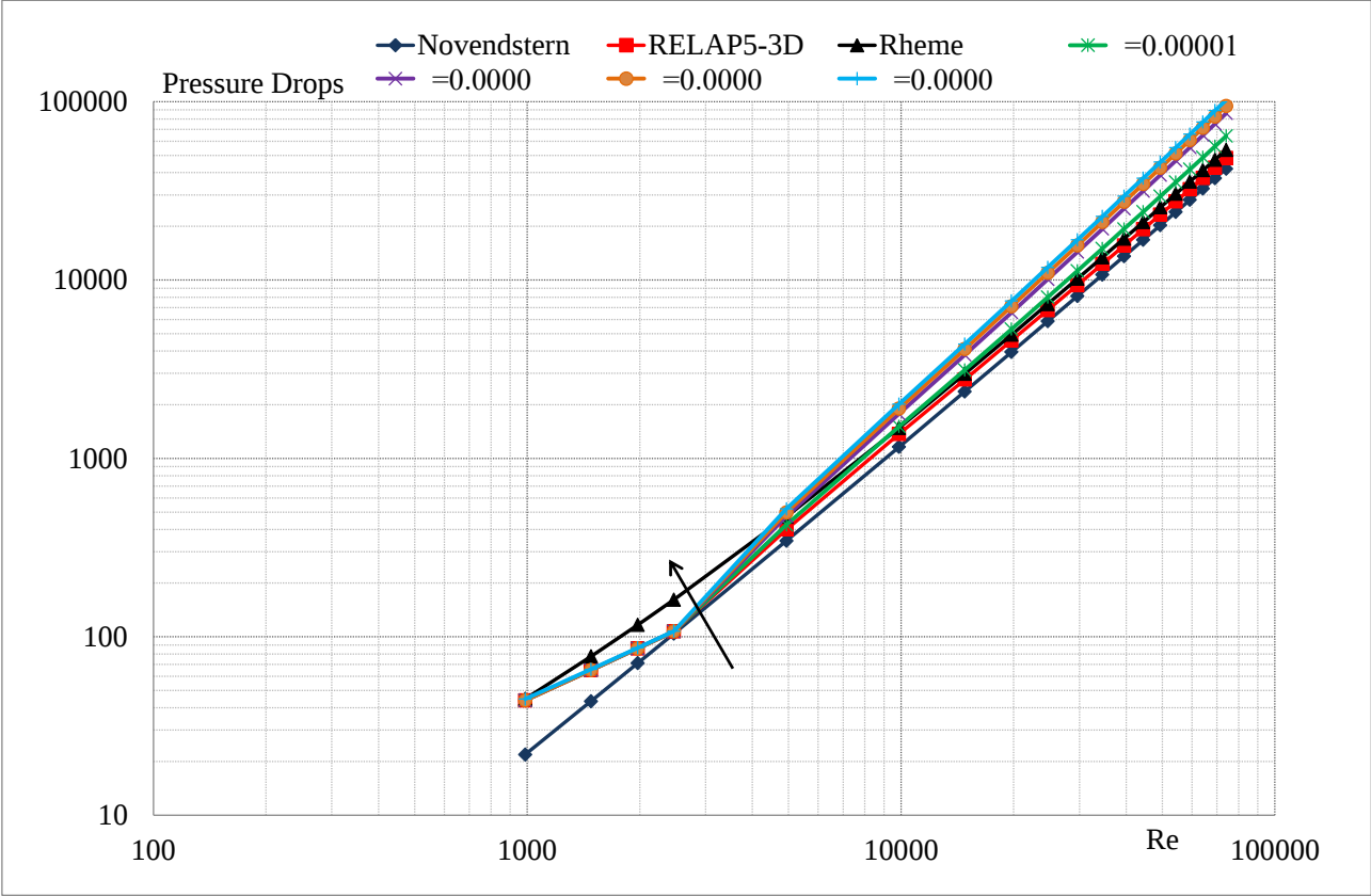
Fig. 30 – EBR-II nodalization. MARK II dynamic pressure drop in wire wrapped fuel bundle
