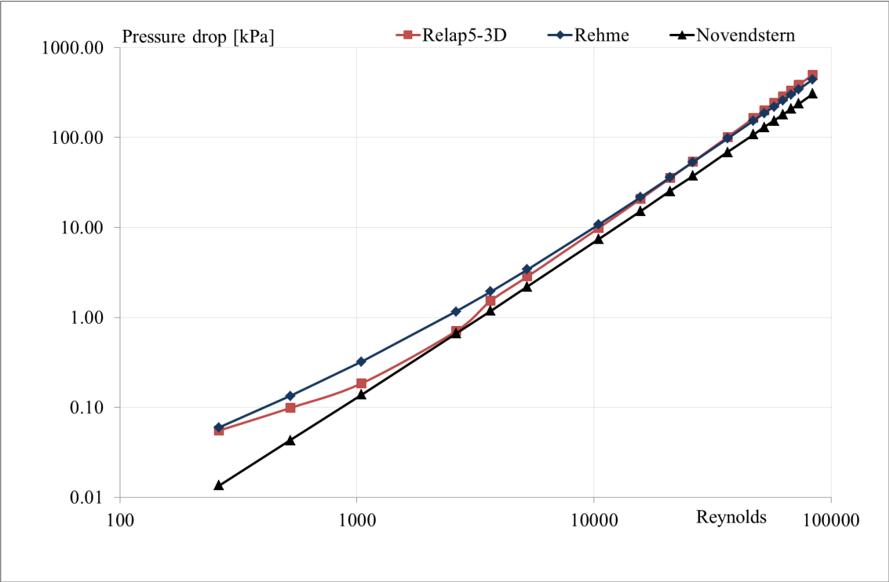
Fig. 14 – CP-ESFR fuel assembly performances: friction losses in wire wrapped fuel assembly vs. experimental based empirical correlations.
