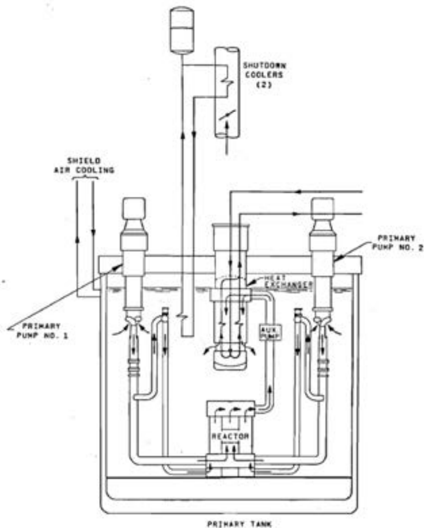
Fig. 15 - EBR-II Primary Tank Sodium Flow Paths.
