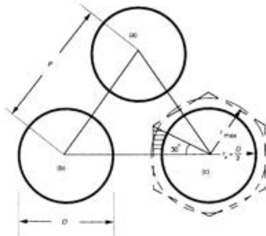
Fig. 3.1. On the left: equivalent annulus around a rod in a triangular array. Cross-hatched area represents an elementary coolant flow section; circle of radius r_{\max} represents the equivalent annulus with equal flow area. On the right: product of laminar friction factors and N_{Re} for parallel fully developed laminar flow in a triangular array rod bundle [6].
