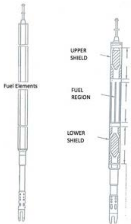
Fig. 19 - EBR-II MARK-II AI Subassembly Configuration.
