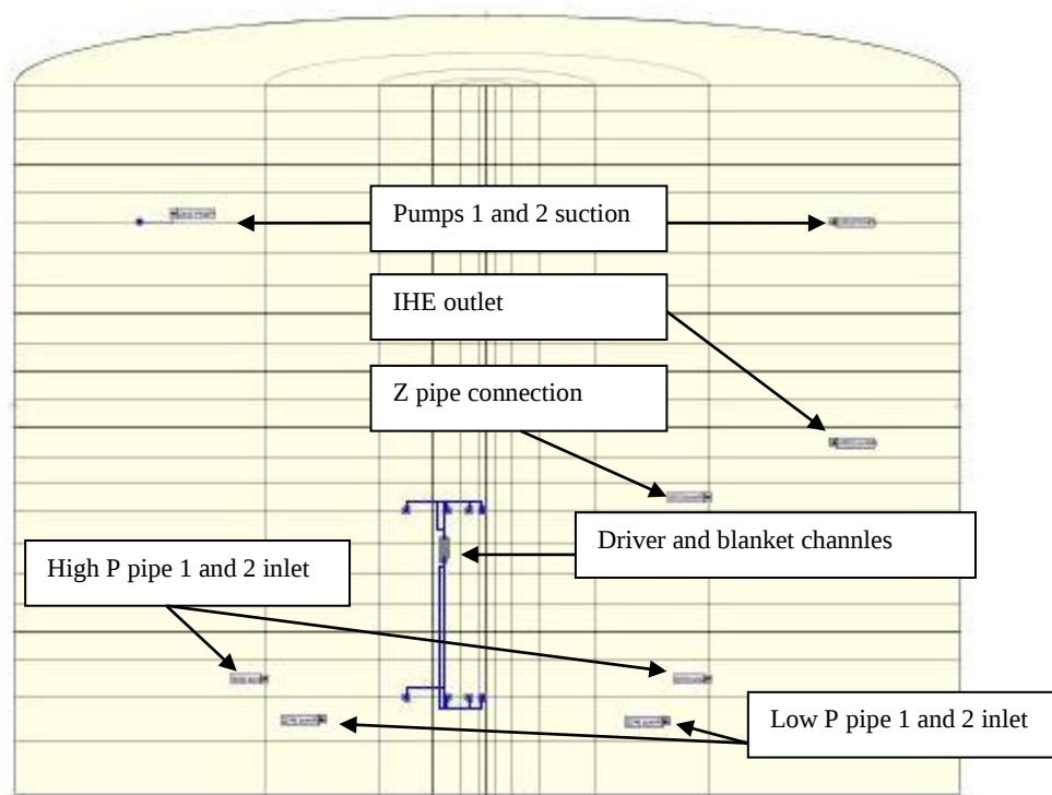
Fig. 26 - EBR-II nodalization: schematization of the 3D component with the 1D componenet connections.
