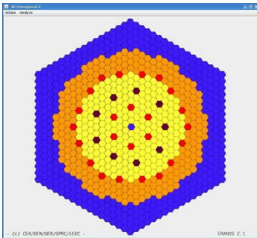
Fig. 2 – CP-ESFR: radial cross-section of the SFR core with oxide fuel
