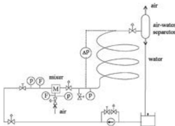
Fig. 5. Schematic of the experimental facility at the Polytechnic of Torino laboratory (Bertani et al., 2007, 2008).
