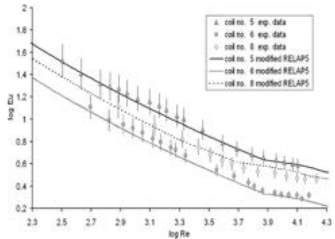
Fig. 2. Ali's (2001) experiments relevant to log Euler numbers for coil no. 5, coil no. 6 and coil no. 8: effect of modified RELAP5 smoothing procedure. The bars represent \pm 10\% errors.
