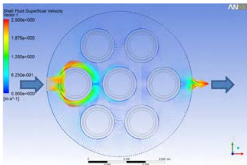
Figure 8 Water velocity vector in the middle z plane for case 15.
