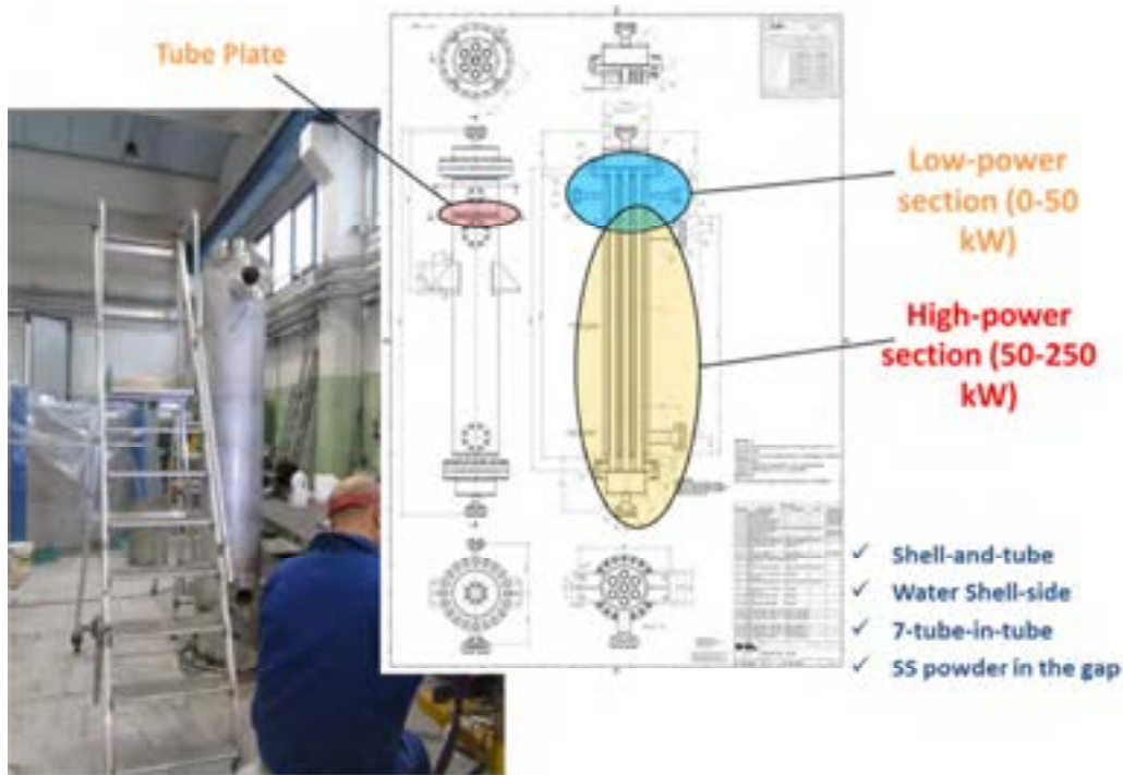
Figure 3 Picture of the NACIE-UP HX with some schematic indication.
