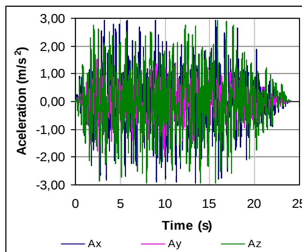
Figure 8- Seismic ATHs with PGA = 0.3 g.
