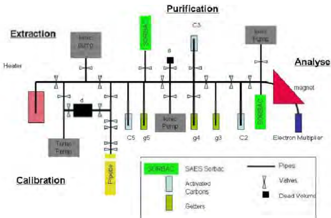
Figure 1: experimental device for characterising traces of rare gases
