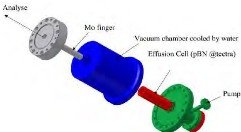
Figure 2: Extraction furnace
