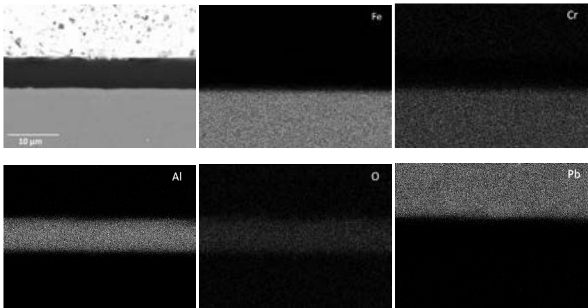
Figure 2. Cross-sectional SEM micrograph of the coated surface of a steel sample after exposure to HLM at 600°C for 500 hours (a). The coating is compact and reproduces the roughness of the substrate. No defects can be found throughout the thickness and no signs of corrosion are observed, as confirmed by Energy Dispersive X-Ray Spectroscopy (EDX) maps for Fe (b), Cr (c), Al (d), O (e) and Pb (f).
