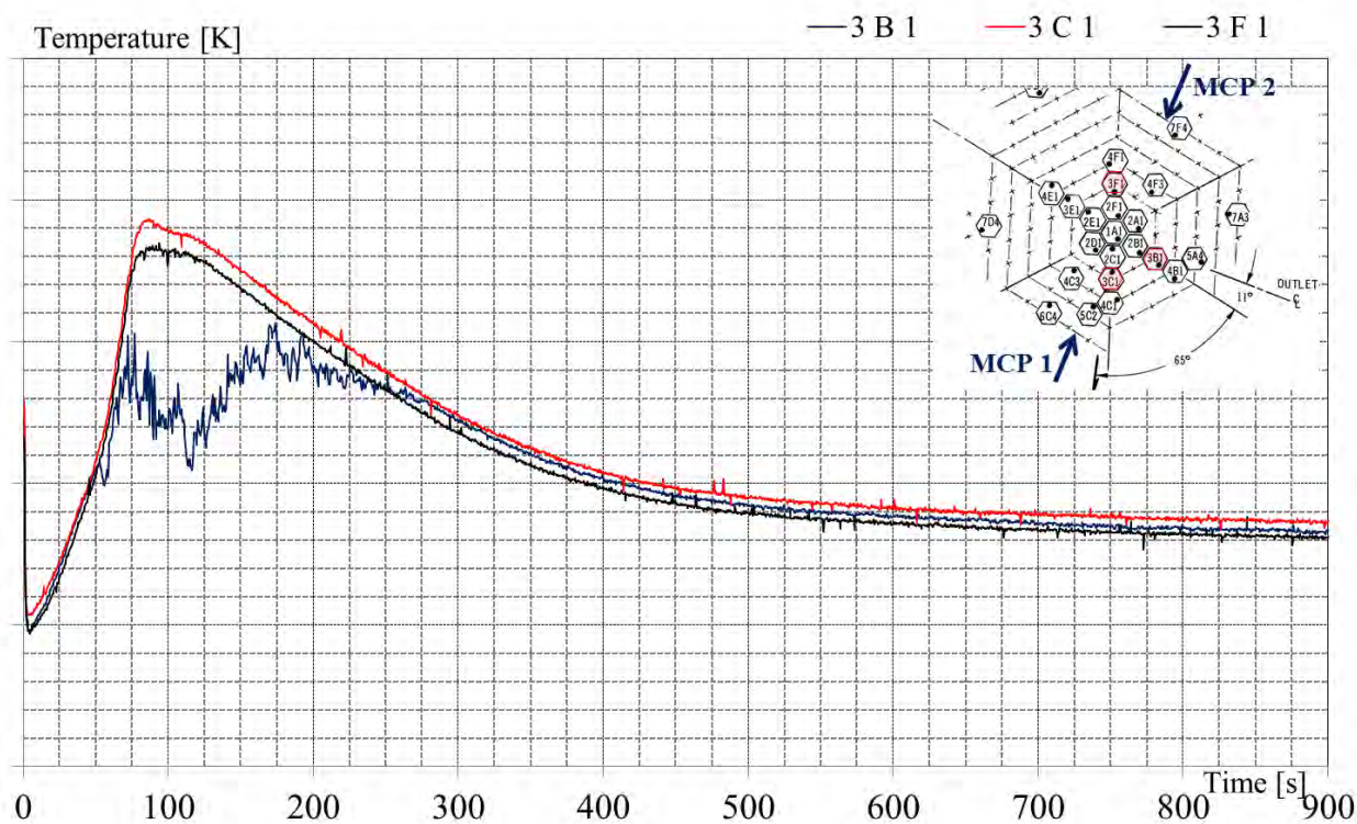
Fig. 42 – EBR-II, SHRT-17: Subassembly Outlet Temperature (Row 3).
