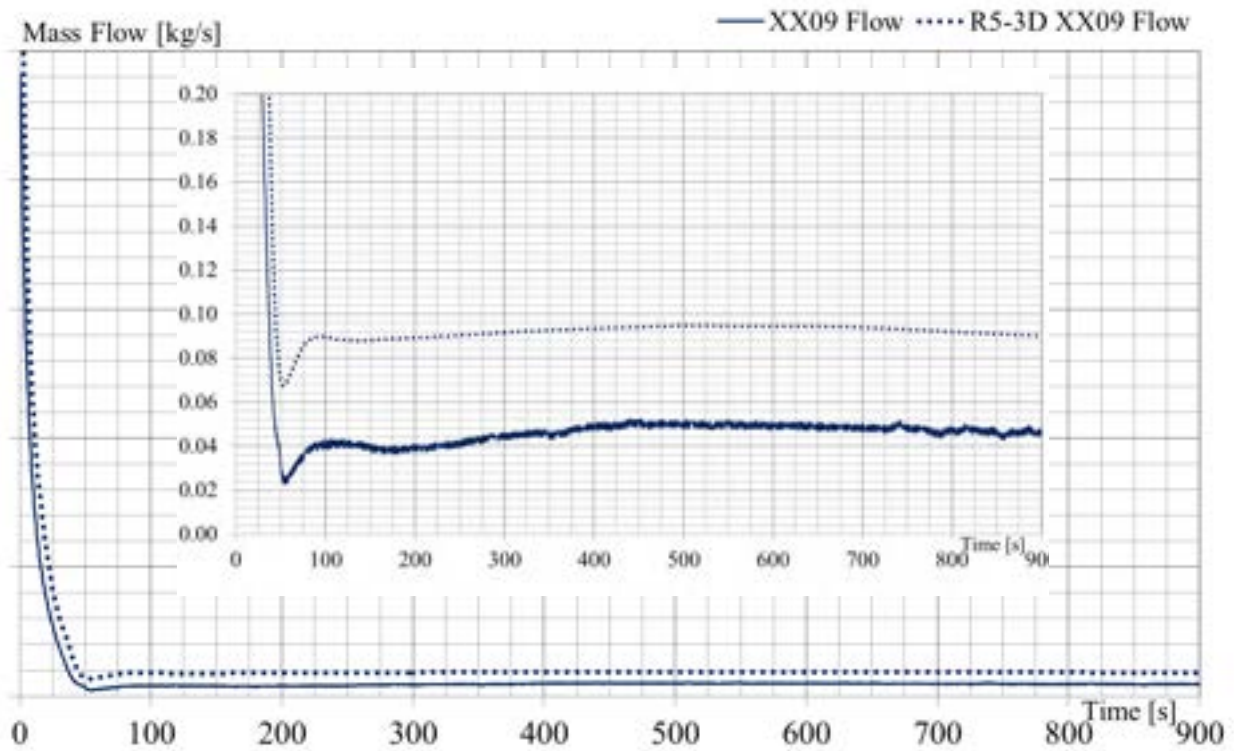
Fig. 65 – EBR-II SHRT-17, RELAP5-3D ® : XX09 Mass Flow Rate.
