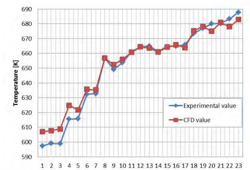
Fig. 94 – Comparison of duct (wrap internal) temperature predictions at different heights with TEST SERIES 4-RUN105 experimental results.
