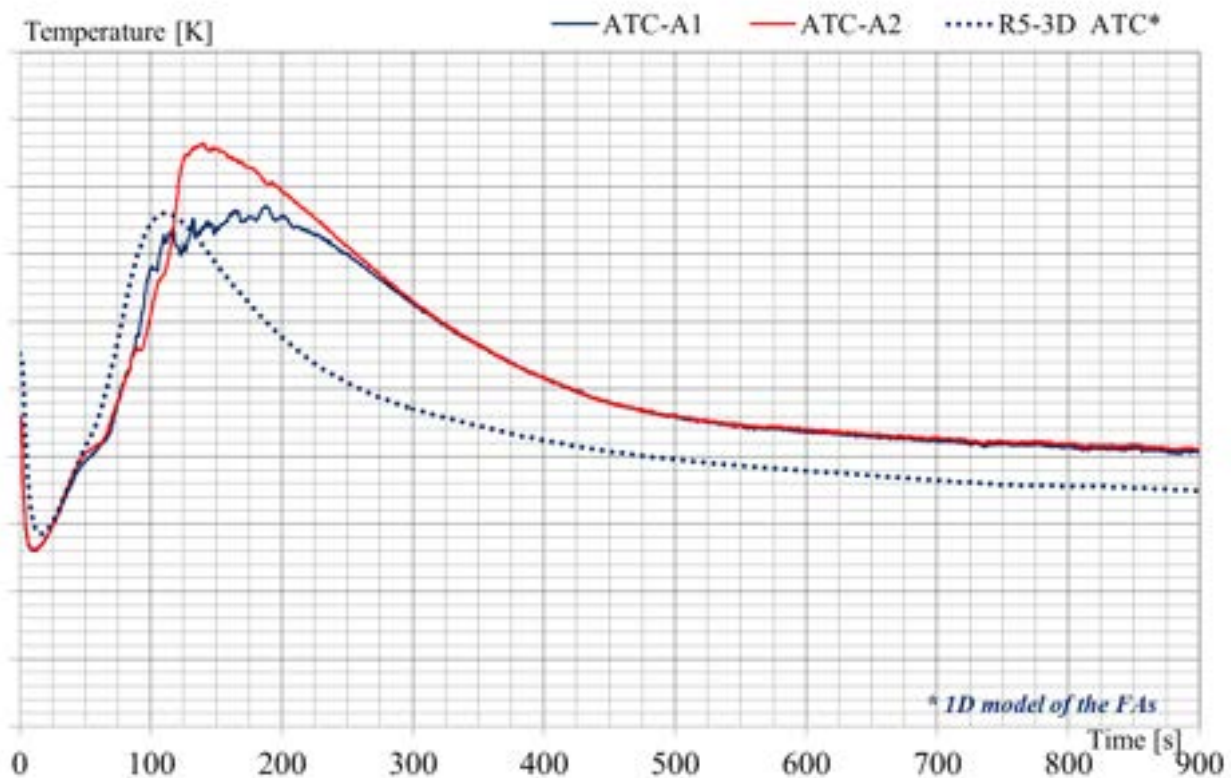
Fig. 79 – EBR-II SHRT-17, RELAP5-3D®: XX10 Thimble Annulus Temperature.
