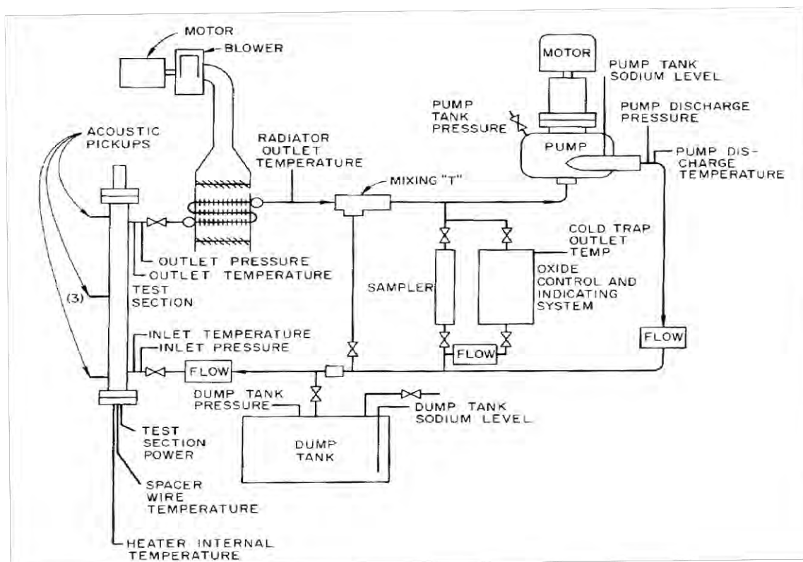
Fig. 88 – Fuel Failure Mockup test facility at ORNL.
