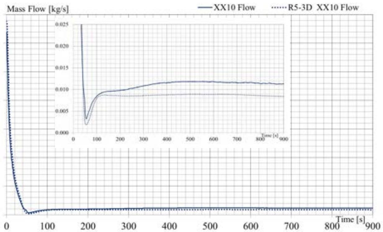
Fig. 66 – EBR-II SHRT-17, RELAP5-3D ® : XX10 Mass Flow Rate.
