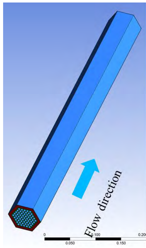
Fig. 95 – Overview of the CFD model for the XX09/XX10 FA of the EBR II reactor.
