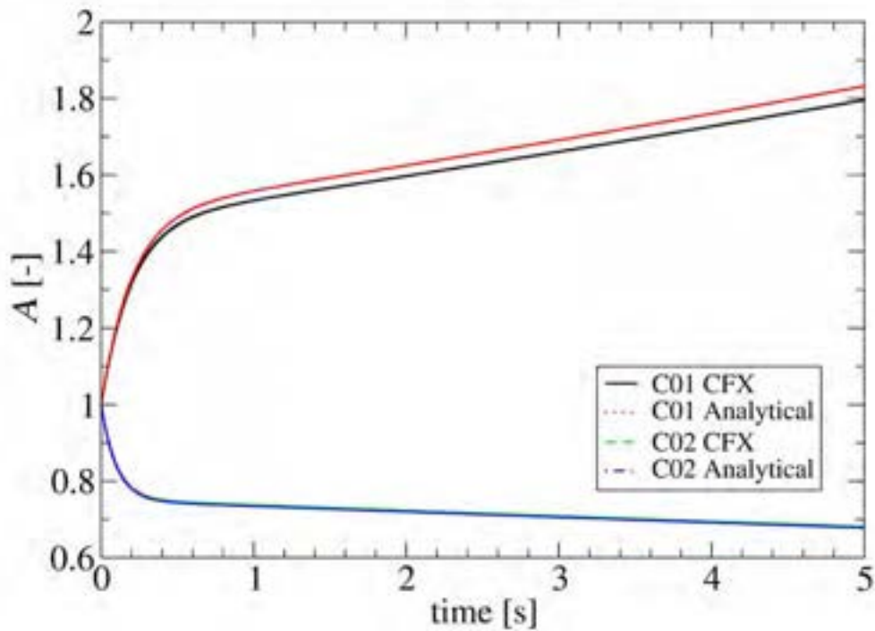
Figure 41 Comparison between CFX and analytical solutions for C01 and C02.
