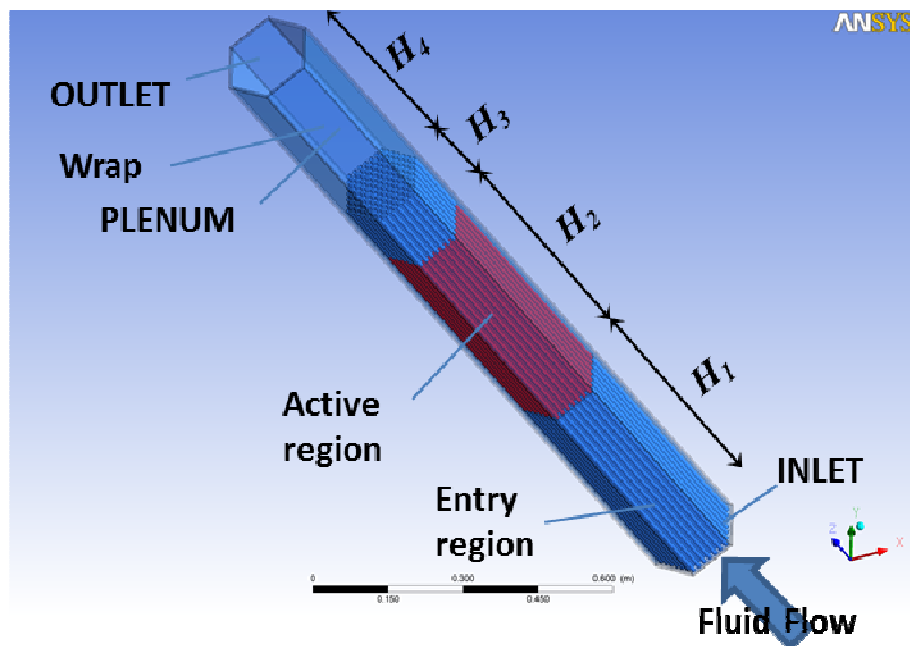
Figure 5 Computational domain for the CFD: perspective view.
