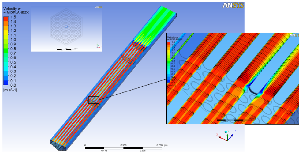
Figure 19 Streamwise velocity contours in the ZX midplane for case 1.
