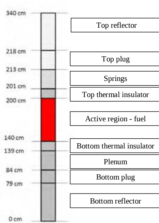
Figure 39 ERANOS model for neutronic calculation for cell code ECCO.
