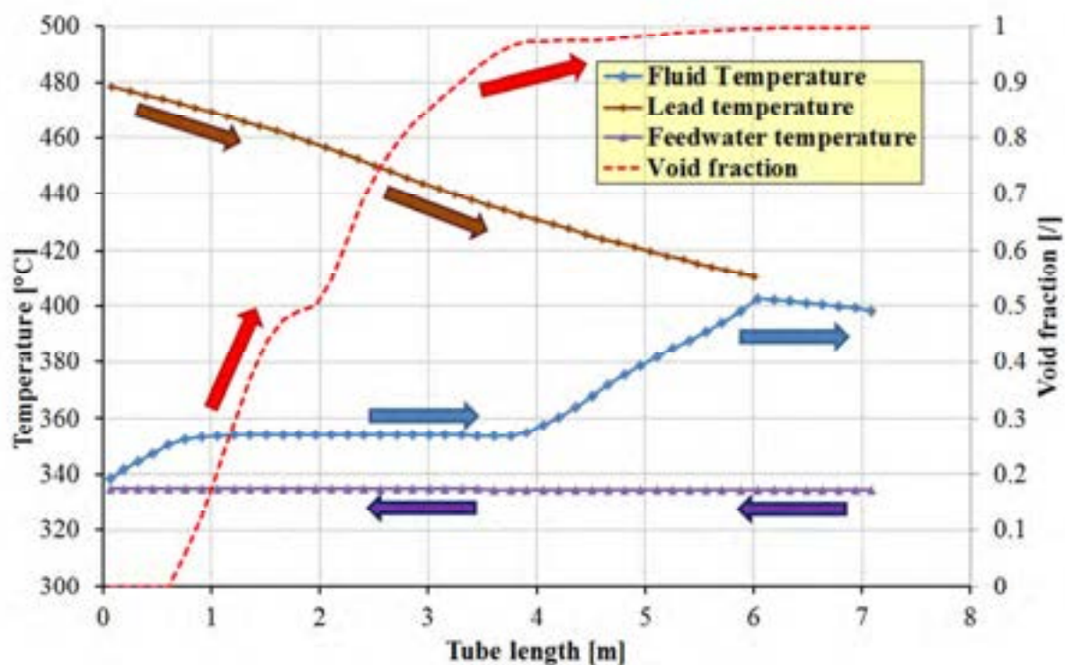
Fig. 23 – HERO-CIRCE SGBT unit vs RELAP-5 main TH parameters.
