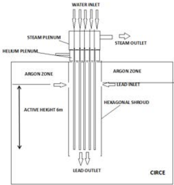
Schematic layout
