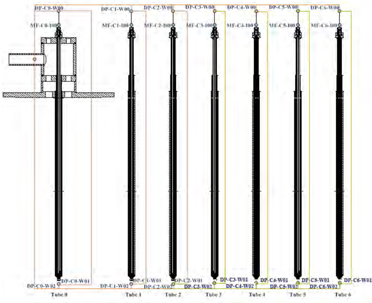
Fig. 20 – HERO-CIRCE SGBT unit instrumentation: pressure transducers and mass-flow meters in the steam-water side.
