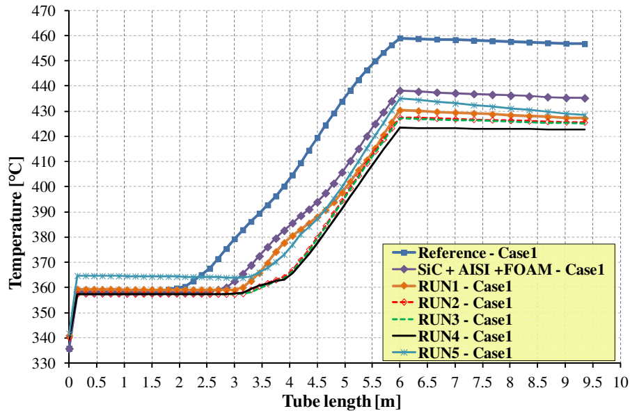
Fig. 5 – HERO-CIRCE SGBT unit vs. RELAP5, investigations on tube geometry, steam temperature, case 1.
