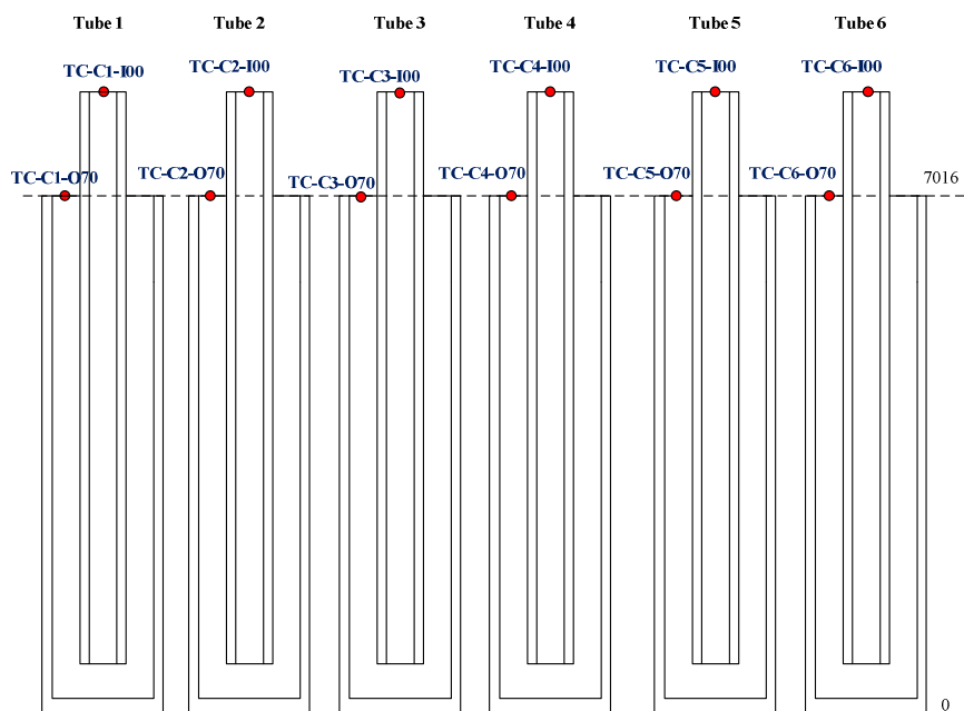
Fig. 17 – HERO-CIRCE SGBT unit instrumentation: TCs in tubes 1-2-3-4-5-6.
