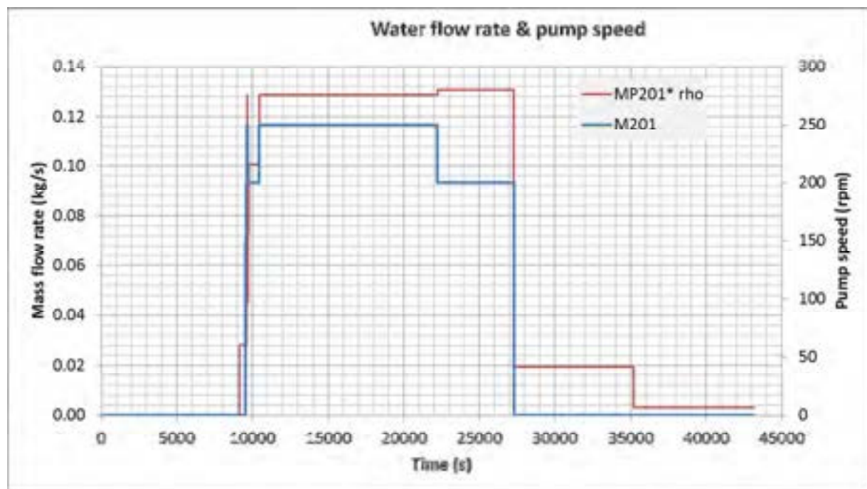
Figure 8 – Water flow rate and pump speed during test 301.
