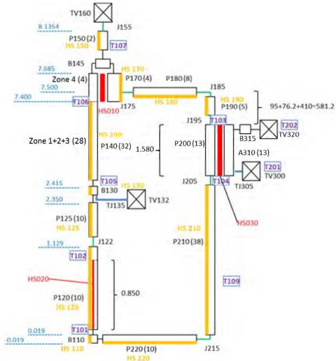
Figure 9 – Sketch of the 1D RELAP nodalization for NACIE loop.
