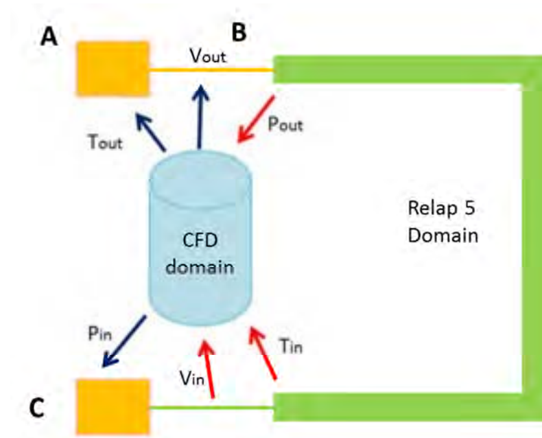
Figure 25 – Simplified sketch of the coupling procedure.
