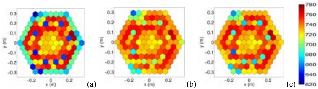
Fig. 8 Computed Na temperature (K) distribution at the outlet of the heated region: (a) FRENETIC, adiabatic HAS; (b) FRENETIC, coupled HAS; (c) RELAP5-3D©, coupled HAS.
