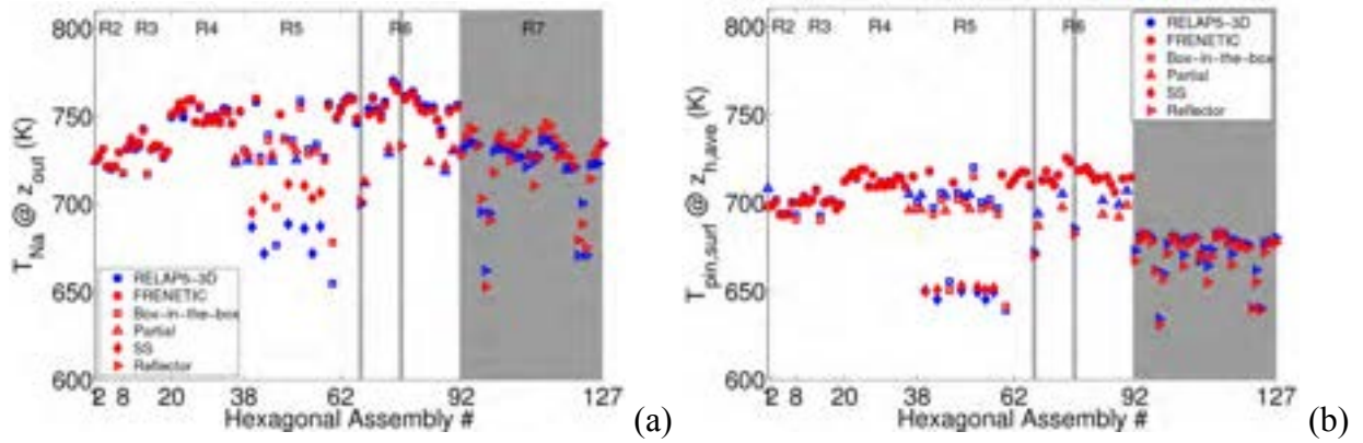
Fig. 9 Comparison between FRENETIC (red symbols) and RELAP5-3D© (blue symbols) at steady state, in the case of thermally coupled HAs: (a) T_{out} ; (b) average pin surface temperature at mid height of the heated region. Solid circles refer to all driver and experimental HAs.
