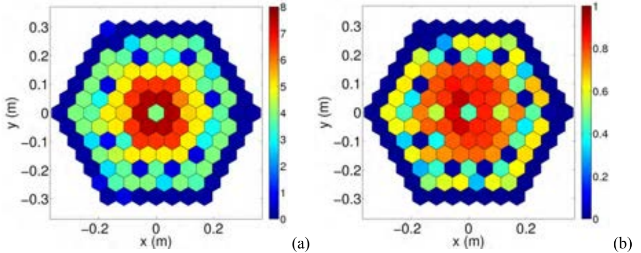
Fig. 6 (a) Distribution among HAs of the inlet mass flow rate (kg/s) computed by RELAP5-3D© and used as BC by FRENETIC. (b) Distribution among HAs of the input power (MW).
