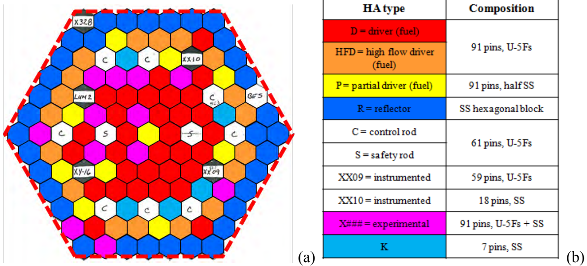
Fig. 4 (a) EBR-II core loading pattern. (b) Composition of the main HA types (BES, LUM 2 and XY-16 are SS HAs geometrically similar to the R, XX10 and XX09 HAs, respectively).
