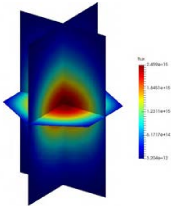
Fig. 74 – PHISICS 3D model: total flux.
