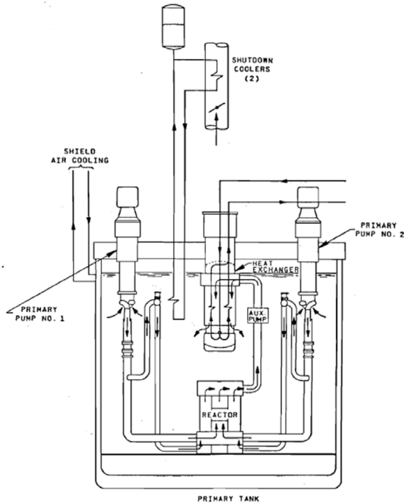
Fig. 2 – EBR-II Primary Tank Sodium Flow Paths.
