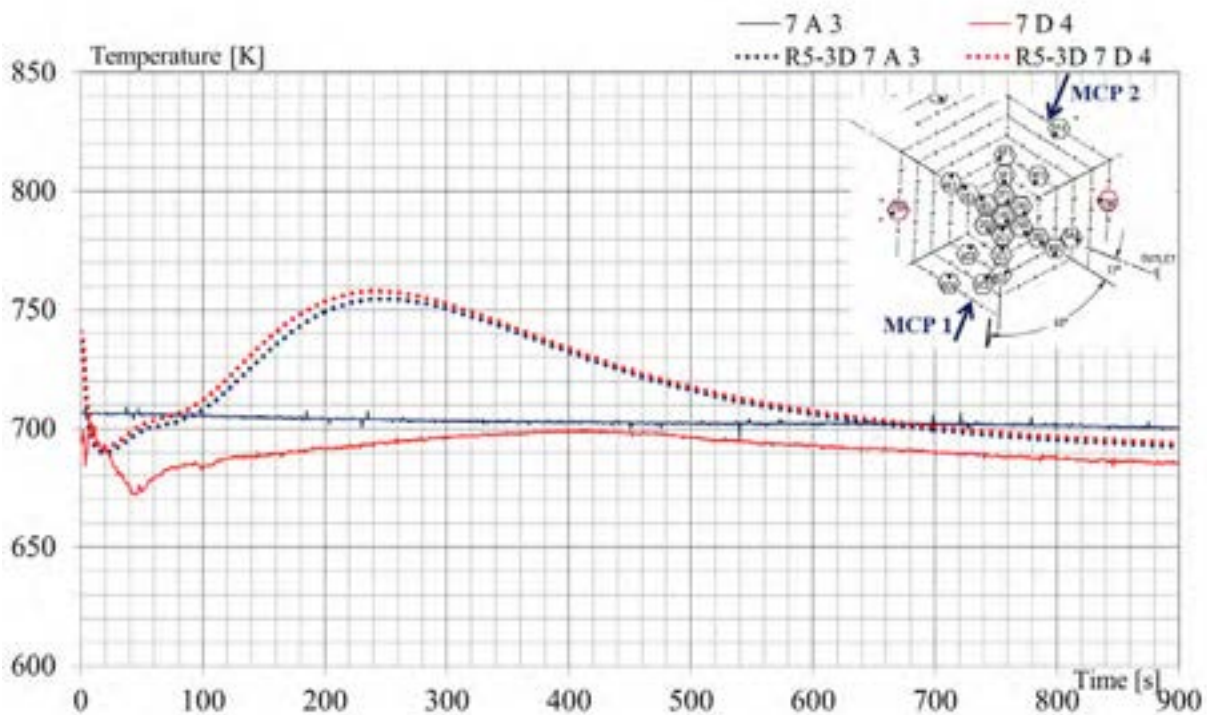
Fig. 37 – EBR-II SHRT-17, RELAP5-3D©: selected SA, ring 7 coolant outlet T.
