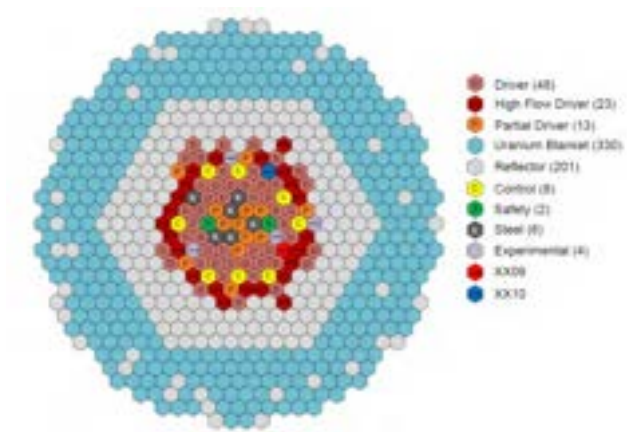
Fig. 59 – Core Neutronic Modelling.
