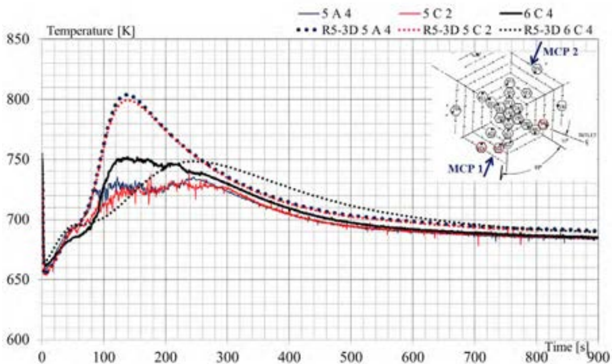
Fig. 36 – EBR-II SHRT-17, RELAP5-3D©: selected SA, ring 5 and 6 coolant outlet T.
