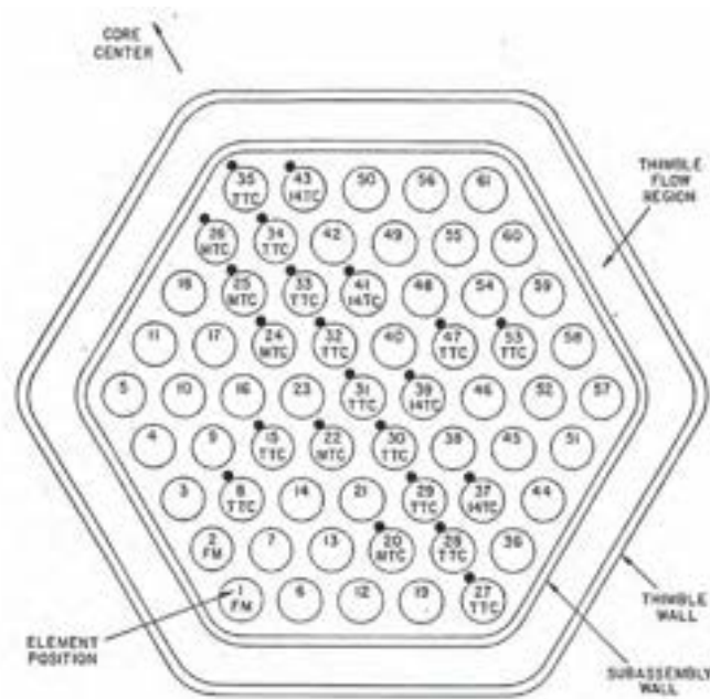
Fig. 51 – Thermocouples position in XX09 Fuel Assembly.
