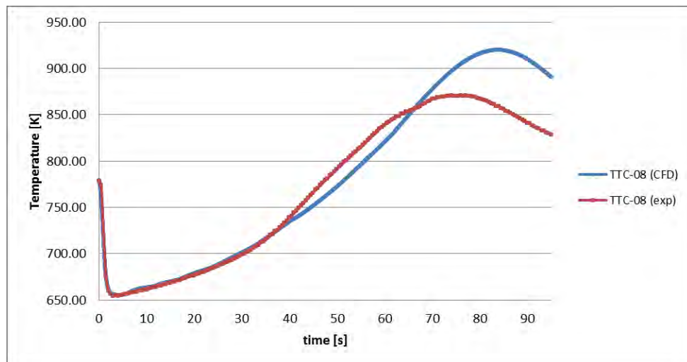
Fig. 55 – Comparison of CFD and experimental results for the top-core plane TTC TTC-08.
