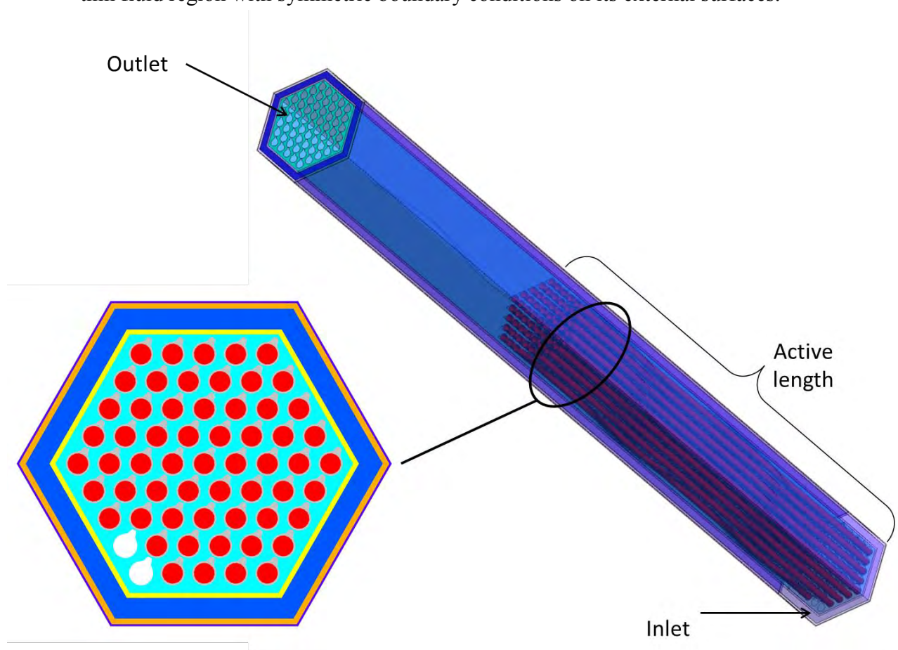
Fig. 49 – Layout of the CFD model.
