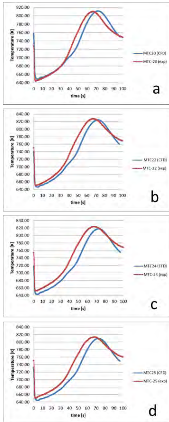
Fig. 54 – Comparison of CFD and experimental results for the mid-core plane MTC.
