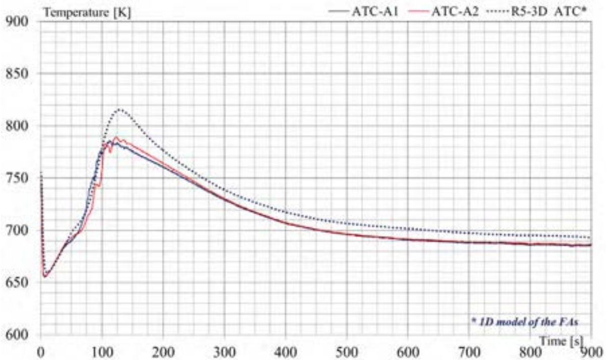
Fig. 26 – EBR-II SHRT-17, RELAP5-3D ® : FA XX09 coolant temperatures at outlet of thimble channel.
