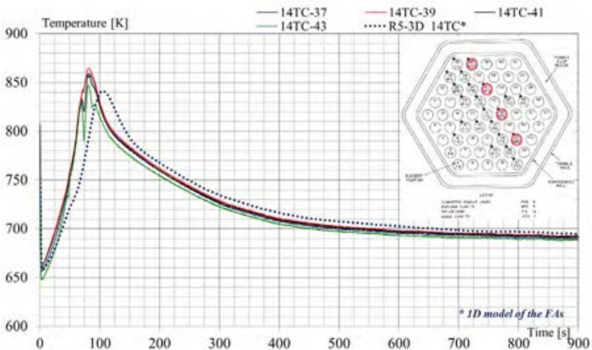
Fig. 24 – EBR-II SHRT-17, RELAP5-3D ® : FA XX09 cladding temperatures at top of wire wrapped fuel bundle.
