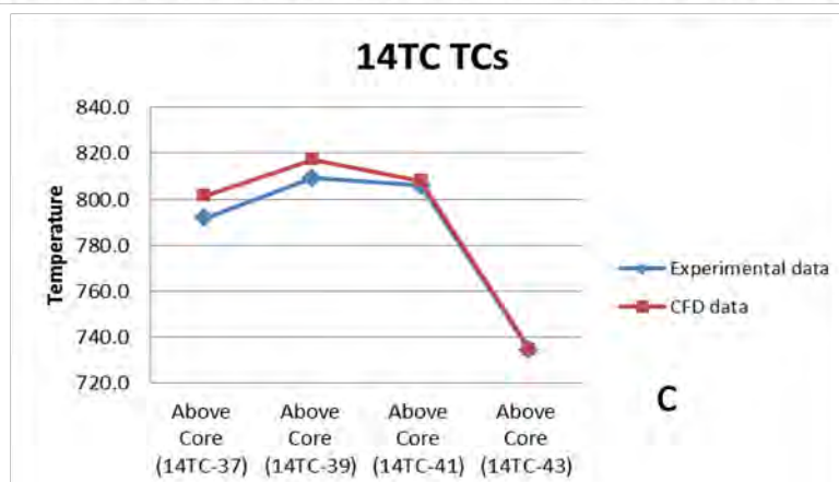
Fig. 53 – Comparison of the CFD results with SHRT-17 experimental values.
