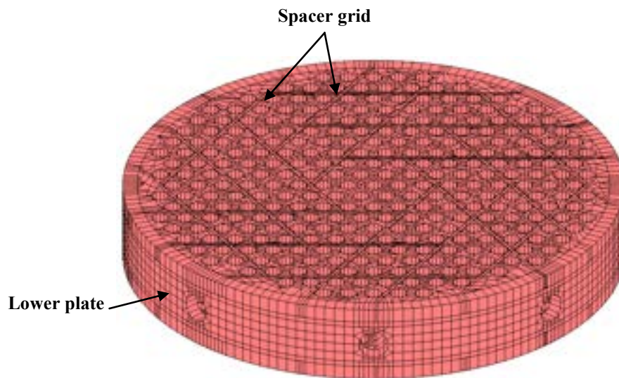
Figure 9 – Details of the lower grid model with plates and spacer grid.
