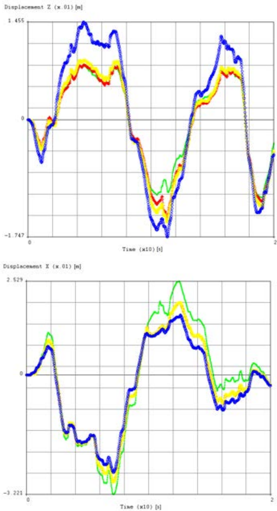
Figure 16 – FAs horizontal displacements.
