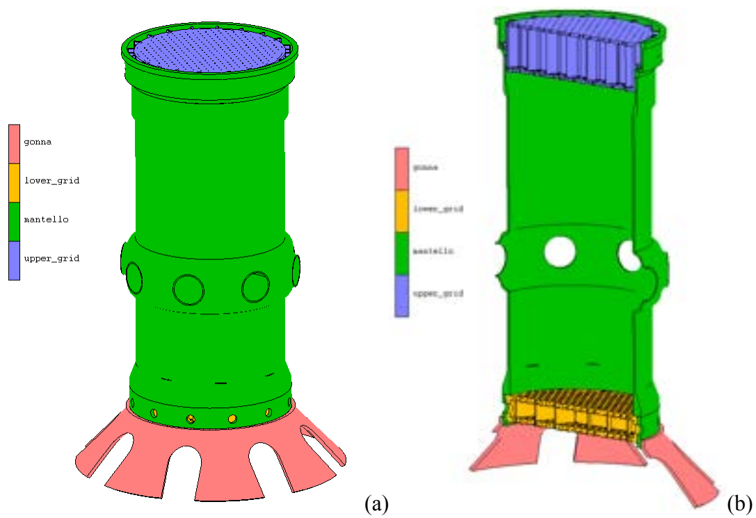
Figure 7 – FEM model of the inner cylindrical vessel: view (a) and vertical section (b).
