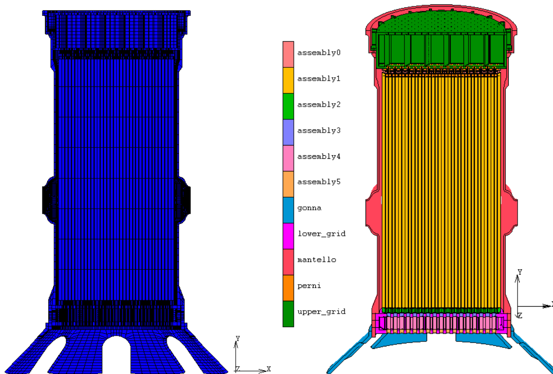
Figure 8 –Model of the inner cylindrical vessel with FAs
