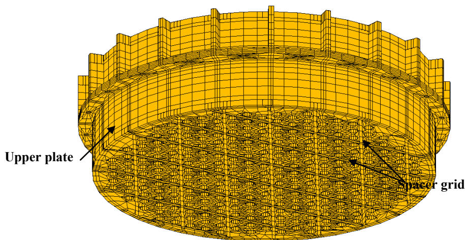
Figure 10 – Details of the upper grid model with plates and spacer grid.
