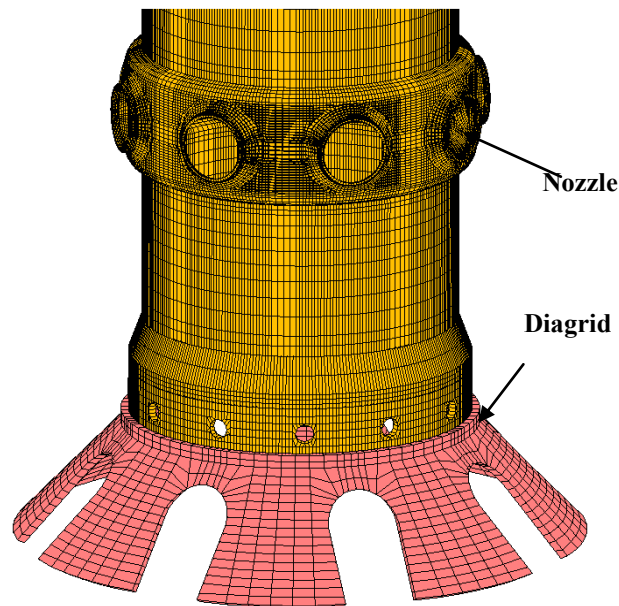
Figure 11 – Details of the bottom part of the inner vessel with lower late and diagrid.
