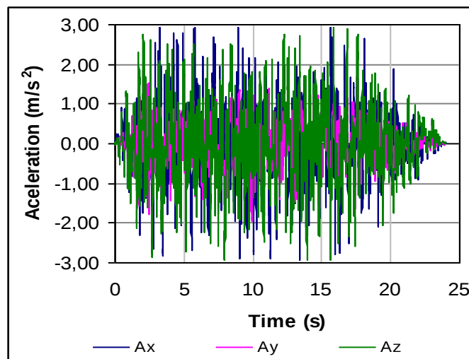
Figure 5 – 0.3 g PGA ATHs ground motion.
