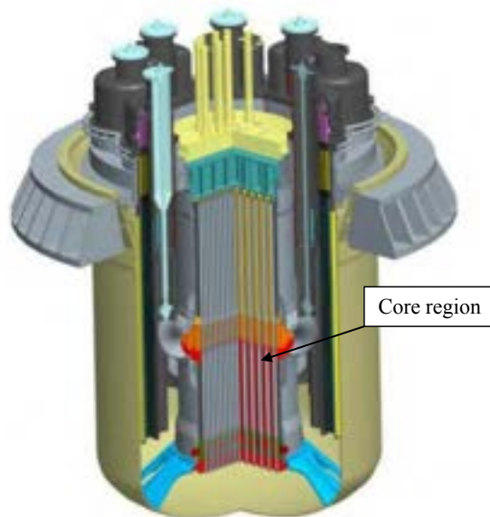
Figure 2 – Advanced Lead-cooled Fast Reactor European Demonstrator - ALFRED scheme [3].
