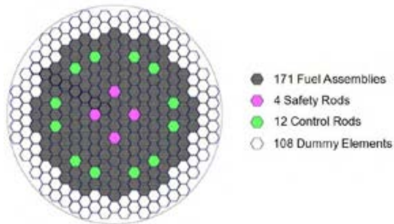
Figure 3 – ALFRED core configuration.
