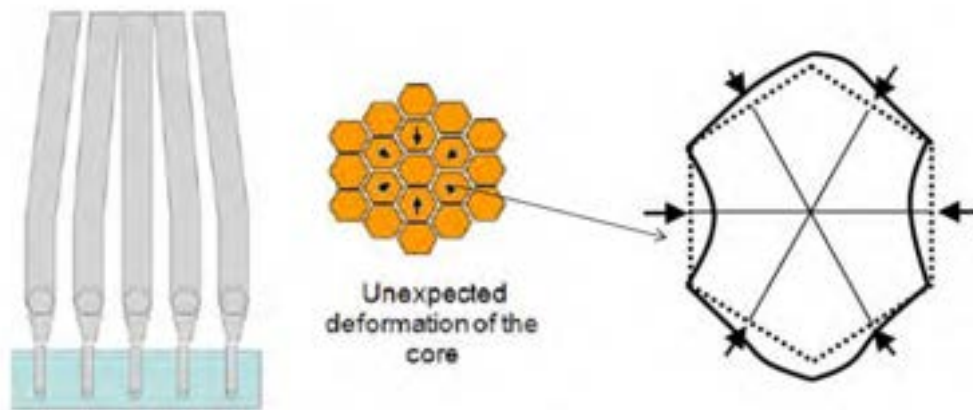
Figure 1 – Scheme of core compaction.
