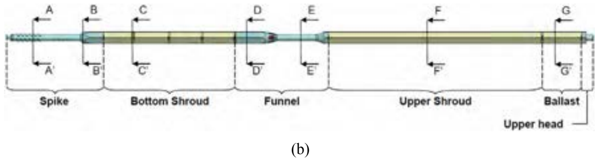
Figure 4 – Hexagonal FA geometry (the dimensions are in mm) (a), and an overview of the element parts (b) [12].
