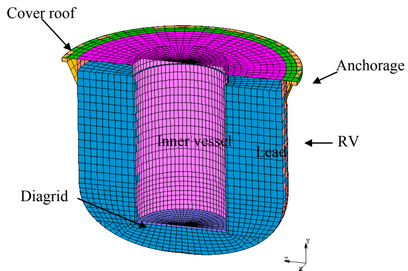
Figure 6 – FEM model of the RV.
