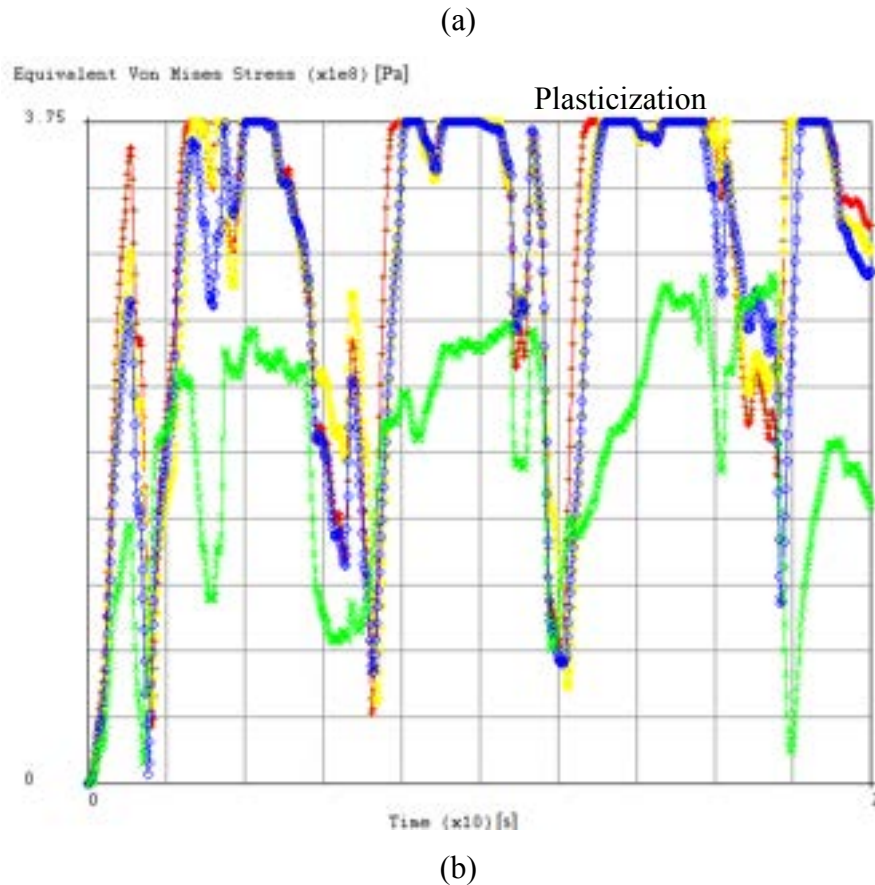
Figure 15 – FAs Von Mises stress vs. time.
