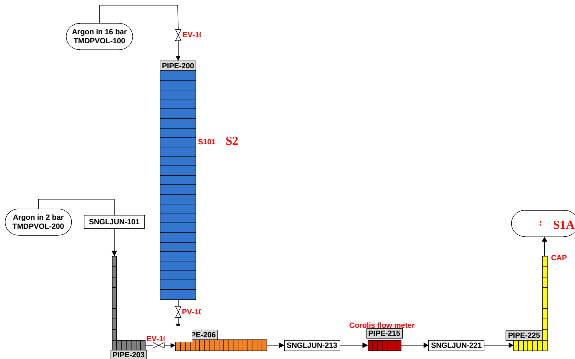
Fig. A. 1 – RELAP5/Mod3.3 nodalization of the injection line
