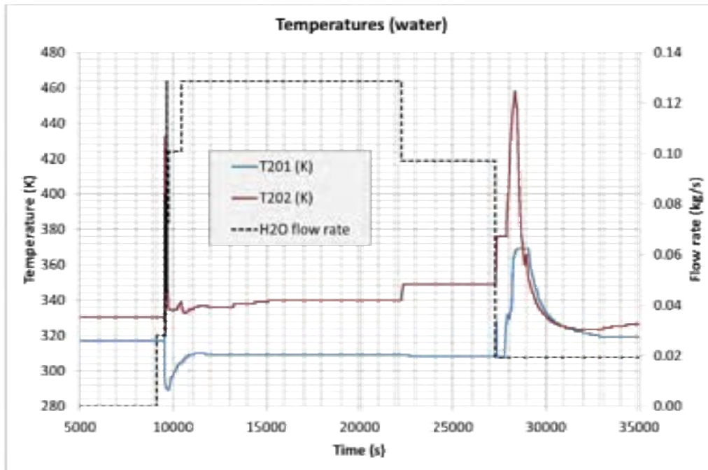
Figure 10: Test #301 – Water flow rate and temperatures
