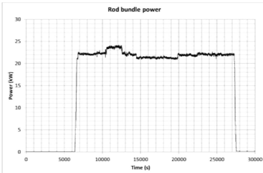
Figure 11: Test #303 – Fuel pin simulator power
