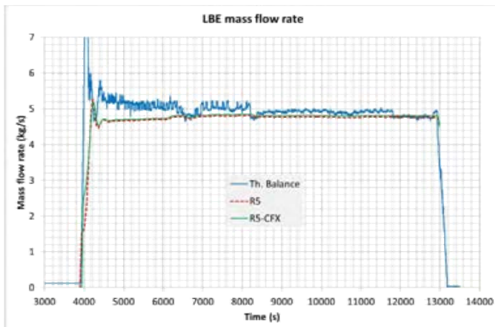
Figure 30: Test #201 Coupled Simulation Results – LBE flow rate
