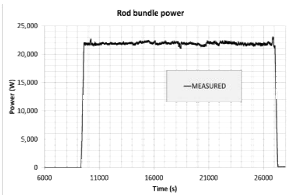
Figure 7: Test #301 – Fuel pin simulator power
