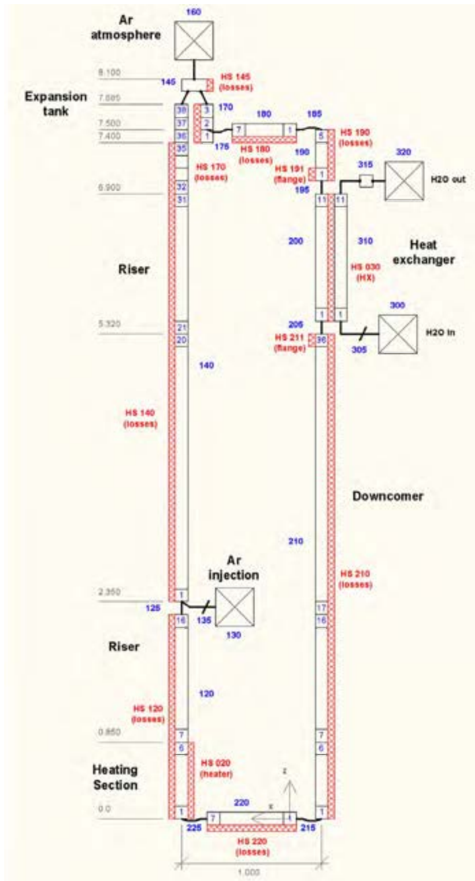
Figure 16: Sketch of RELAP5 nodalization
