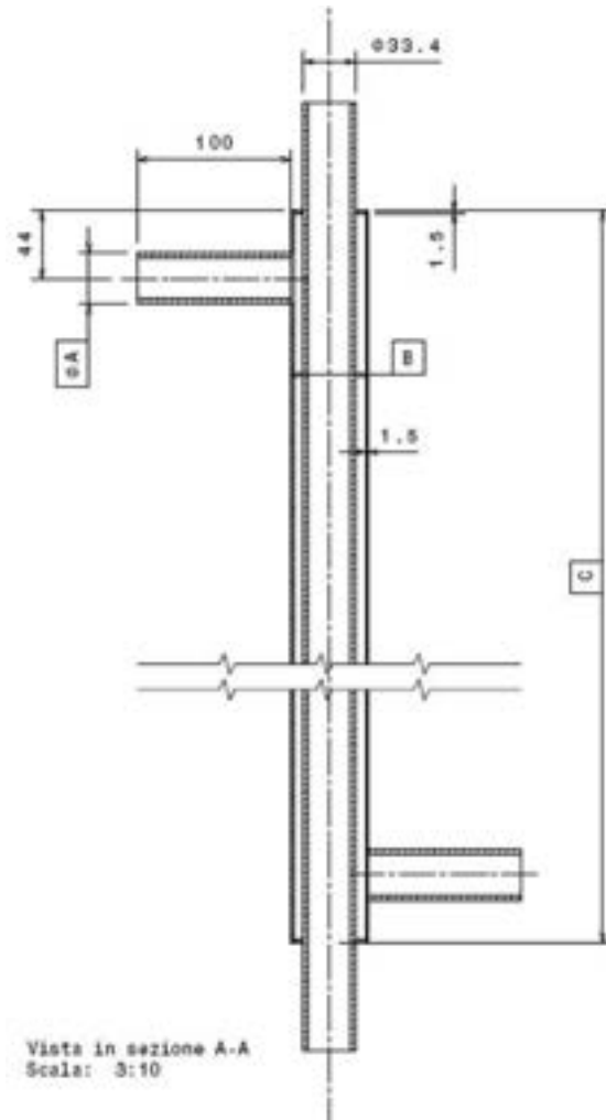
Figure 5 - design of the lithium/air heat exchanger
