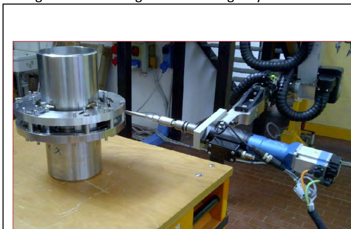
Closing operation of the FDS
