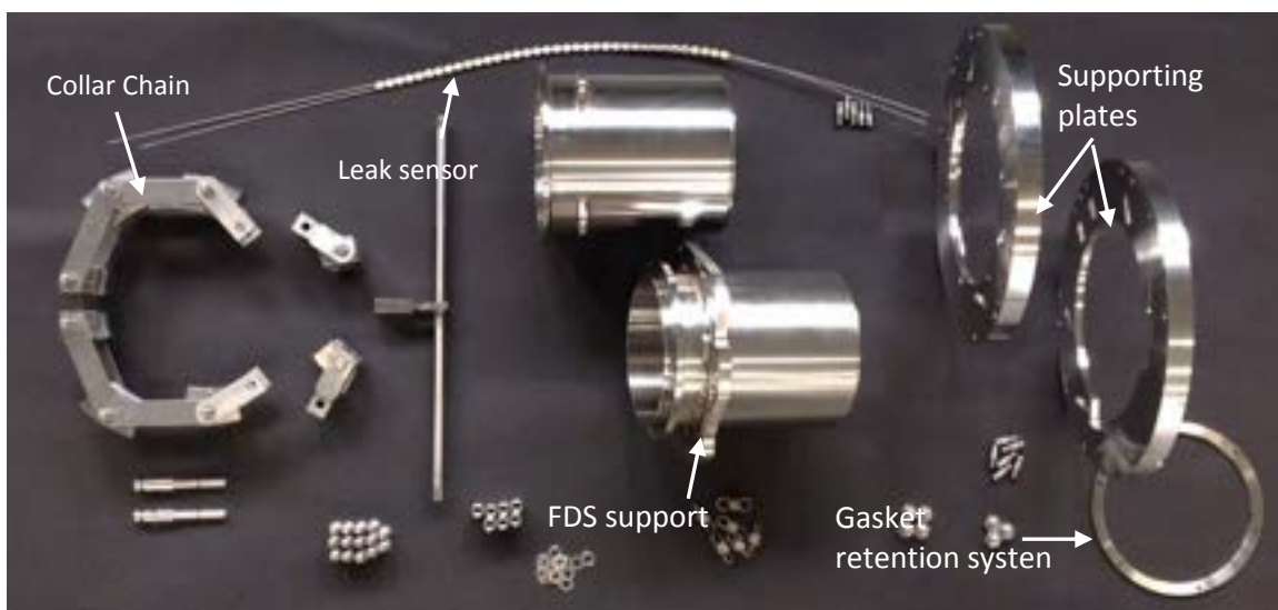
Fig. 3 FDS components
