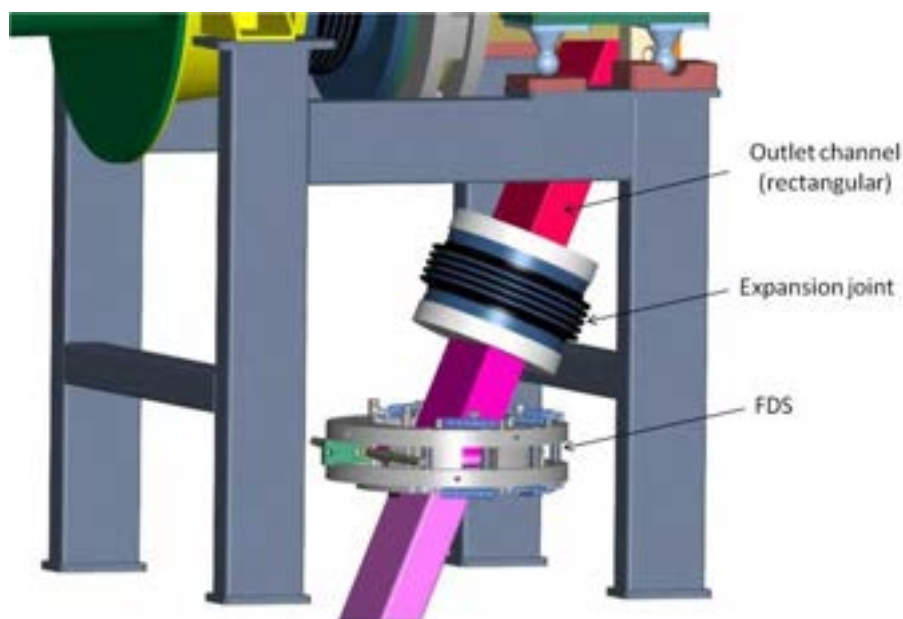
Fig. 2.9 – Outlet channel
