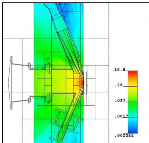
Fig.2.36 - Gamma heating ( \text{W}/\text{cm}^3 ) distribution on TA. Vertical cut at x=0 .
