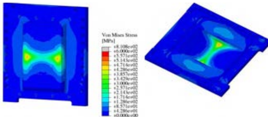
Fig. 2.47 - Von Mises equivalent stress field in the BP
