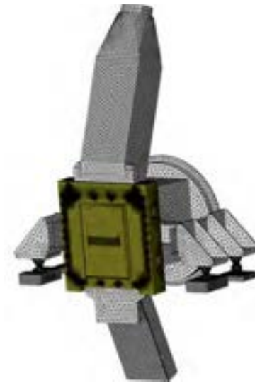
Fig. 2.40 - FE computational mesh
