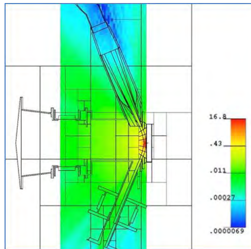
Fig.2.35 - Neutron heating ( \text{W}/\text{cm}^3 ) distribution on TA. Vertical cut at x=0 .
