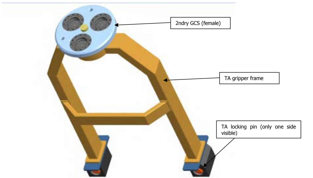
Fig. 2.25 - TA gripper overall view
