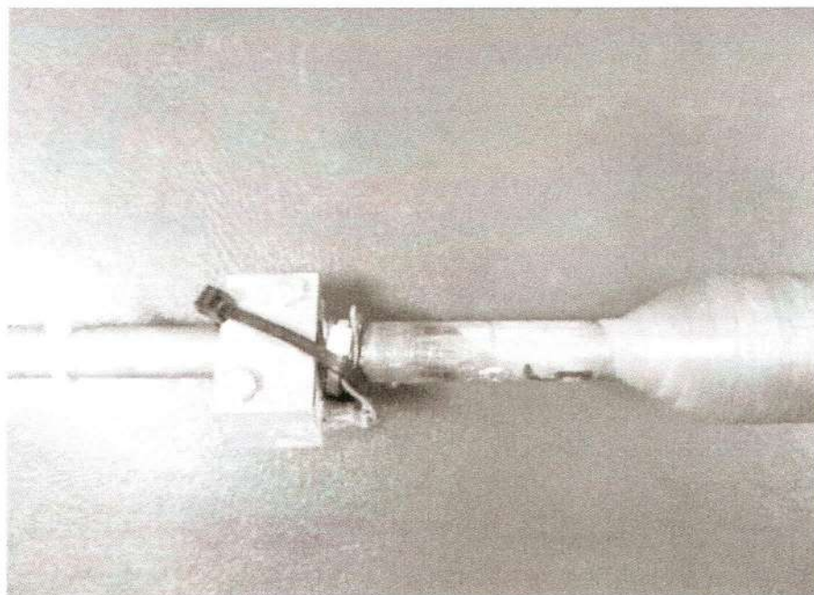
Fig. 4 – PT100 location
