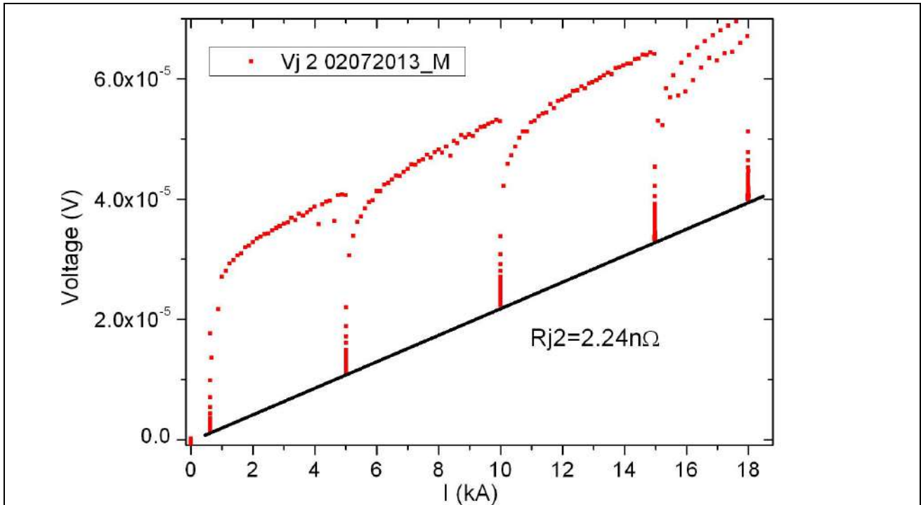
Figure 12: Measured voltage Vj2 across JT60SA joint versus current during run 02072013_M. The joint resistance value is obtained by the slope of the line that connects the points of minimum voltage for each current plateaux.
