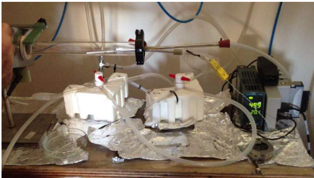
Fig. 8 Apparatus used to heat the strand samples up to 500 °C for 30 s.
