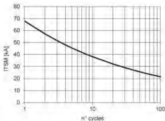
SURGE CHARACTERISTIC T J = 125 °C
