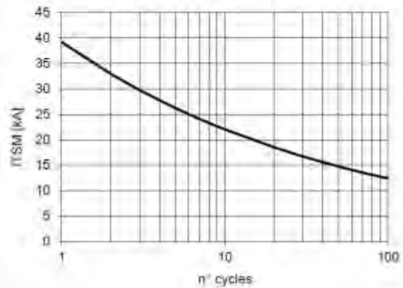
SURGE CHARACTERISTIC T_J = 125^\circ\text{C}
