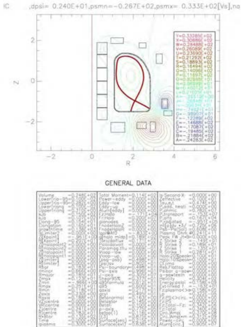
Figure 5. FAST-like Super-X: Super-X plasma shape and features.
