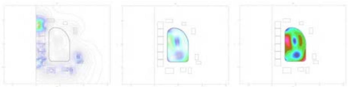
Figure 12. Poloidal magnetic field B due to PF coils and Super-X plasma in Super-X FAST.
