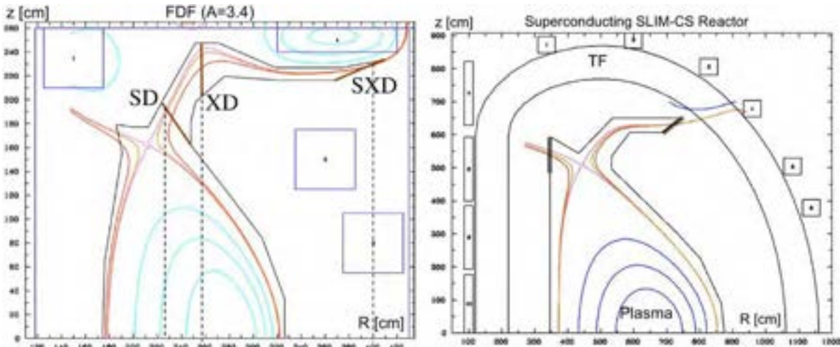
Figure 1. Left: SXD with PF coils inside TF; right: a SLIM-SXD reactor with PF coils outside TF
