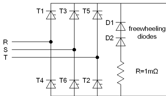
Figure 5 – Subunit electrical scheme
