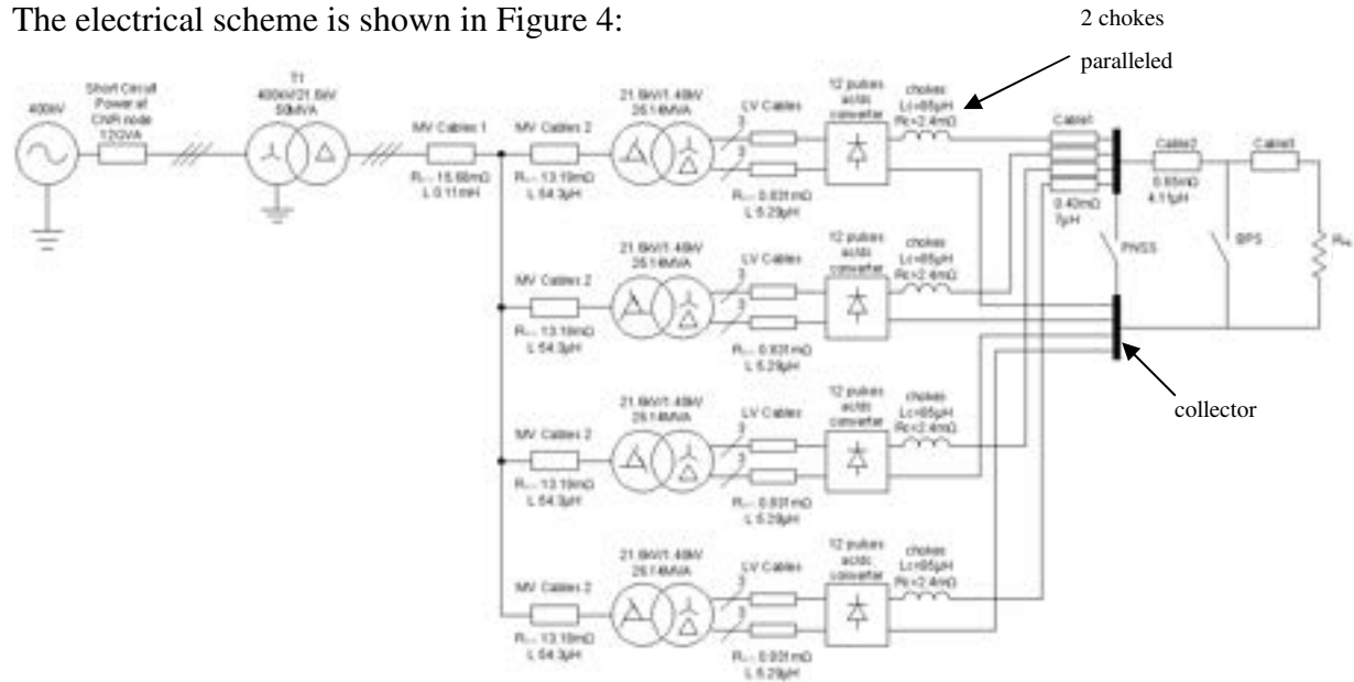
Figure 4 – Electrical scheme
