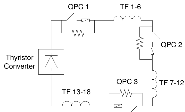
Figure 2.2 – Toroidal Circuit
