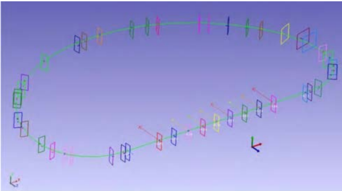
Fig. 3. DP centerline reconstructed form laser tracker measurements.
