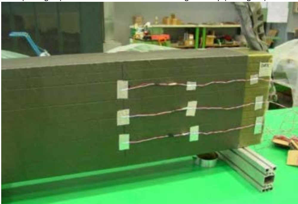
Fig. 19. Impregnation beam equipped with thermocouples before insertion in the curved leg mock-up.
