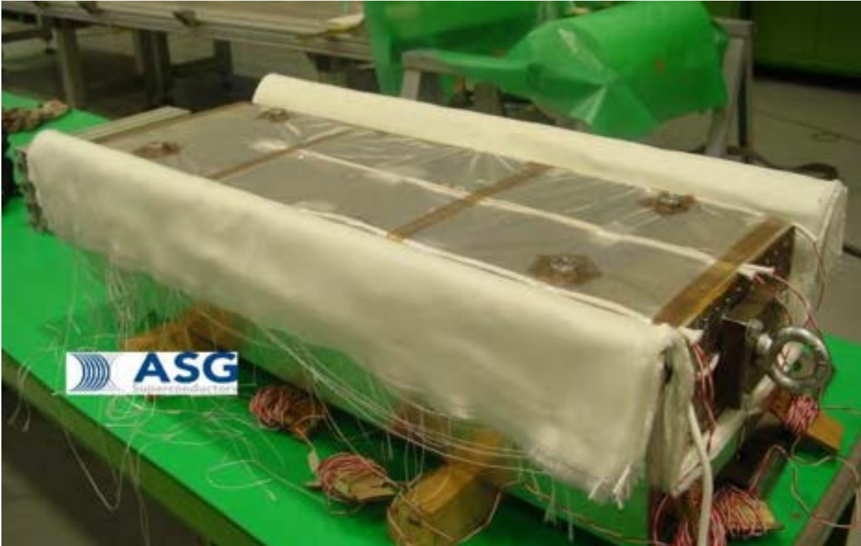
Fig. 22. WP mock-up inserted in straight leg mock-up.
