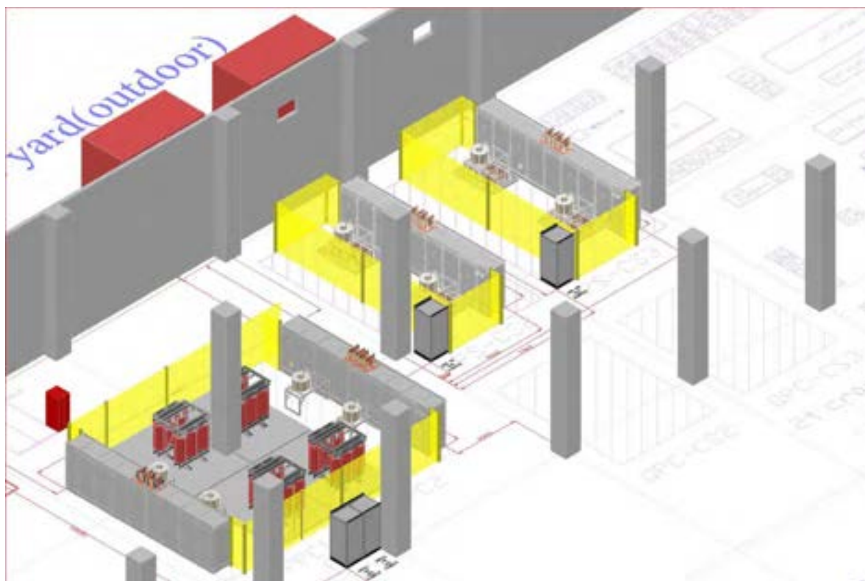
Figure 9 – Axonometric view
