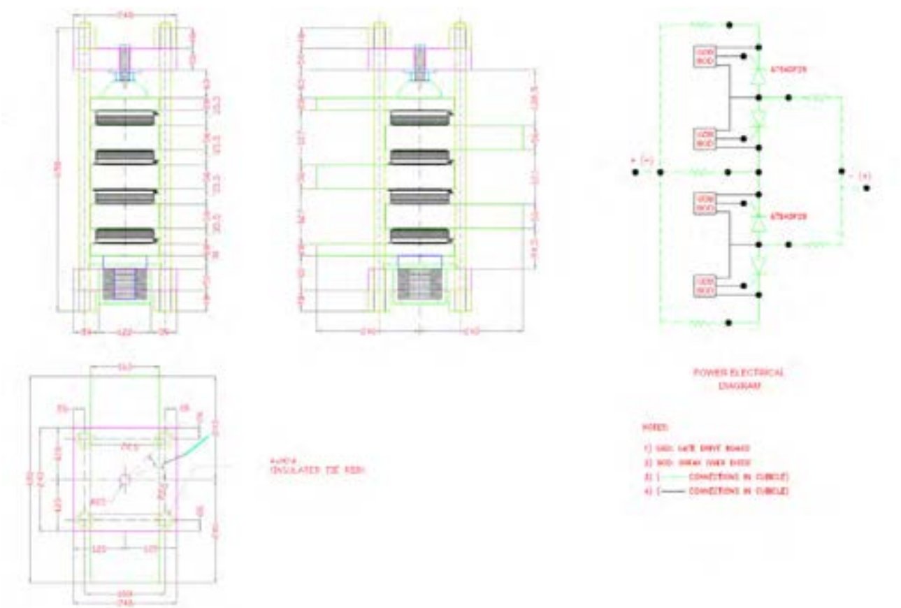
Figure 7 – Crowbar Power Assembly
