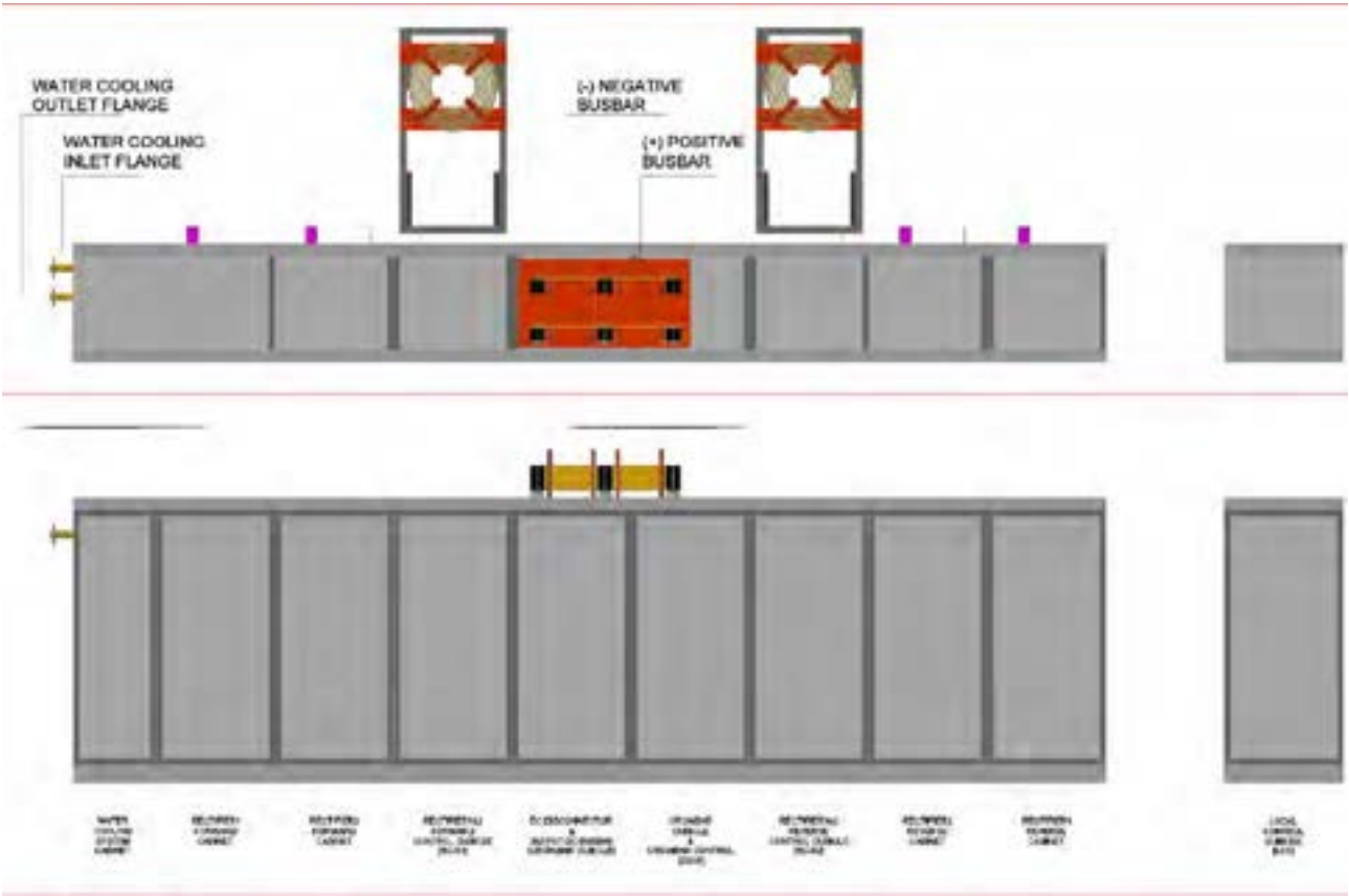
Figure 11 – FPPC PS Layout
