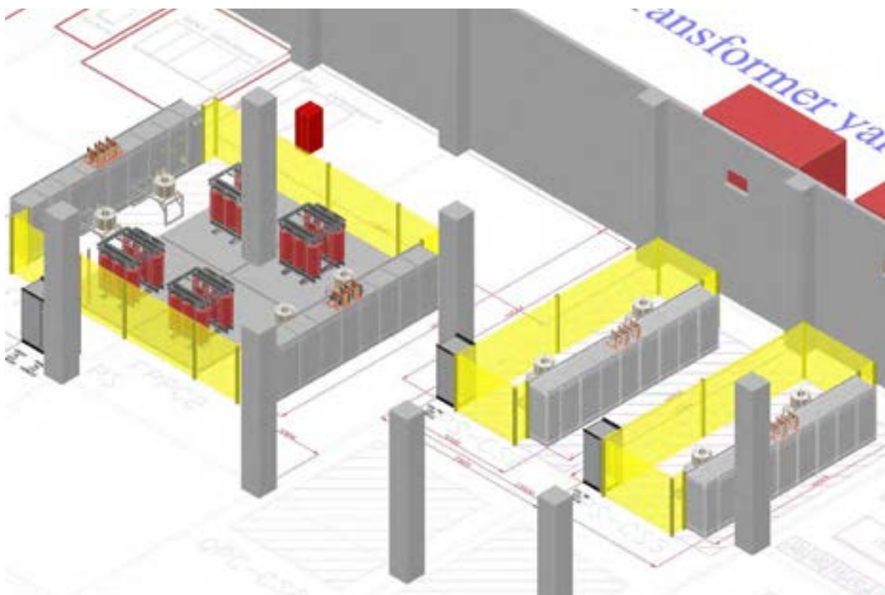
Figure 10 - Axonometric view
